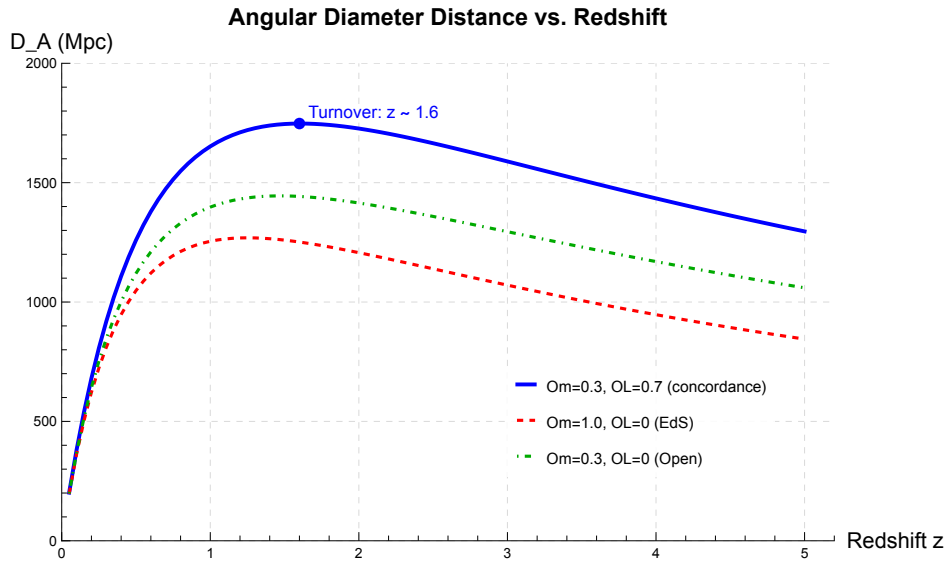
Figure 7.1: Angular diameter distance D_A(z) for the concordance cosmology ( \Omega_m = 0.3 , \Omega_\Lambda = 0.7 , H_0 = 70 \text{ km s}^{-1} \text{ Mpc}^{-1} ). D_A reaches a maximum of approximately 1748 Mpc at z \approx 1.6 and then decreases. This turnover is a key consequence of the expanding universe and has no analogue in Euclidean geometry. Generated by friedmann_equations.wl .
