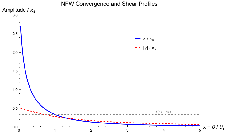
Figure 11.2: NFW convergence \kappa(x)/\kappa_s = f(x) (solid) and shear |\gamma(x)|/\kappa_s = \bar{\kappa}(x)/\kappa_s - f(x) (dashed) as functions of the dimensionless radius x = \theta/\theta_s . Both curves are normalized to \kappa_s and are universal functions of x (independent of concentration); the horizontal grey line marks f(1) = 1/3 . The concentration c enters only through the overall scale \kappa_s and the angular scale \theta_s , both of which absorb the dependence on c and on the cosmological distances. Generated by axisymmetric_models.wl .
