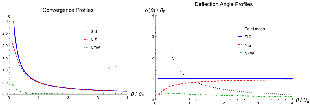
Figure 11.3: Comparison of convergence profiles (left) and deflection angles (right) for the four axisymmetric models. All curves use the SIS Einstein radius \theta_E as the unit of length on the horizontal axis; the SIS, NIS and NFW amplitudes are set so that the profiles can be compared on the same panel (specifically NIS with \theta_c = 0.2 \theta_E and NFW with \theta_s = 0.3 \theta_E , \kappa_s = 0.5 ). Only the SIS and NIS are normalized to reproduce \bar{\kappa}(\theta_E) = 1 ; the NFW deflection therefore does not pass through \alpha = \theta_E at \theta = \theta_E on this plot. The point mass convergence is a delta function and is not shown. Generated by axisymmetric_models.wl .
