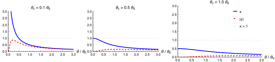
Figure 11.1: Effect of the core radius on the NIS convergence and shear, shown for three regimes that control the critical-curve topology. Left: for \theta_c = 0.1 \theta_E < \theta_E/2 , the central convergence \kappa(0) > 1 , so both tangential and radial critical curves exist and three images can form. Center: at the critical value \theta_c = 0.5 \theta_E = \theta_E/2 , \kappa(0) = 1 exactly and the radial critical curve collapses to a point. Right: for \theta_c = 1.0 \theta_E > \theta_E/2 , \kappa(0) < 1 everywhere; no critical curves exist and only one image forms. Generated by axisymmetric_models.wl .
