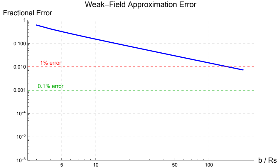
Figure 5.3: Fractional error |\hat{\alpha}_{\text{exact}} - \hat{\alpha}_{\text{weak}}|/\hat{\alpha}_{\text{exact}} of the weak-field approximation as a function of b/R_S . The error is \approx (15\pi/32) R_S/b : below 1% for b/R_S \gtrsim 150 and below 0.1% for b/R_S \gtrsim 1500 . For typical astrophysical lenses ( b/R_S > 10^4 ), the weak-field approximation is essentially exact.
