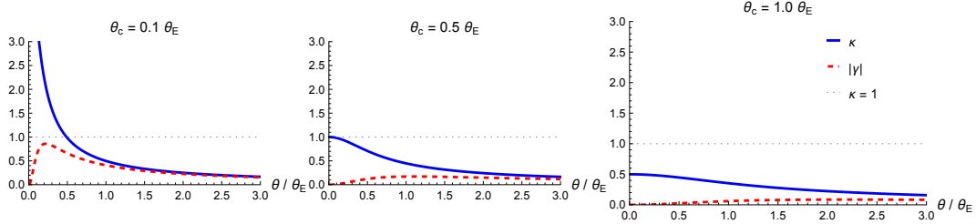
Figure 11.1: Effect of the core radius on the NIS convergence and shear, shown for three regimes that control the critical-curve topology. Left: for \theta_c = 0.1 \theta_E < \theta_E/2 , the central convergence \kappa(0) > 1 , so both tangential and radial critical curves exist and three images can form. Center: at the critical value \theta_c = 0.5 \theta_E = \theta_E/2 , \kappa(0) = 1 exactly and the radial critical curve collapses to a point. Right: for \theta_c = 1.0 \theta_E > \theta_E/2 , \kappa(0) < 1 everywhere; no critical curves exist and only one image forms. Generated by axisymmetric_models.wl .
