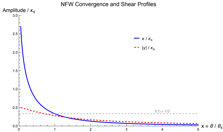
Figure 11.2: NFW convergence \kappa(x)/\kappa_s = f(x) (solid) and shear |\gamma(x)|/\kappa_s = \bar{\kappa}(x)/\kappa_s - f(x) (dashed) as functions of the dimensionless radius x = \theta/\theta_s . Both curves are normalized to \kappa_s and are universal functions of x (independent of concentration); the horizontal grey line marks f(1) = 1/3 . The concentration c enters only through the overall scale \kappa_s and the angular scale \theta_s , both of which absorb the dependence on c and on the cosmological distances. Generated by axisymmetric_models.wl .
