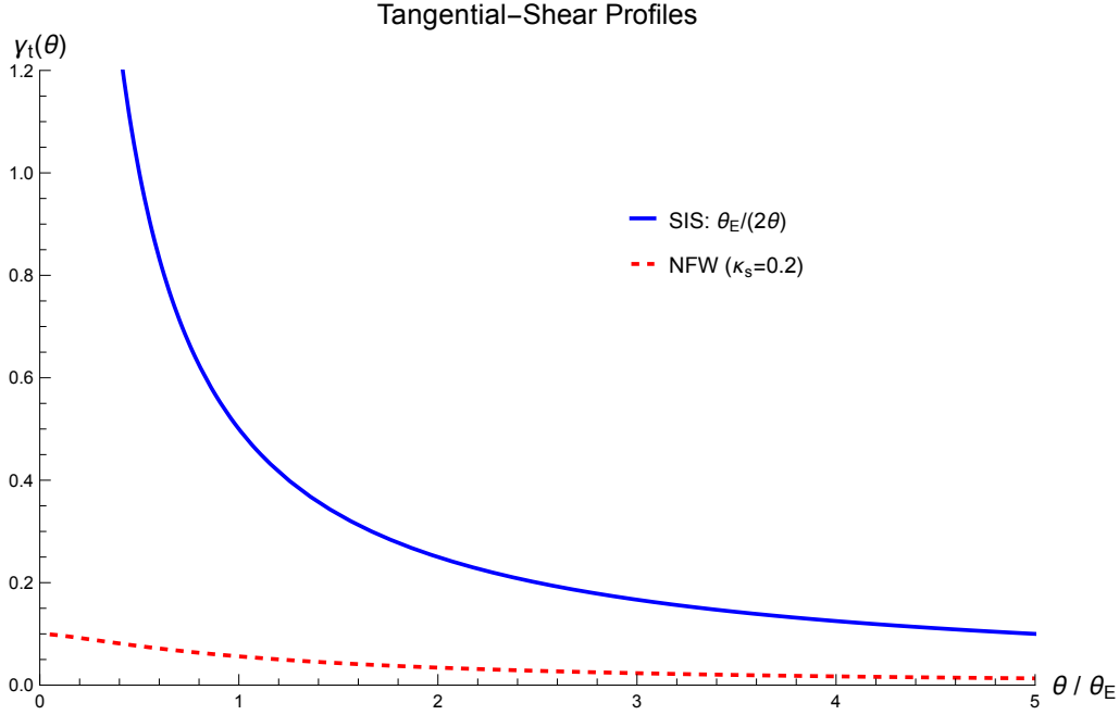
Figure 16.1: Tangential-shear profiles \gamma_t(\theta) for two axisymmetric lenses, illustrating eq. (16.10). Solid: the singular isothermal sphere, \gamma_t = \theta_E/(2\theta) (eq. 16.12), with \theta_E = 1 . Dashed: an NFW halo (Module 11, eq. 11.53) with \kappa_s = 0.2 and scale \theta_s = 1 . The NFW tangential shear decreases monotonically: it tends to the finite value \kappa_s/2 at the centre, is nearly flat inside \theta_s , and steepens outside it, whereas the SIS is a single power law. The measurable \gamma_t maps directly to the excess surface mass density \Delta\Sigma (eq. 16.11). Generated by weak_lensing.wl .
