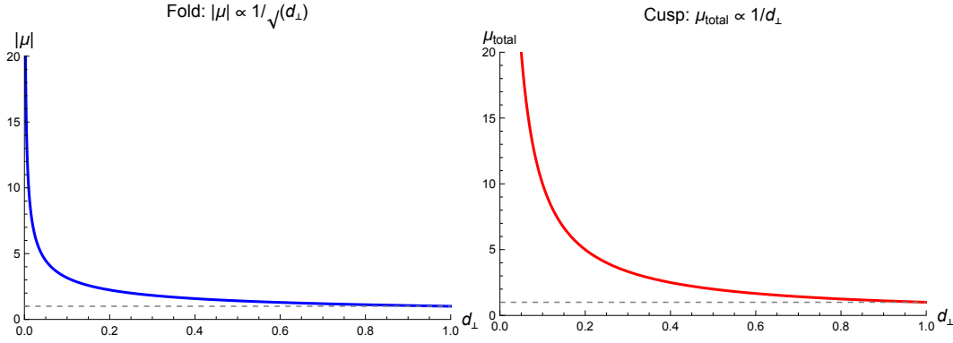
Figure 12.4: Magnification behavior near fold and cusp caustics. Left: Near a fold, two images straddle the critical curve with magnifications scaling as |\mu| \propto 1/\sqrt{d_{\perp}} . Right: Near a cusp, three images merge, with stronger divergence. The cusp relation \mu_A + \mu_B + \mu_C \approx 0 holds for the signed magnifications. Generated by critical_curves_caustics.wl .
