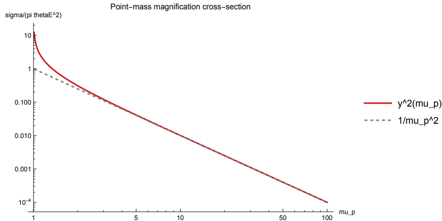
Figure 15.1: The point-mass magnification cross-section \sigma(\mu_p)/(\pi\theta_E^2) = y^2(\mu_p) of Eq. (15.1), as a function of the magnification threshold \mu_p . At high magnification the cross-section falls as \sigma \propto \mu_p^{-2} (dashed), the universal scaling that produces p(\mu) \propto \mu^{-3} and drives the magnification bias. Generated by lensing_statistics.wl .
