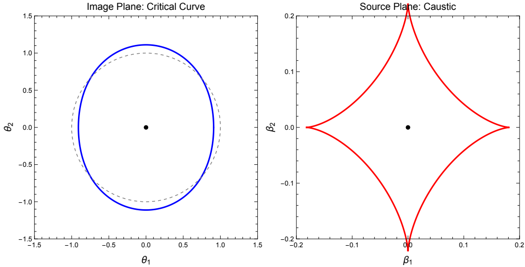
Figure 12.1: Critical curves (left, image plane) and caustics (right, source plane) for the SIS + external shear model with \theta_E = 1'' and \gamma_{\text{ext}} = 0.1 . The critical curve is an oval (approximately elliptical for small shear); the caustic is a diamond (astroid) with four cusps. The shear axis is horizontal. Generated by critical_curves_caustics.wl .
