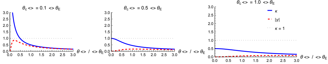
Figure 11.1: Effect of the core radius on the NIS convergence and shear, shown for three regimes that control the critical-curve topology. Left: for \theta_c = 0.1 \theta_E < \theta_E/2 , the central convergence \kappa(0) > 1 , so both tangential and radial critical curves exist and three images can form. Center: at the critical value \theta_c = 0.5 \theta_E = \theta_E/2 , \kappa(0) = 1 exactly and the radial critical curve collapses to a point. Right: for \theta_c = 1.0 \theta_E > \theta_E/2 , \kappa(0) < 1 everywhere; no critical curves exist and only one image forms. Generated by axisymmetric_models.wl .
