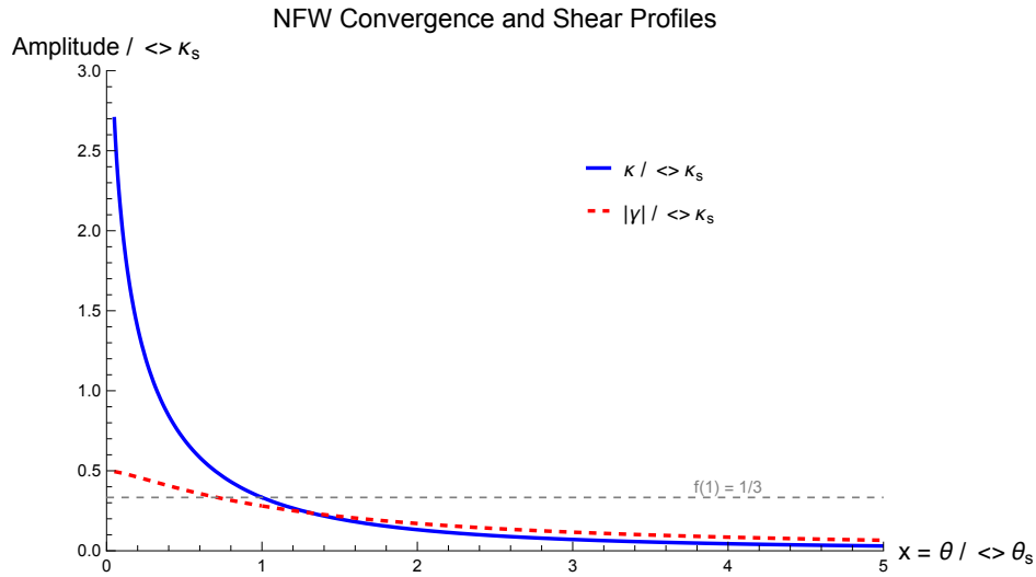
Figure 11.2: NFW convergence \kappa(x)/\kappa_s = f(x) (solid) and shear |\gamma(x)|/\kappa_s = \bar{\kappa}(x)/\kappa_s - f(x) (dashed) as functions of the dimensionless radius x = \theta/\theta_s . Both curves are normalized to \kappa_s and are universal functions of x (independent of concentration); the horizontal grey line marks f(1) = 1/3 . The concentration c enters only through the overall scale \kappa_s and the angular scale \theta_s , both of which absorb the dependence on c and on the cosmological distances. Generated by axisymmetric_models.wl .
