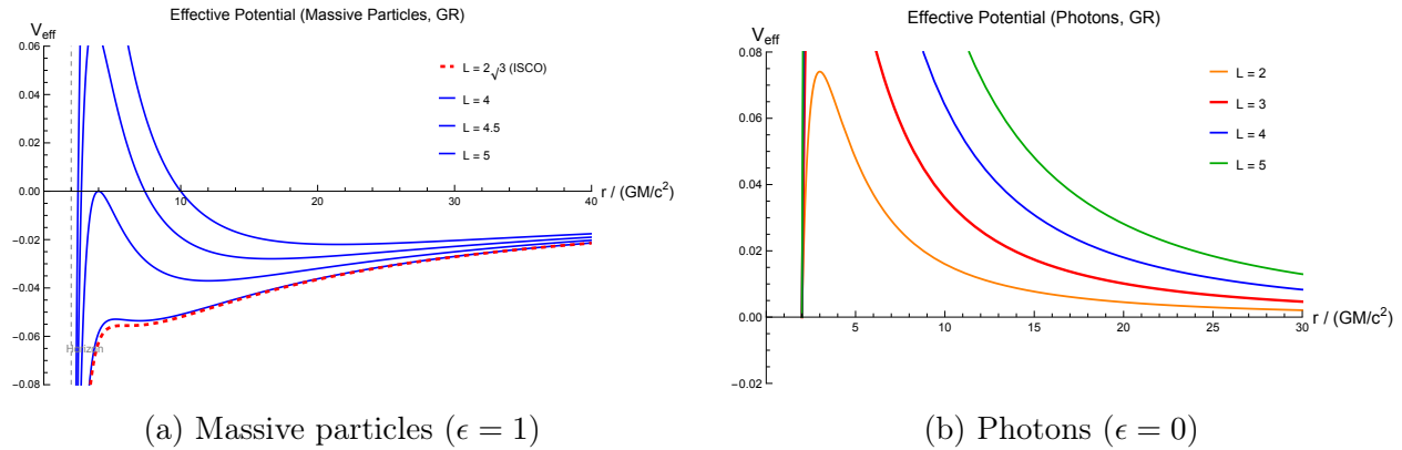
Figure 4.2: GR effective potentials for several values of angular momentum L (in GM/c units). Left: For massive particles, the red dashed curve shows L = L_{\text{ISCO}} = 2\sqrt{3} GM/c , where the stable and unstable circular orbits merge. Right: For photons, the potential always has a maximum at r = 3GM/c^2 (the photon sphere). Interactive versions in effective_potential.nb .
