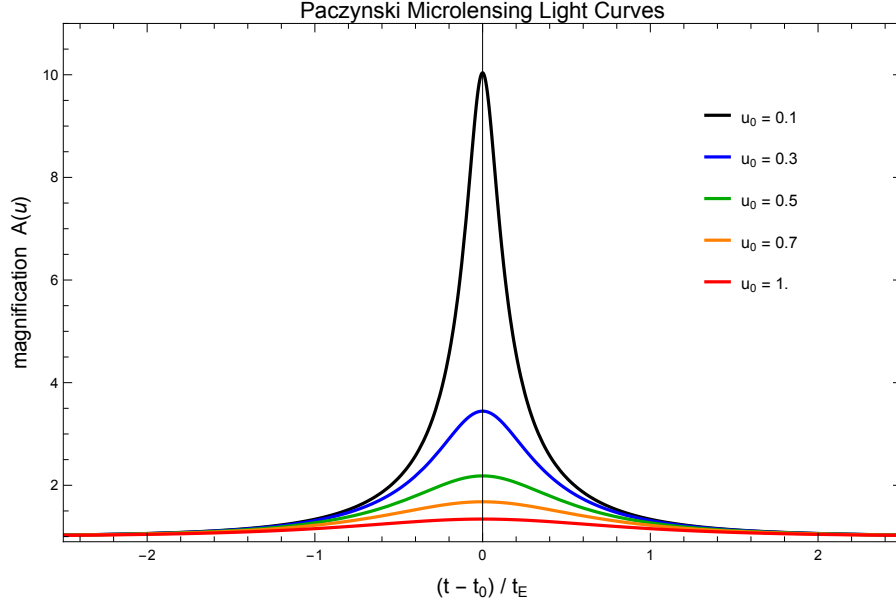
Figure 17.2: Paczyński microlensing light curves (eq. 17.8 substituted into eq. 17.5) for minimum impact parameters u_0 = 0.1, 0.3, 0.5, 0.7, 1.0 (top to bottom). Time is in units of the Einstein timescale t_E ; every curve is symmetric about the peak at (t - t_0)/t_E = 0 , and the smaller the impact parameter the higher and narrower the peak ( A_{\max} \approx 1/u_0 ). Generated by microlensing.wl .
