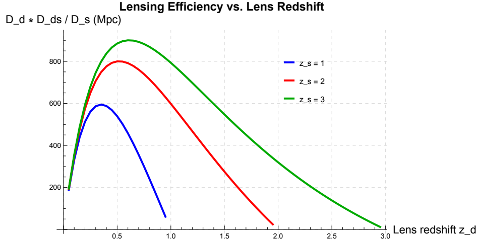
Figure 7.3: Lensing efficiency D_d D_{ds}/D_s as a function of lens redshift z_d for several source redshifts z_s = 1, 2, 3 in the concordance cosmology. For z_s = 1 , lensing is most efficient at z_d \approx 0.35 ; for z_s = 2 , at z_d \approx 0.5 . The lens is typically most effective when placed roughly “halfway” (in comoving distance) between the observer and the source. Generated by friedmann_equations.wl .
