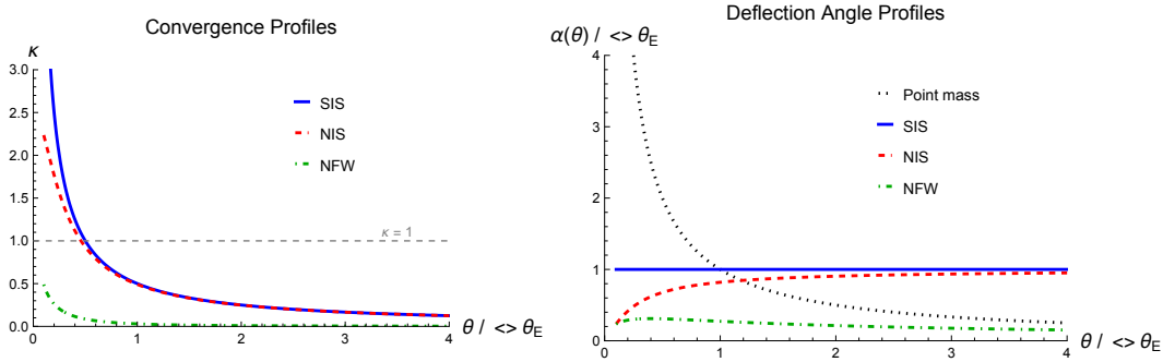
Figure 11.3: Comparison of convergence profiles (left) and deflection angles (right) for the four axisymmetric models. All curves use the SIS Einstein radius \theta_E as the unit of length on the horizontal axis; the SIS, NIS and NFW amplitudes are set so that the profiles can be compared on the same panel (specifically NIS with \theta_c = 0.2 \theta_E and NFW with \theta_s = 0.3 \theta_E , \kappa_s = 0.5 ). Only the SIS and NIS are normalized to reproduce \bar{\kappa}(\theta_E) = 1 ; the NFW deflection therefore does not pass through \alpha = \theta_E at \theta = \theta_E on this plot. The point mass convergence is a delta function and is not shown. Generated by axisymmetric_models.wl .
