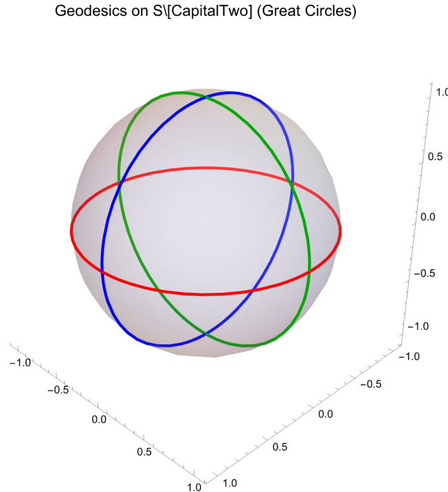
Figure 2.2: Geodesics on the 2-sphere are great circles. Three orthogonal great circles are shown, illustrating that the shortest path between any two points on a sphere follows a great circle arc.
