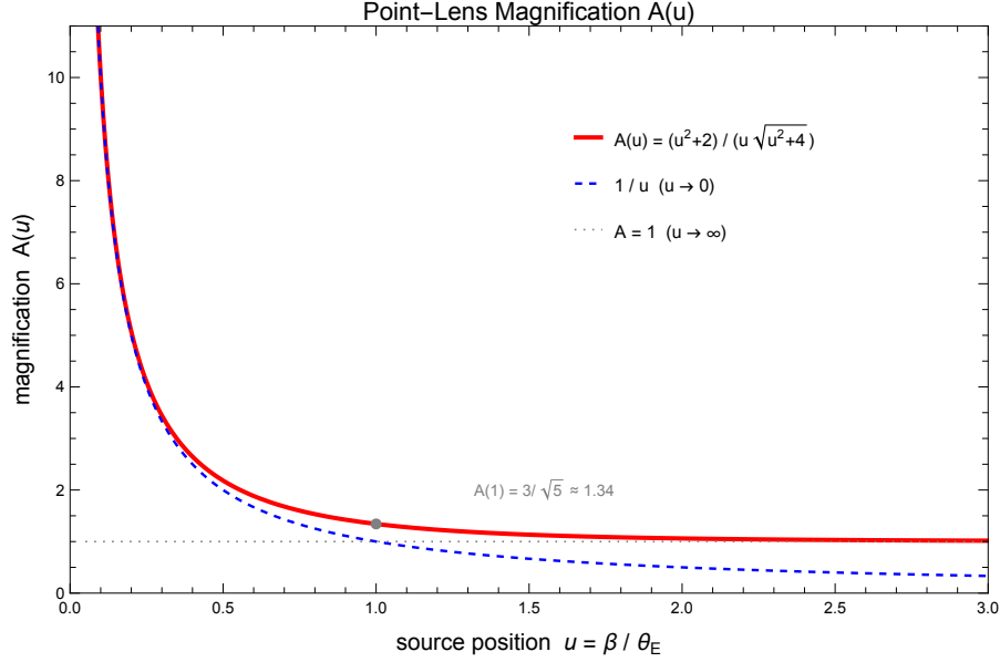
Figure 17.1: The point-lens total magnification A(u) (eq. 17.5, red) as a function of the source–lens separation u = \beta/\theta_E . The high-magnification asymptote A \rightarrow 1/u (blue dashed) and the unlensed limit A \rightarrow 1 (grey dotted) are shown for reference; the marked point is A(1) = 3/\sqrt{5} \approx 1.34 . Generated by microlensing.wl .
