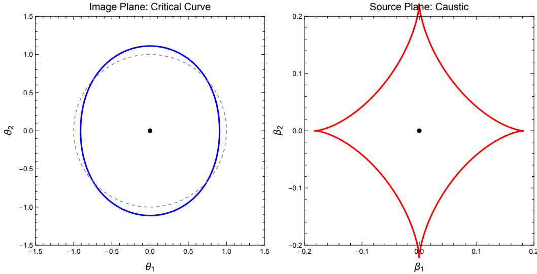
Figure 12.1: Critical curves (left, image plane) and caustics (right, source plane) for the SIS + external shear model with \theta_E = 1'' and \gamma_{\text{ext}} = 0.1 . The critical curve is an oval (approximately elliptical for small shear); the caustic is a diamond (astroid) with four cusps. The shear axis is horizontal. Generated by critical_curves_caustics.wl .
