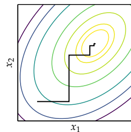
Figure 7.1. Cyclic coordinate descent alternates between coordinate directions.
