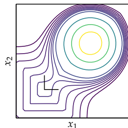
Figure 7.2. Above is an example of how cyclic coordinate search can get stuck. Moving in either of the coordinate directions will result only in increasing f , but moving diagonally, which is not allowed in cyclic coordinate search, can result in lowering f .
