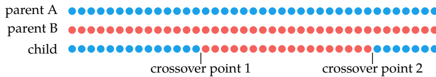
Figure 9.6. Two-point crossover.
