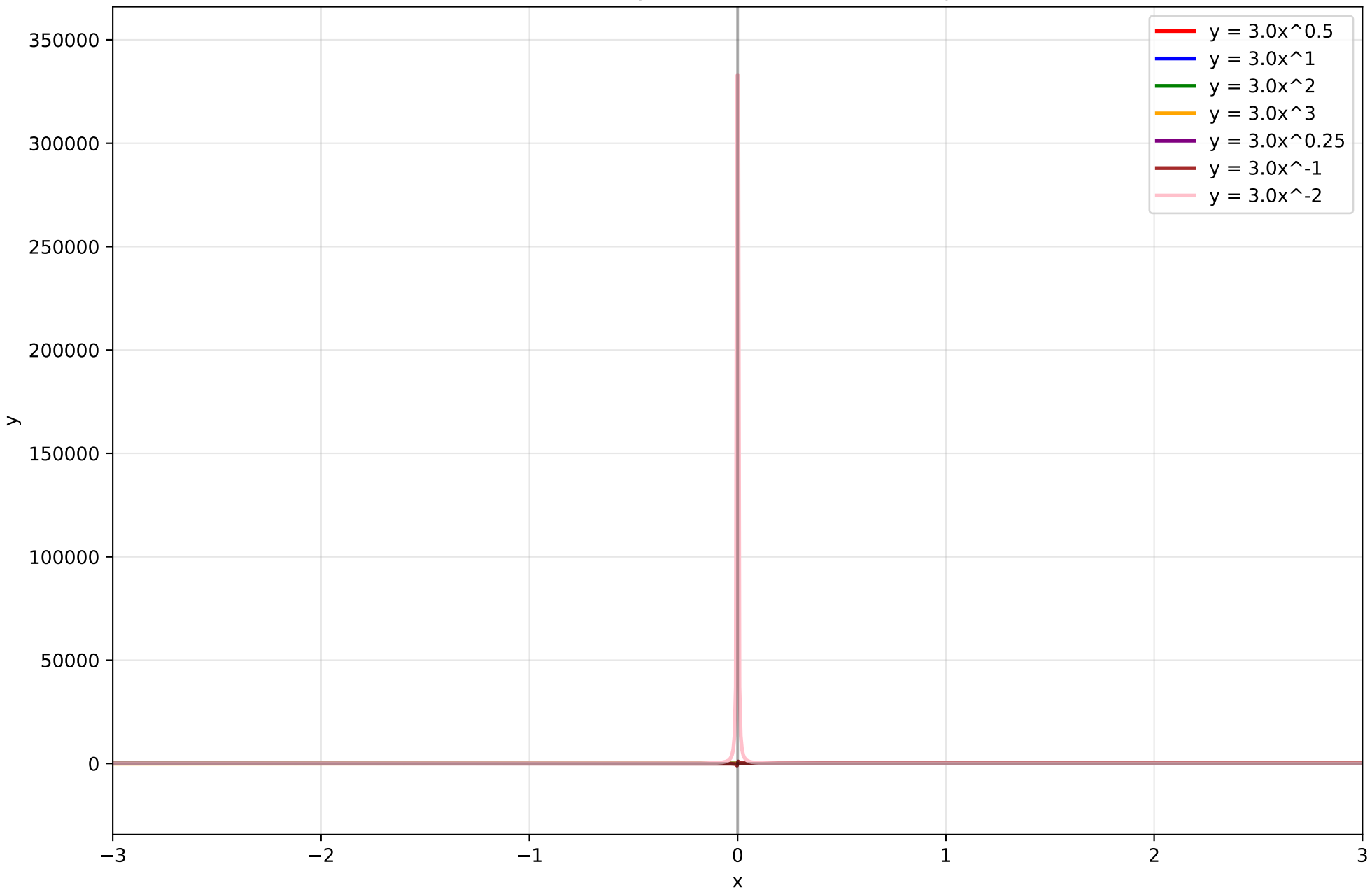
Power Functions: y = 3.0x^n for Different Exponents
