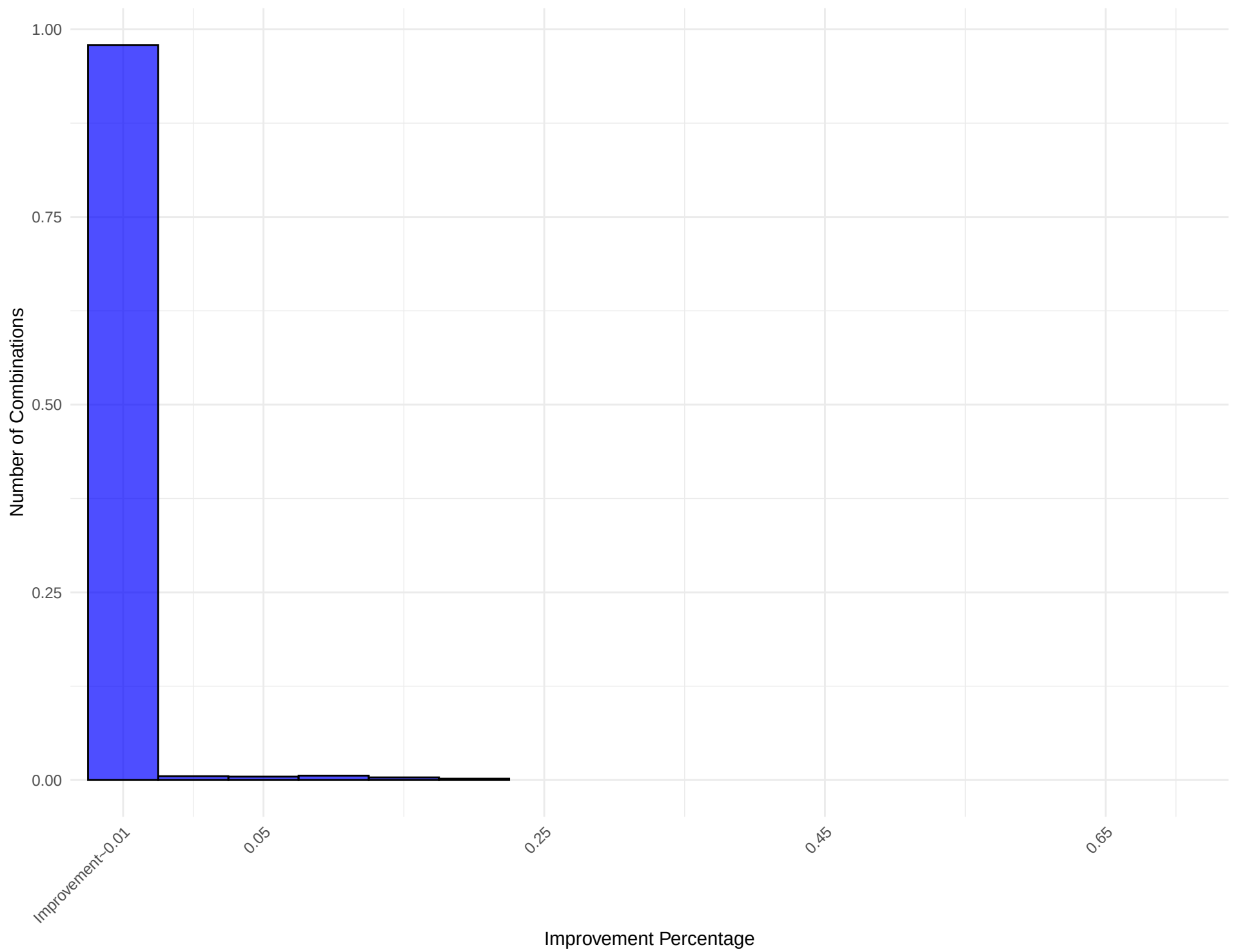
Histogram of Improvement Percentage for Network: small_world_graph_16
