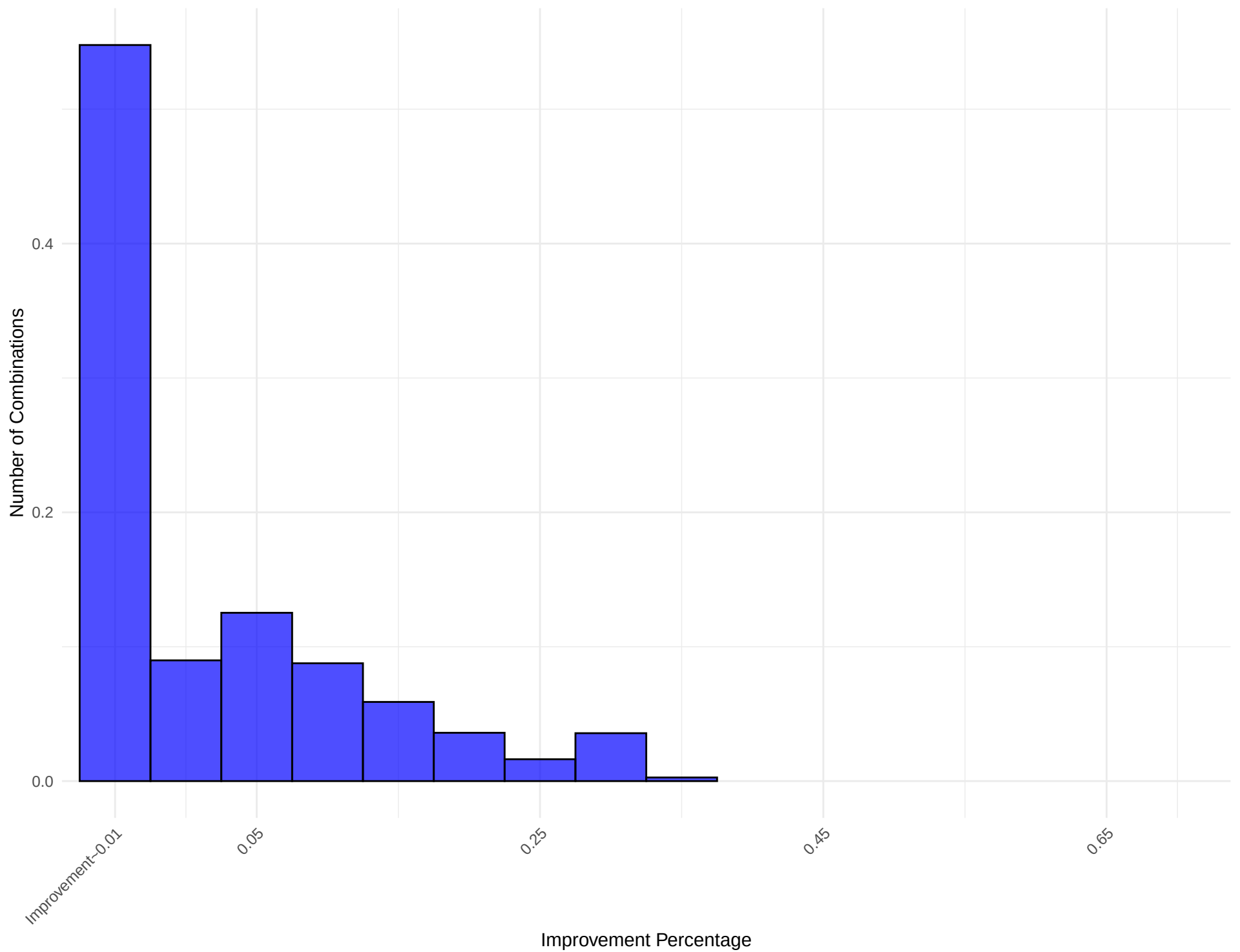
Histogram of Improvement Percentage for Network: small_world_graph_8
