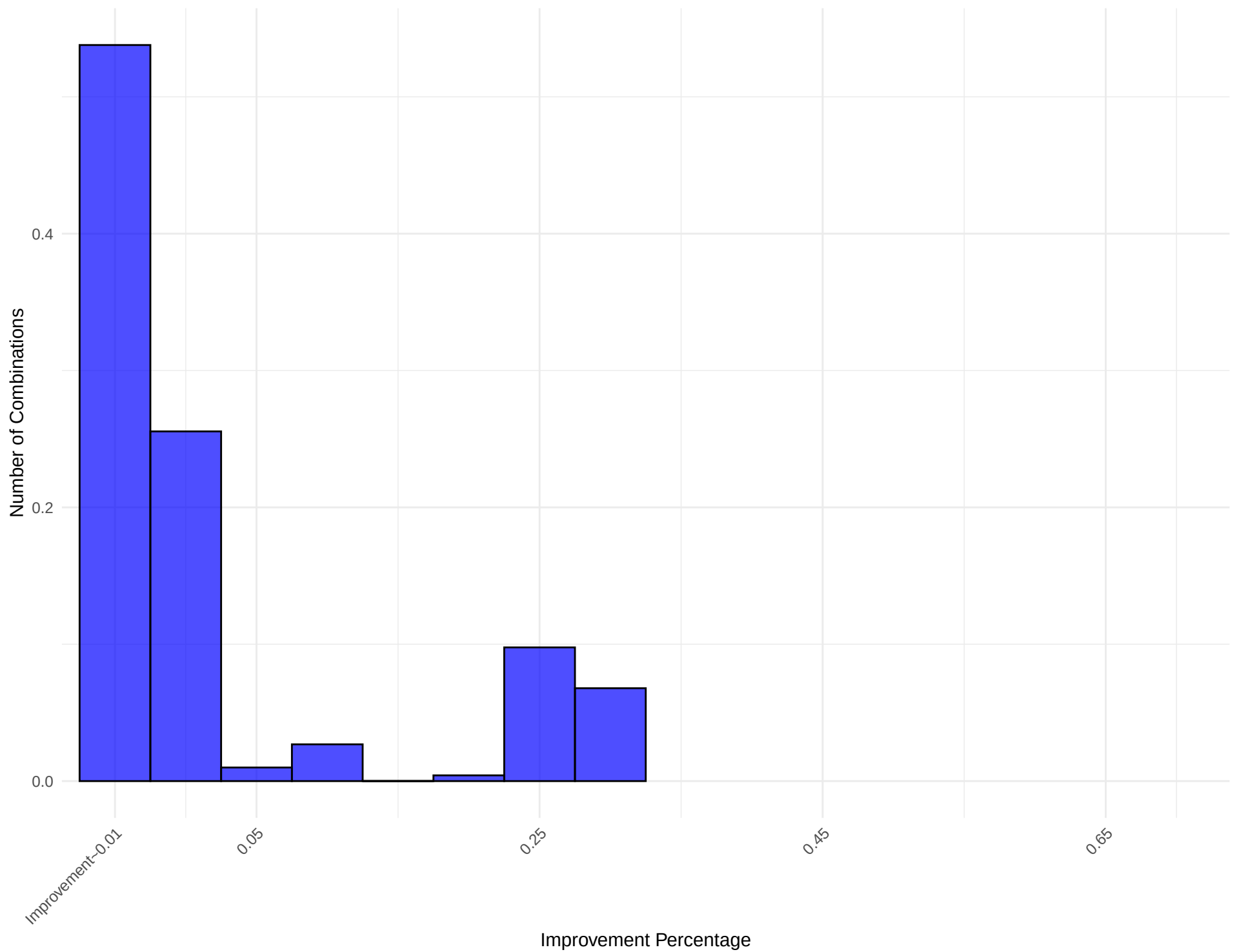
Histogram of Improvement Percentage for Network: small_world_graph_9
