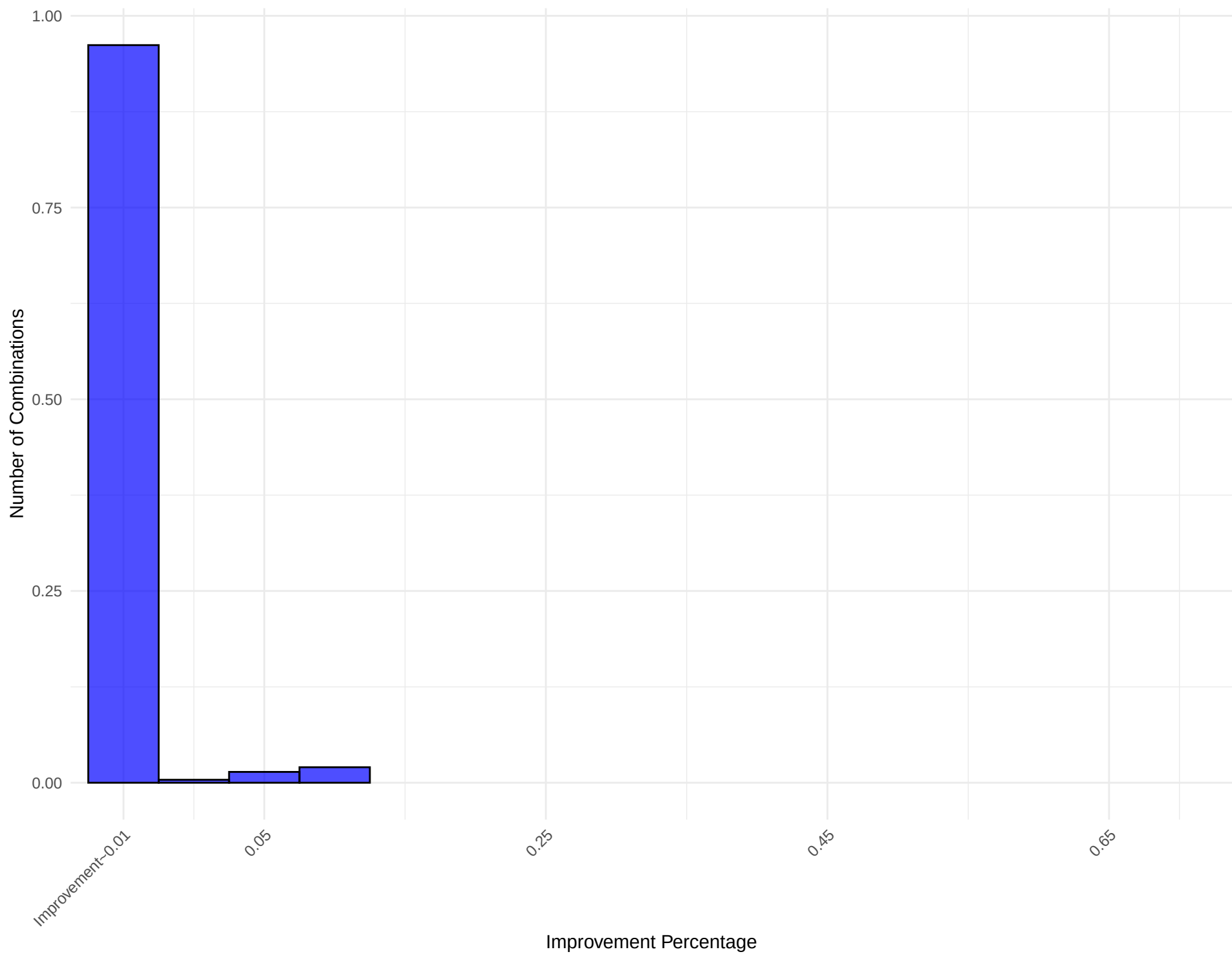
Histogram of Improvement Percentage for Network: edit-alswikiquote
