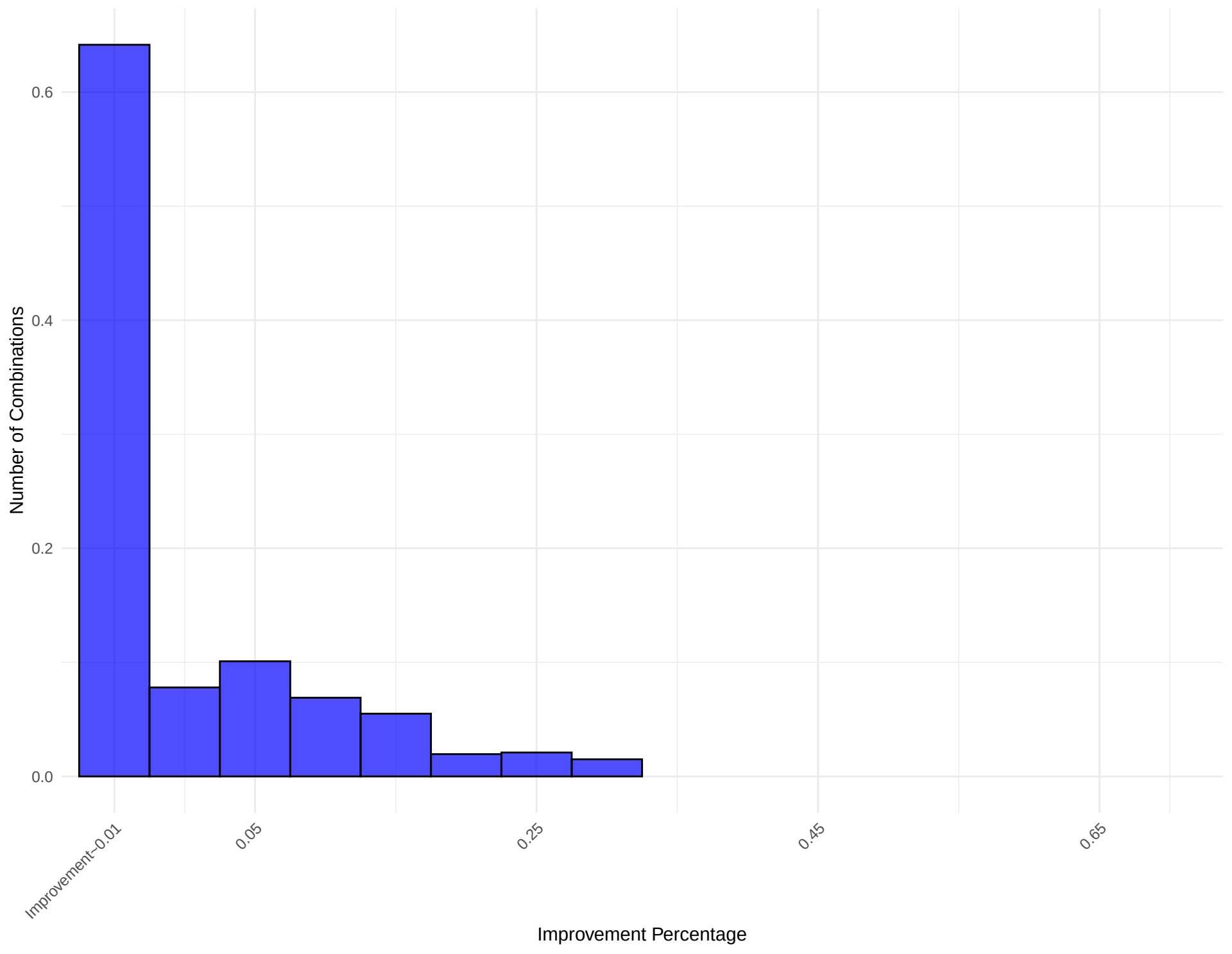
Histogram of Improvement Percentage for Network: small_world_graph_12
