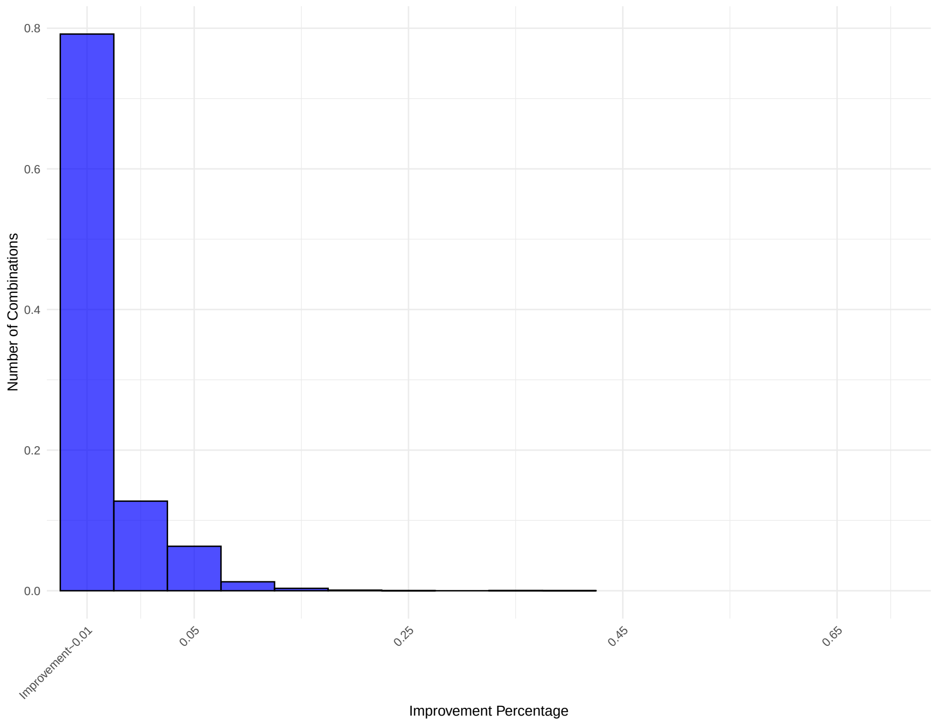
Histogram of Improvement Percentage for Network: hierarchical_graph_10
