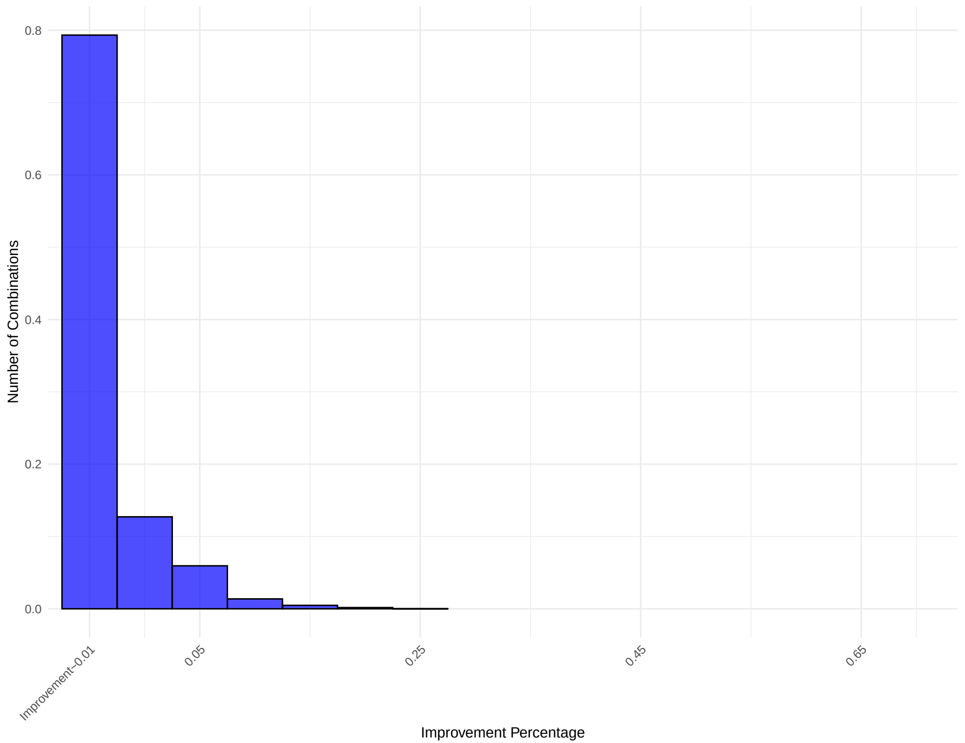
Histogram of Improvement Percentage for Network: barabasi_albert_14
