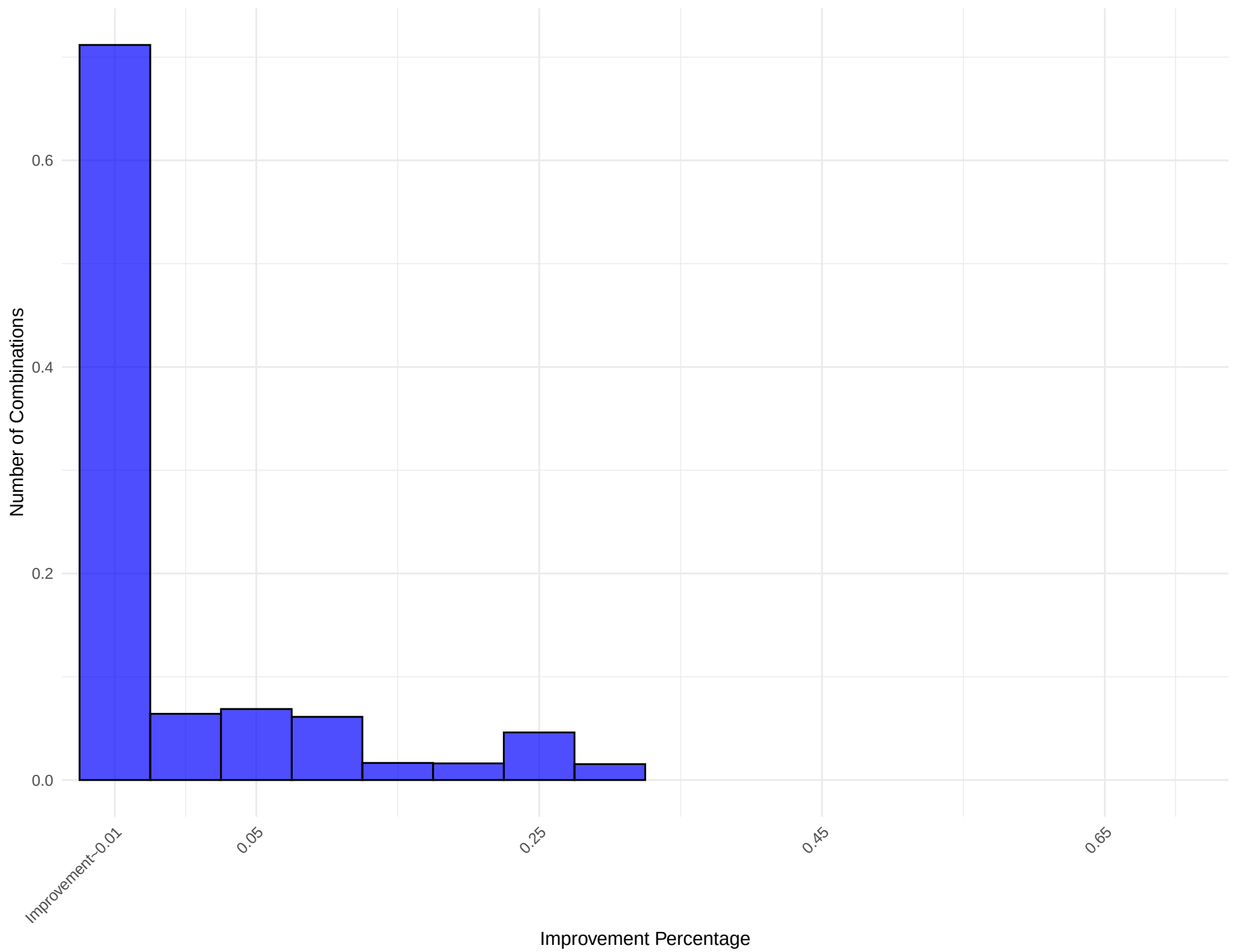
Histogram of Improvement Percentage for Network: edit-gnwikibooks
