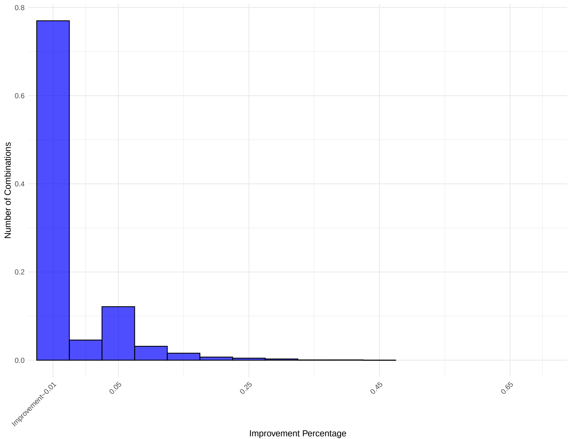
Histogram of Improvement Percentage for Network: hierarchical_graph_5
