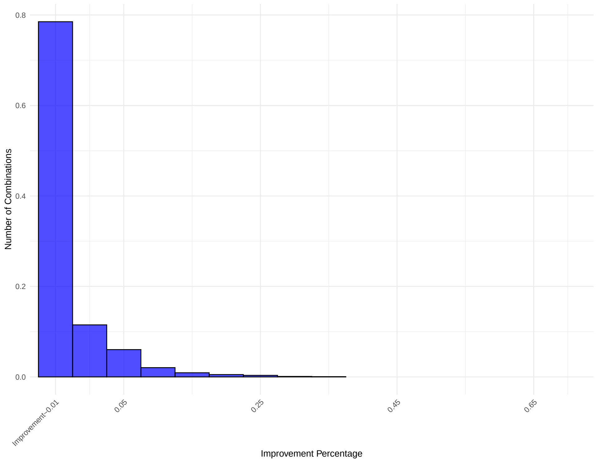
Histogram of Improvement Percentage for Network: barabasi_albert_11
