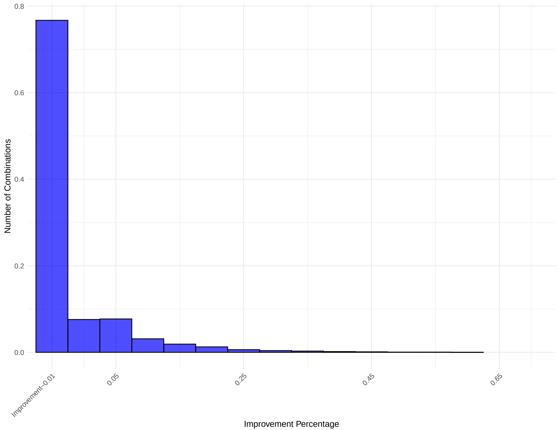
Histogram of Improvement Percentage for Network: barabasi_albert_19
