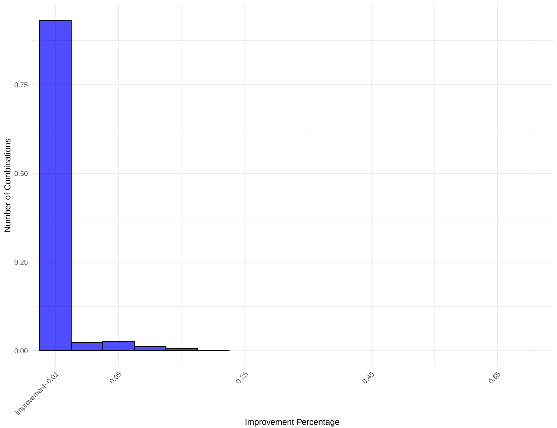
Histogram of Improvement Percentage for Network: hierarchical_graph_14
