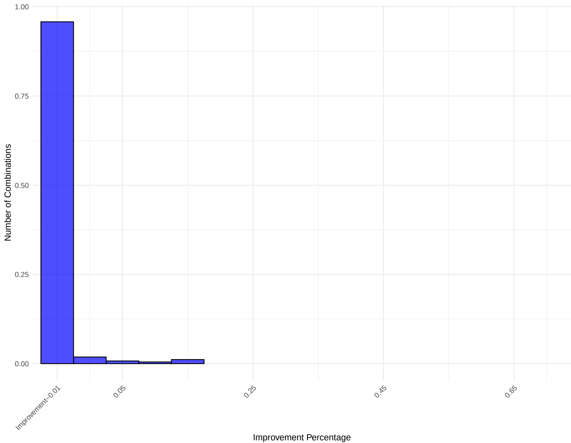
Histogram of Improvement Percentage for Network: edit-lbwikibooks
