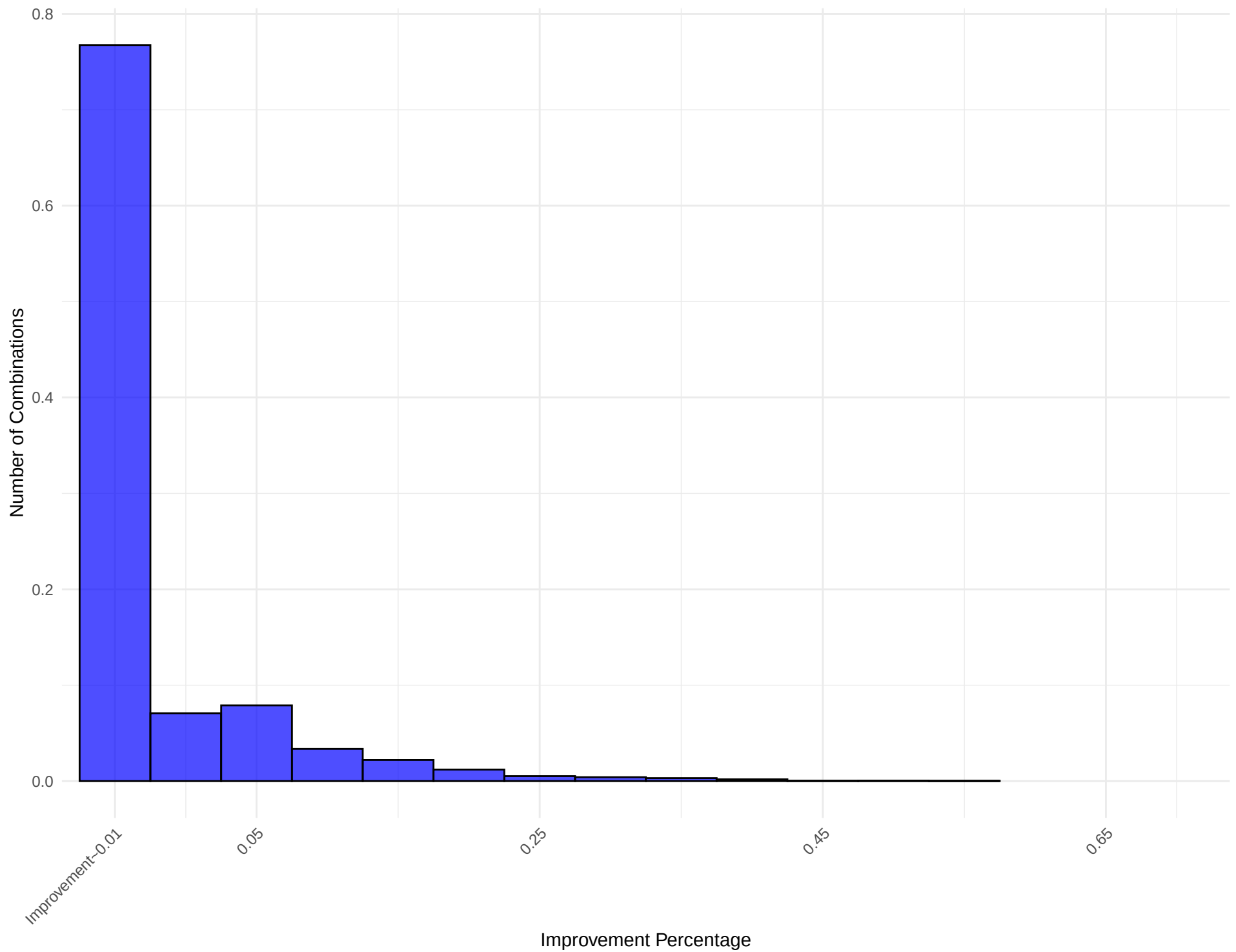
Histogram of Improvement Percentage for Network: barabasi_albert_8
