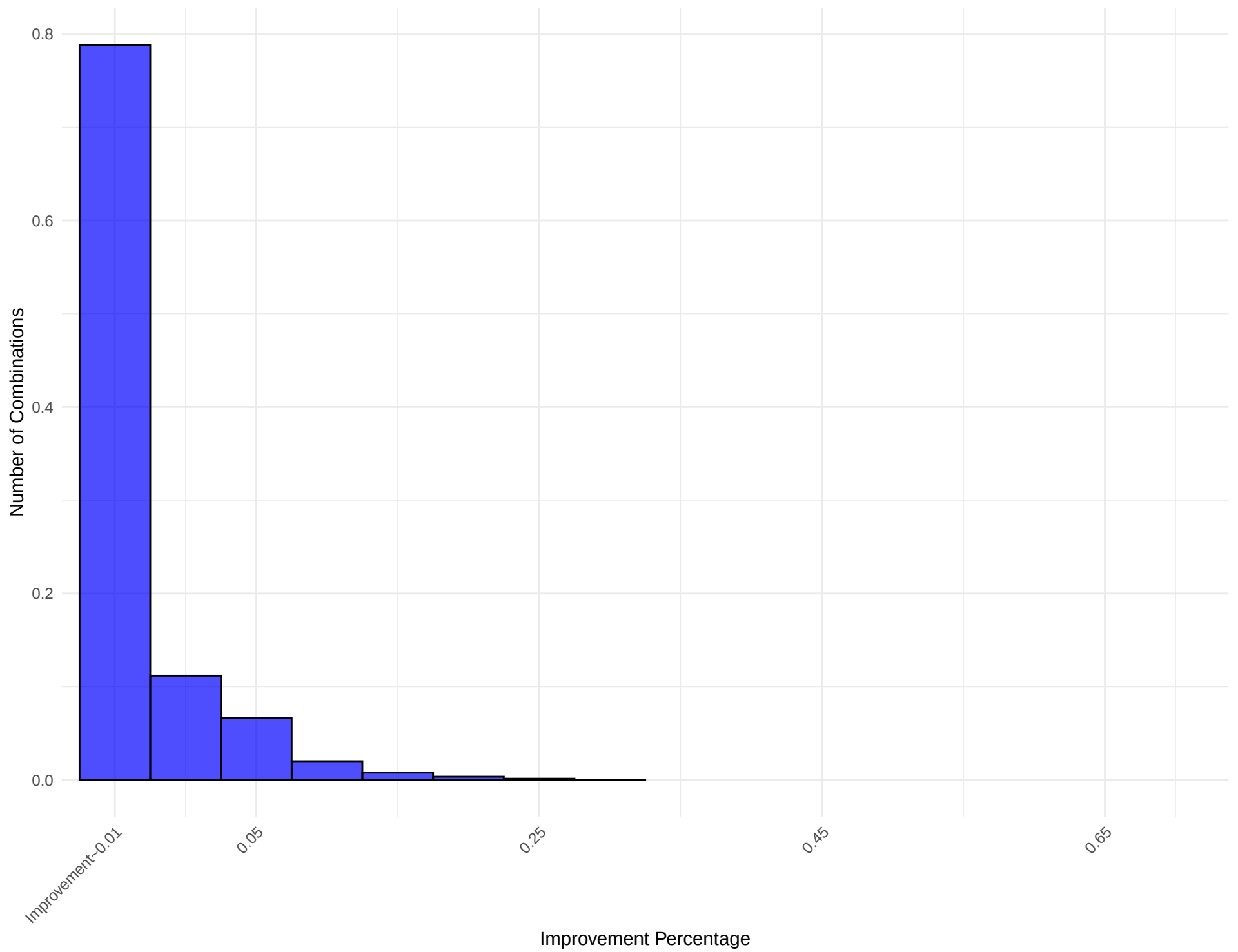
Histogram of Improvement Percentage for Network: barabasi_albert_9
