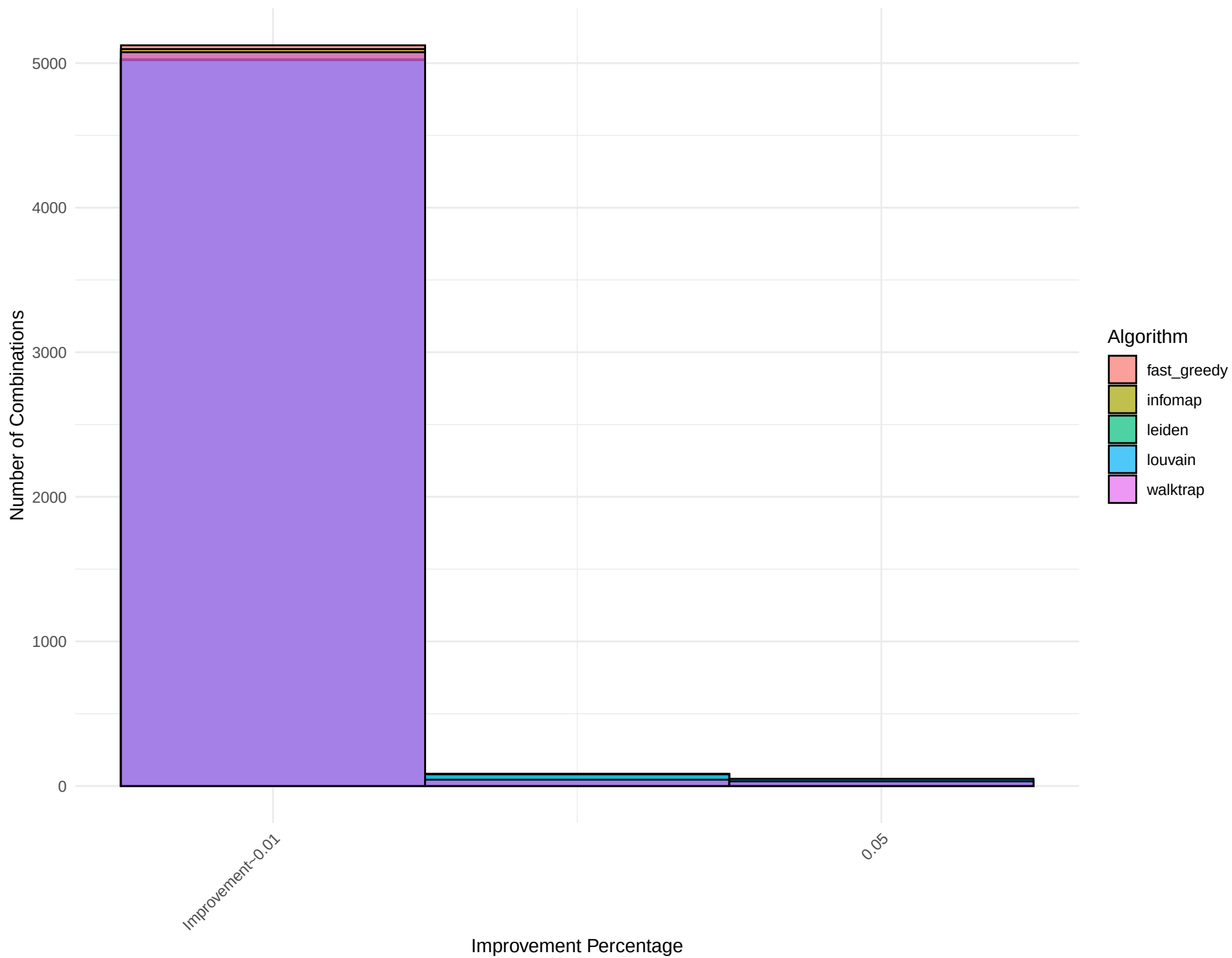
Combined Histogram for Network: edit-nahwikibooks
