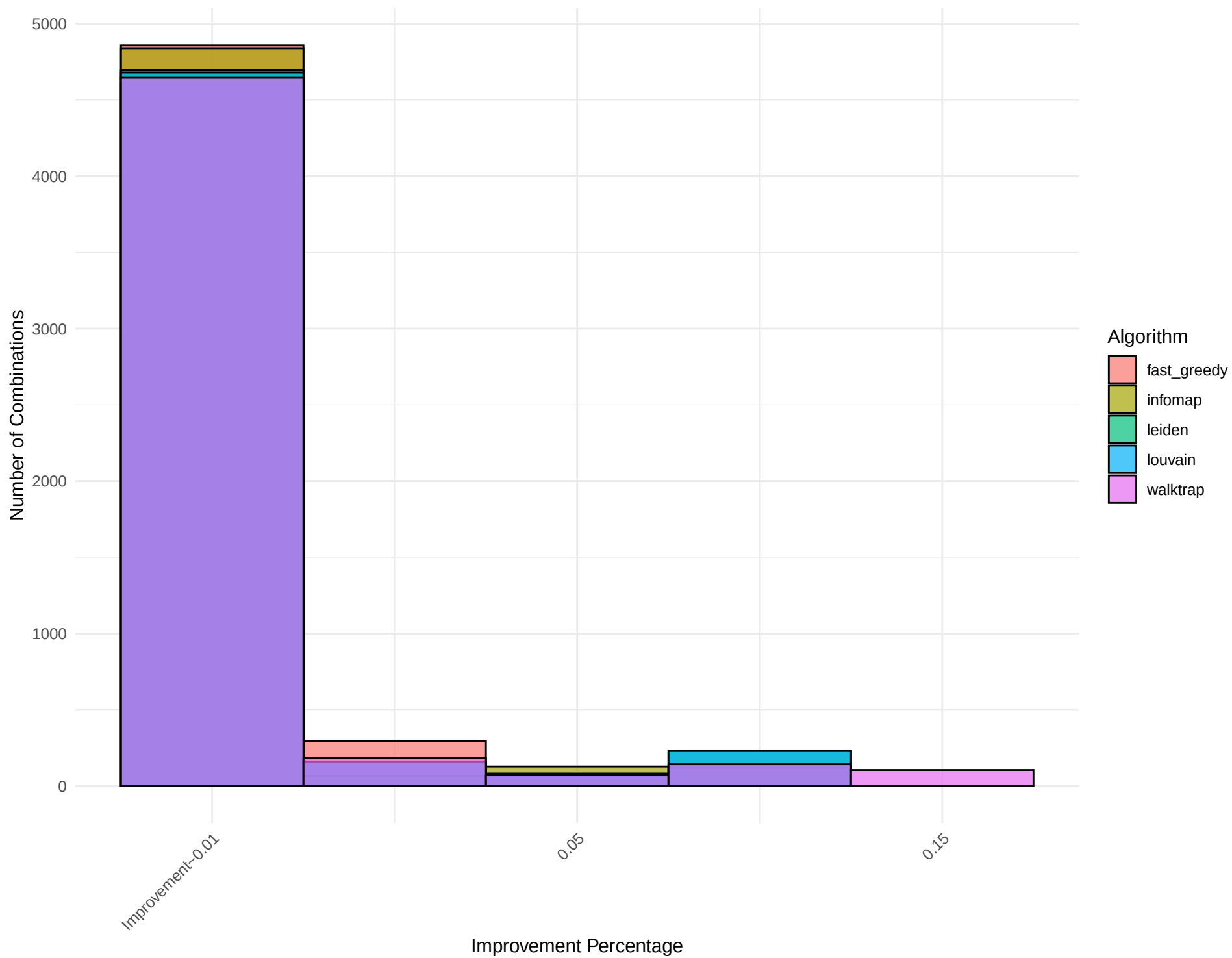
Combined Histogram for Network: edit-aawikibooks
