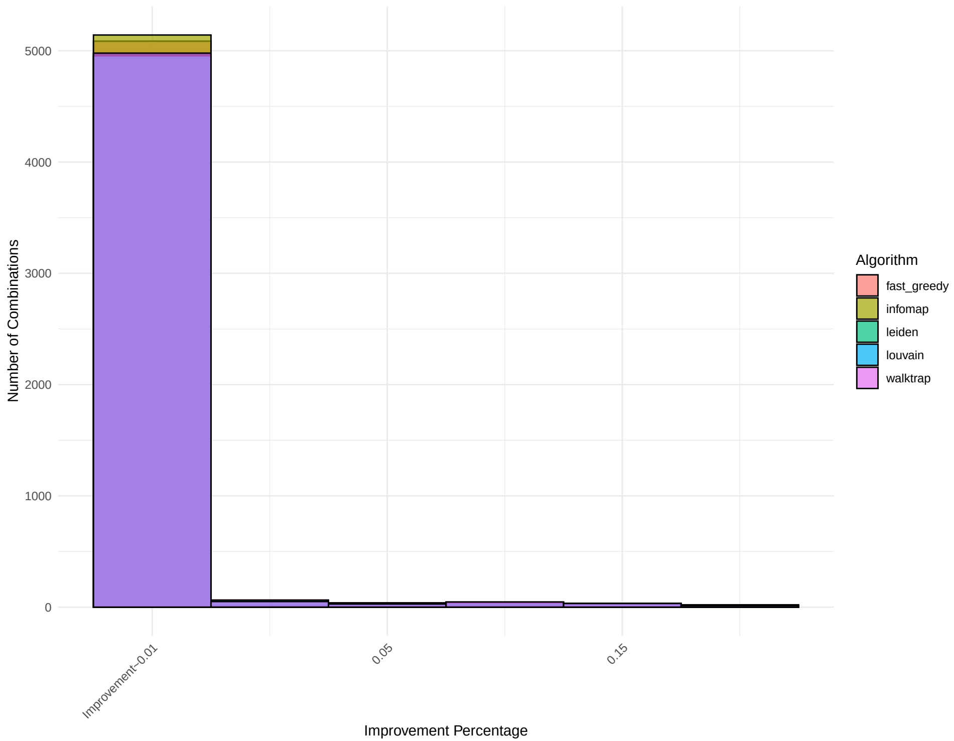
Combined Histogram for Network: small_world_graph_14
