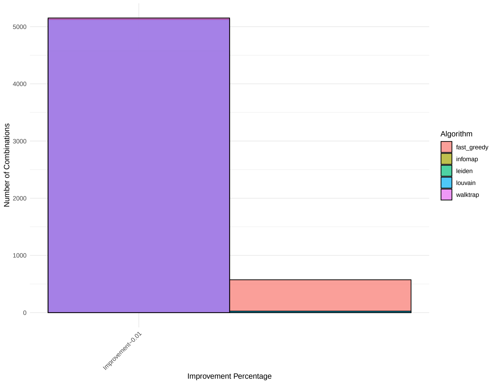
Combined Histogram for Network: edit-dzwiktionary
