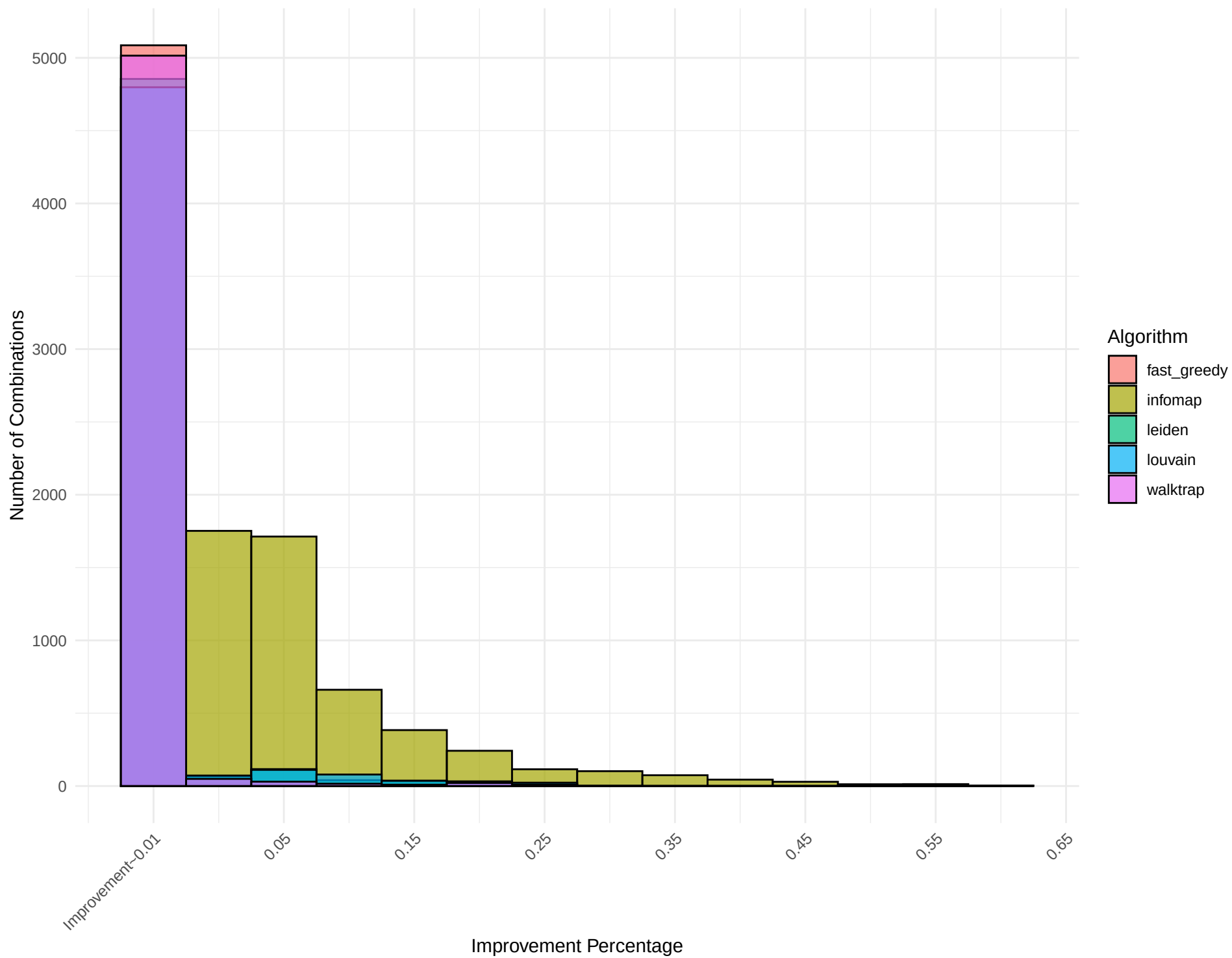
Combined Histogram for Network: barabasi_albert_19
