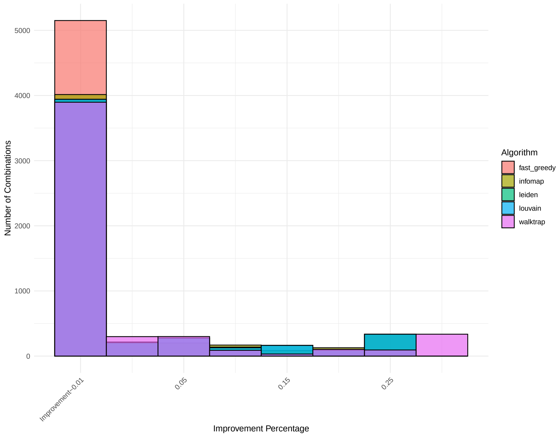
Combined Histogram for Network: hiv
