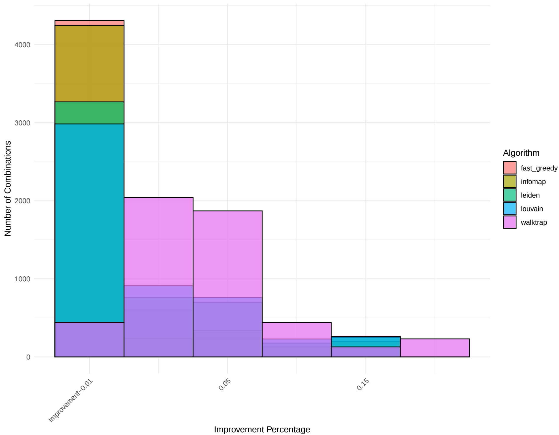
Combined Histogram for Network: edit-tkwikiquote
