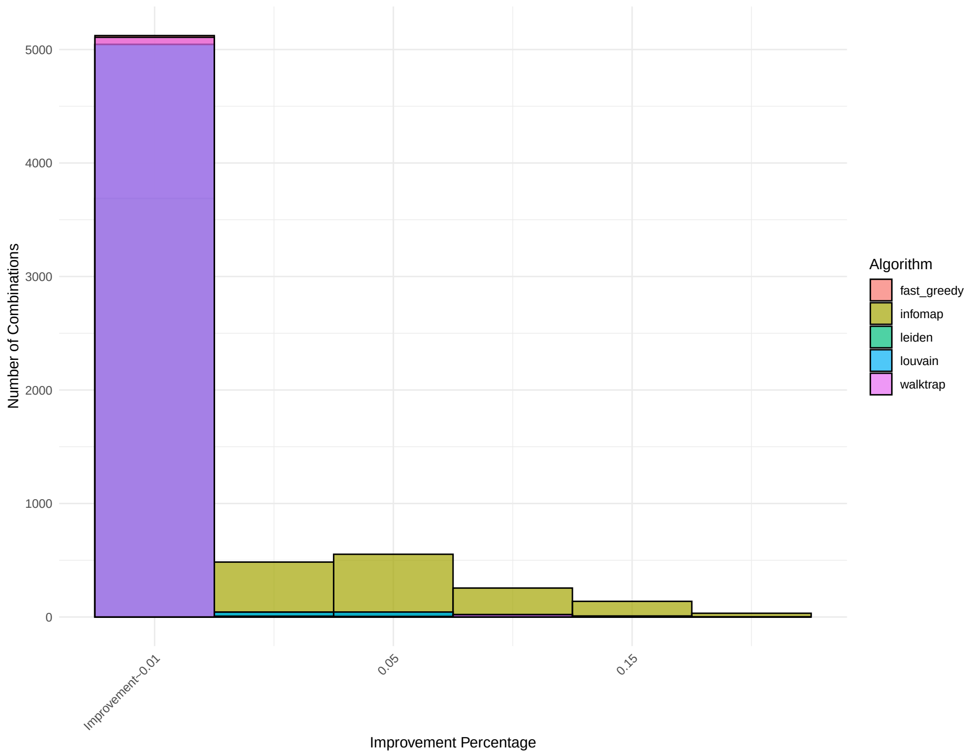
Combined Histogram for Network: hierarchical_graph_14
