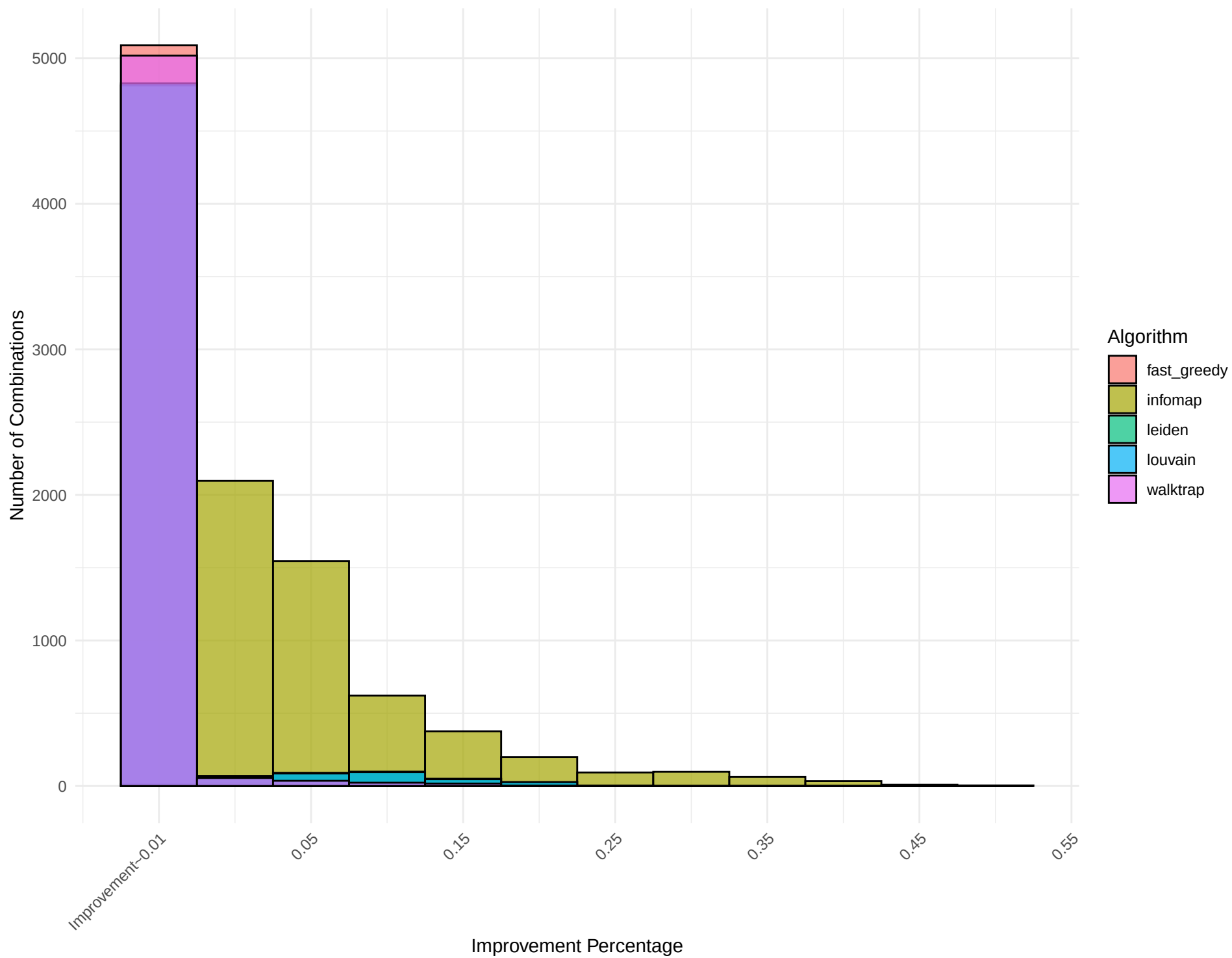
Combined Histogram for Network: barabasi_albert_5
