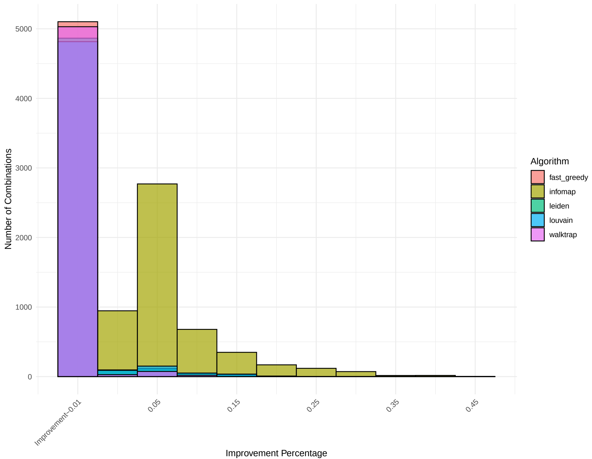
Combined Histogram for Network: hierarchical_graph_5
