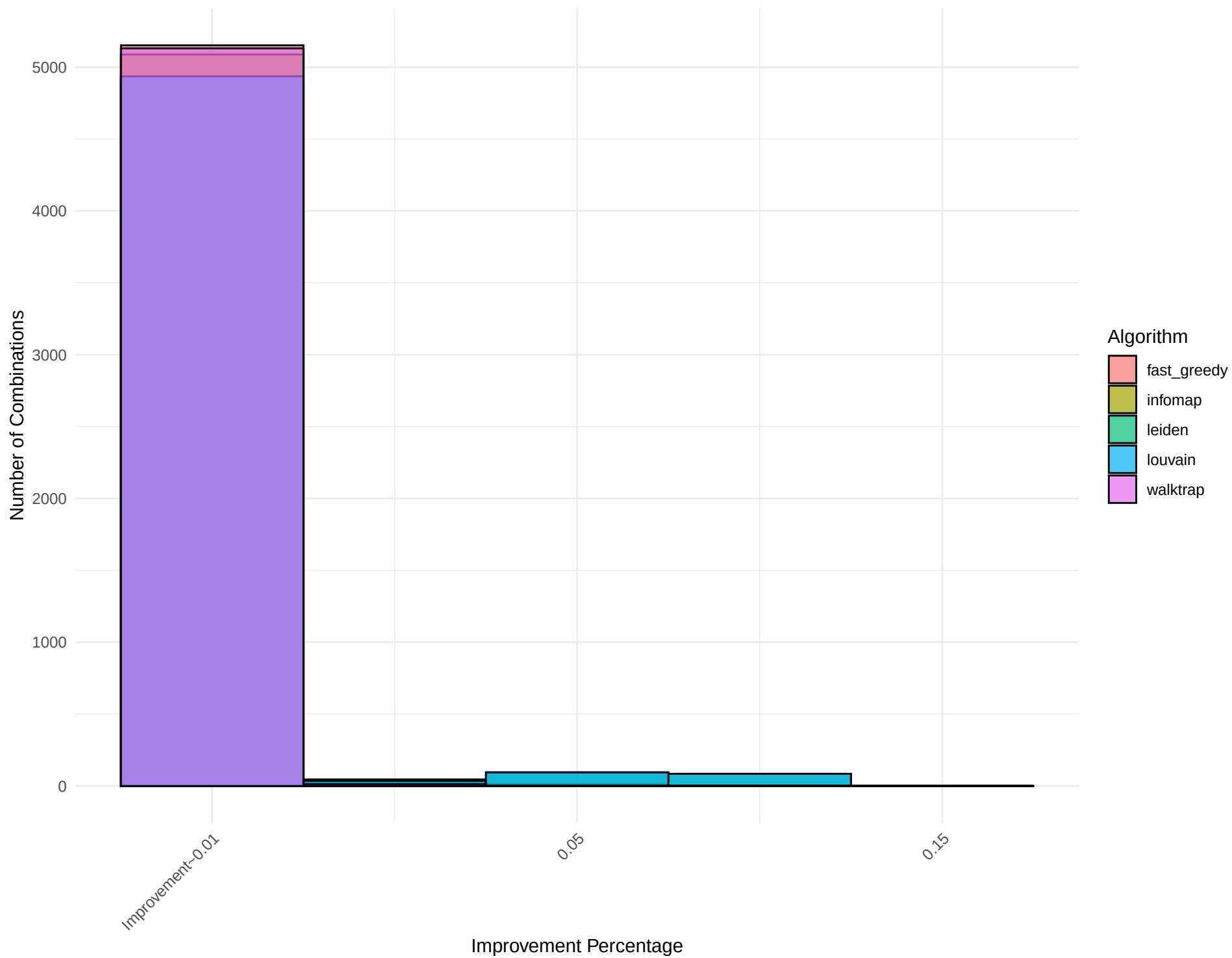
Combined Histogram for Network: brunson_revolution
