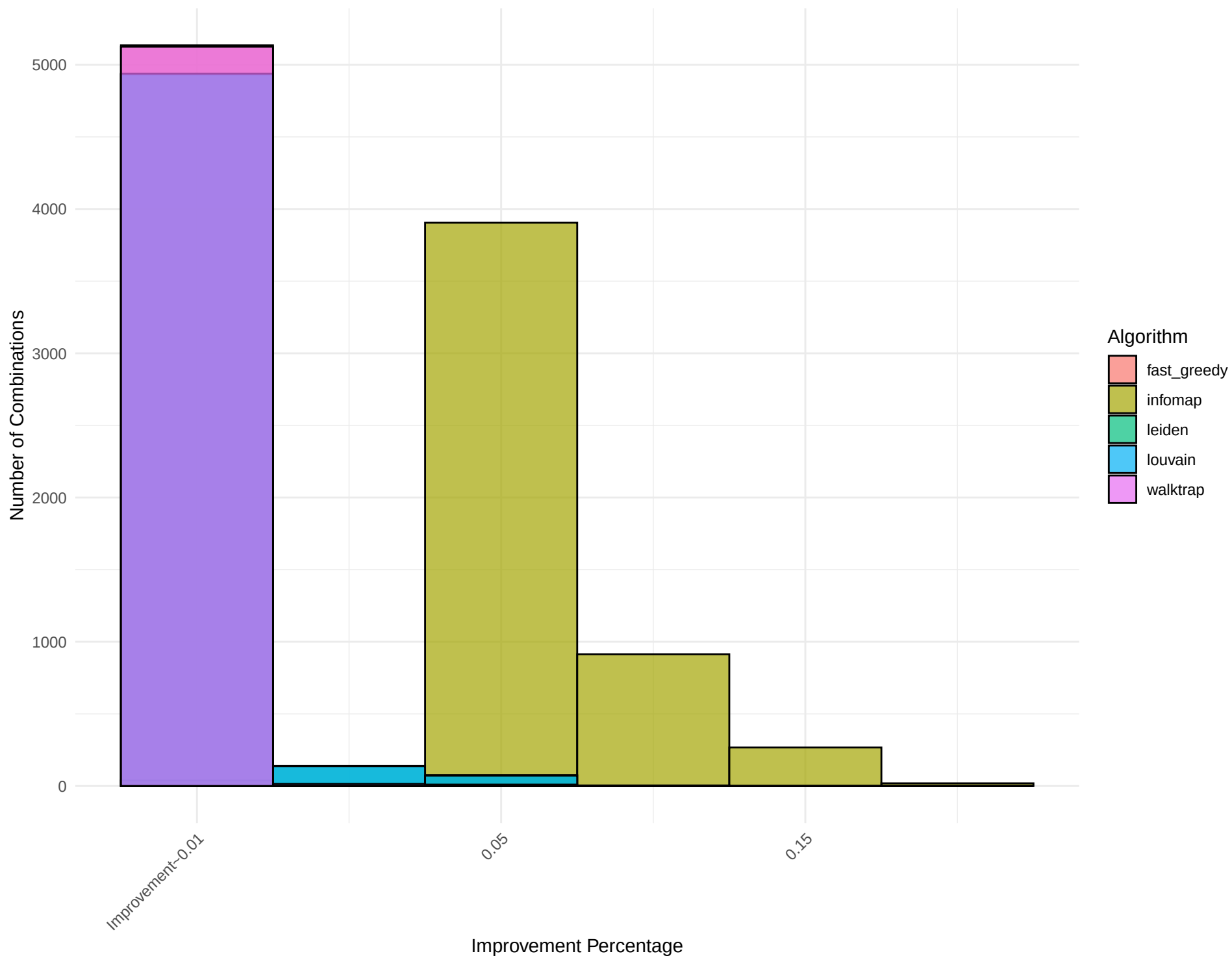
Combined Histogram for Network: ucidata-gama
