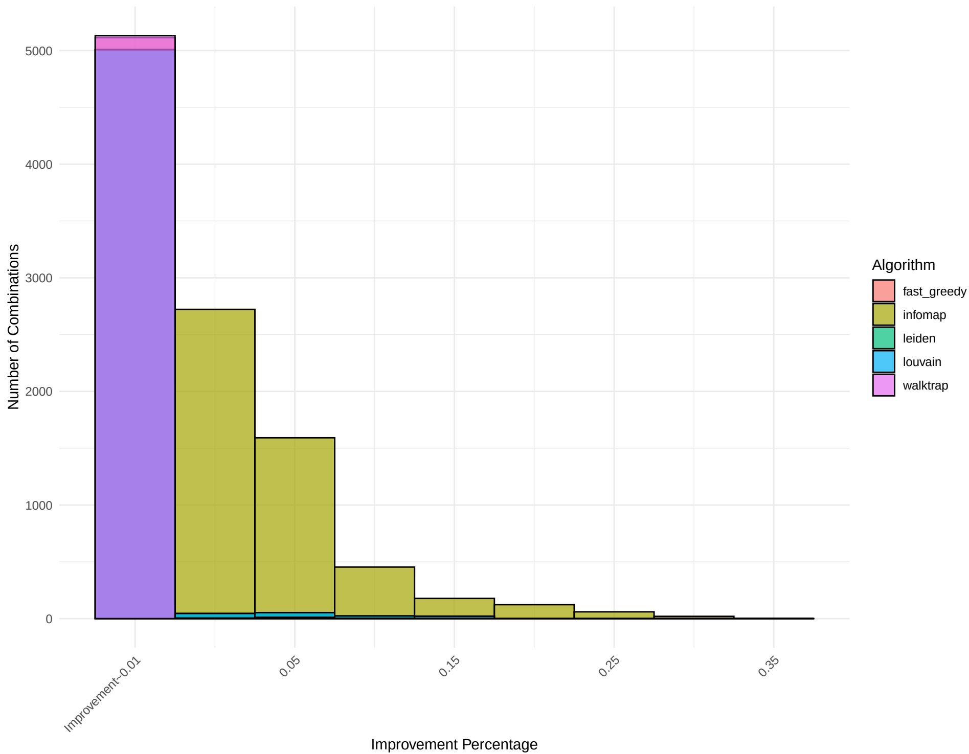
Combined Histogram for Network: barabasi_albert_12
