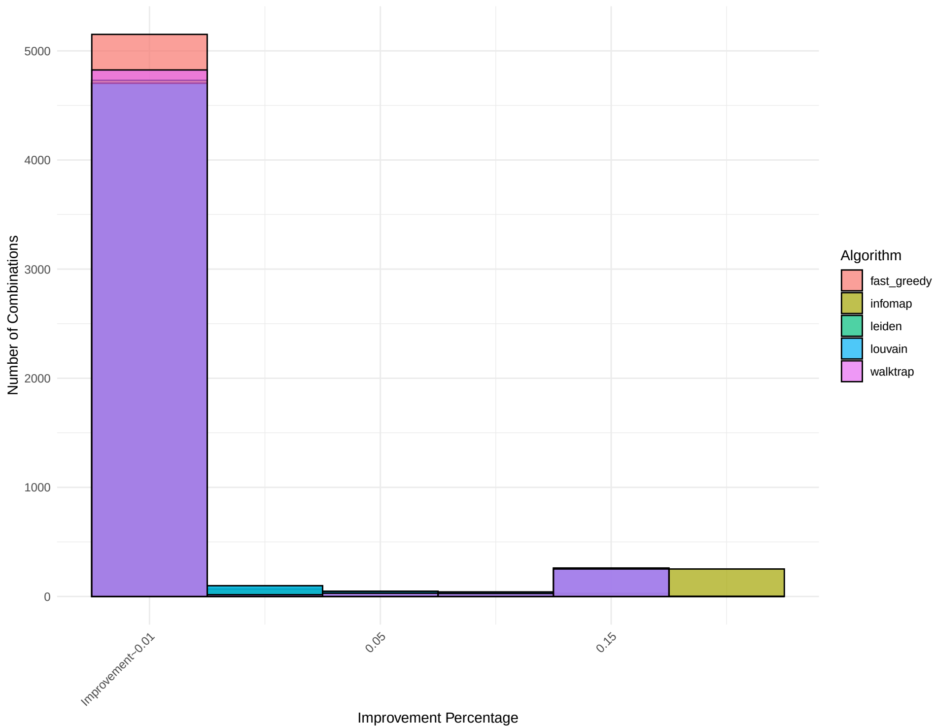
Combined Histogram for Network: barabasi_albert_3
