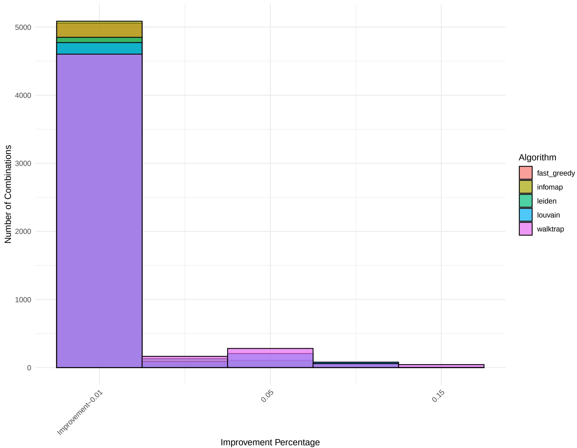
Combined Histogram for Network: ucidata-zachary
