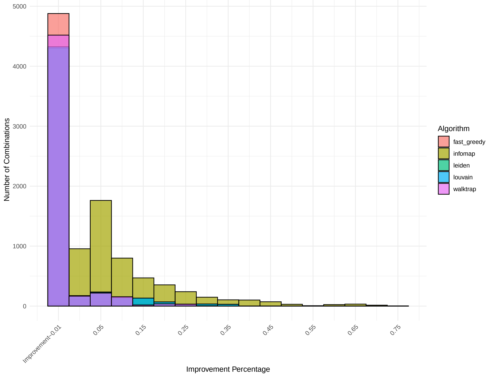
Combined Histogram for Network: hierarchical_graph_9
