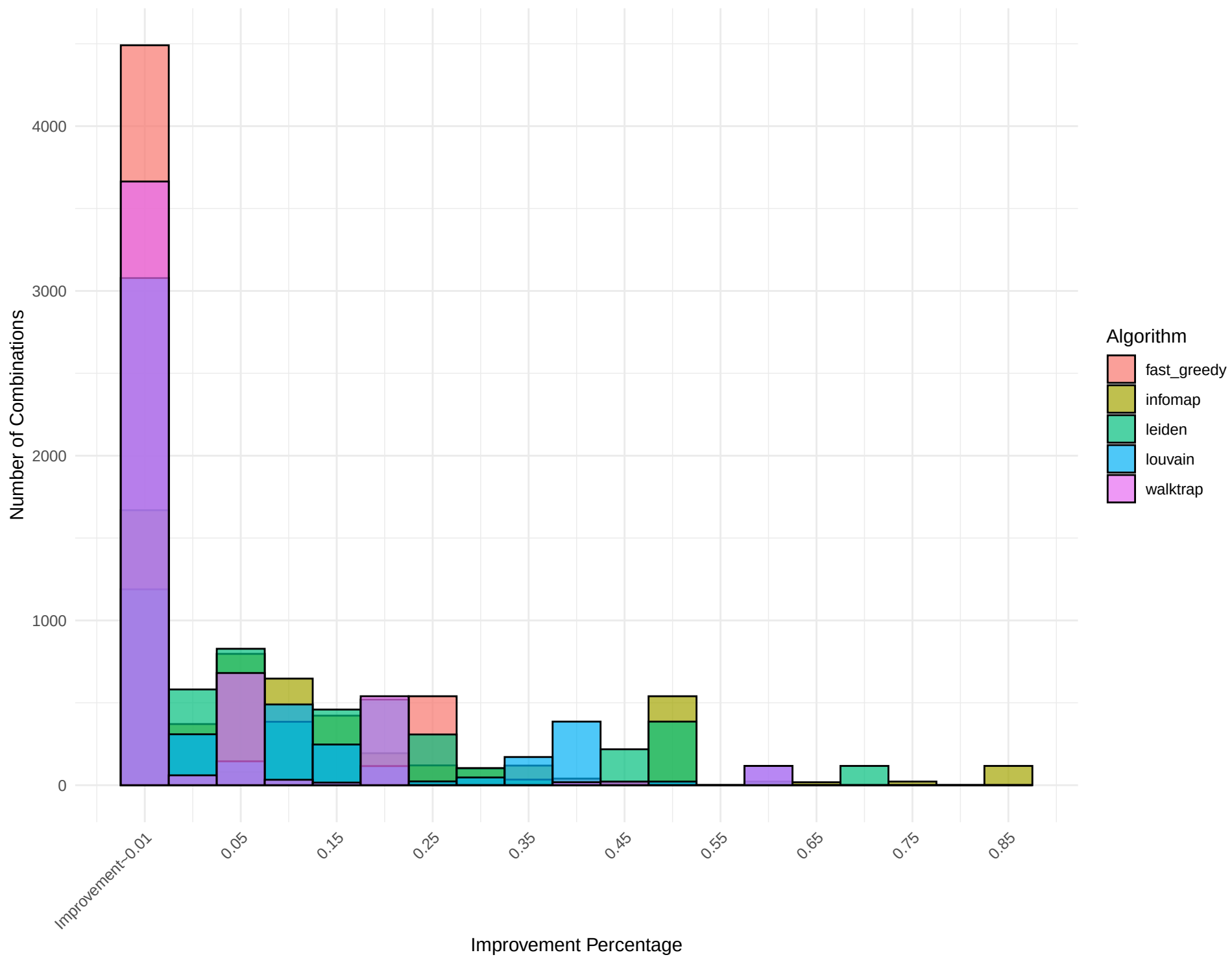
Combined Histogram for Network: brunson_southern-women
