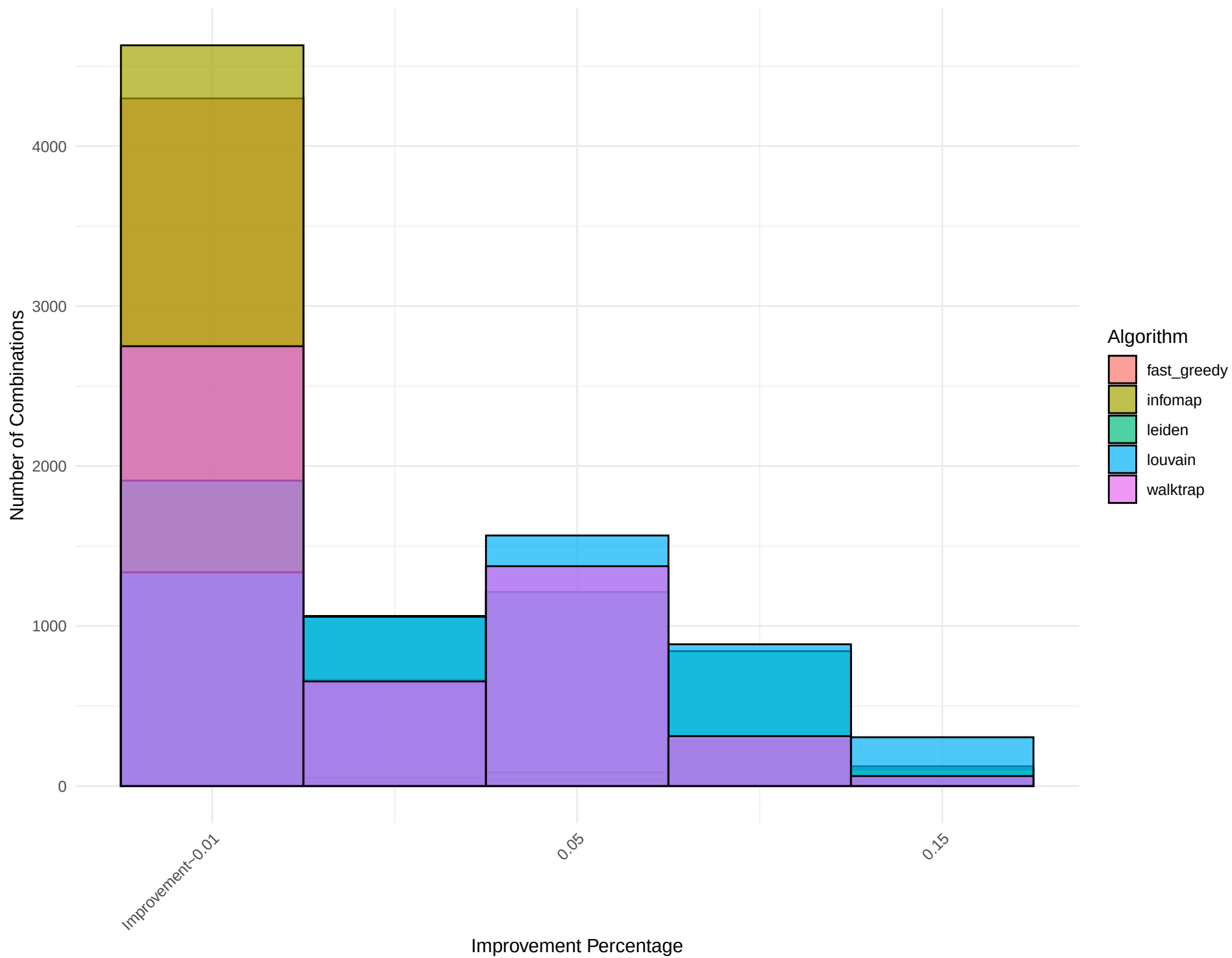
Combined Histogram for Network: small_world_graph_2
