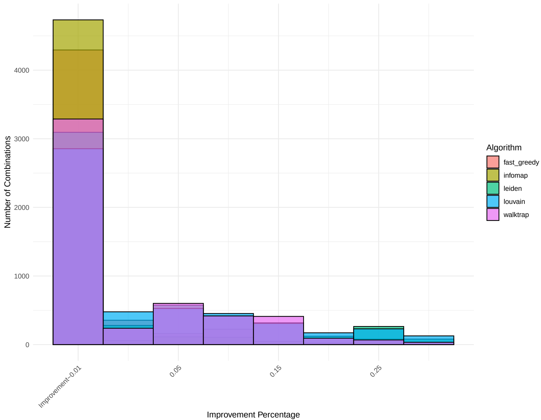
Combined Histogram for Network: small_world_graph_20
