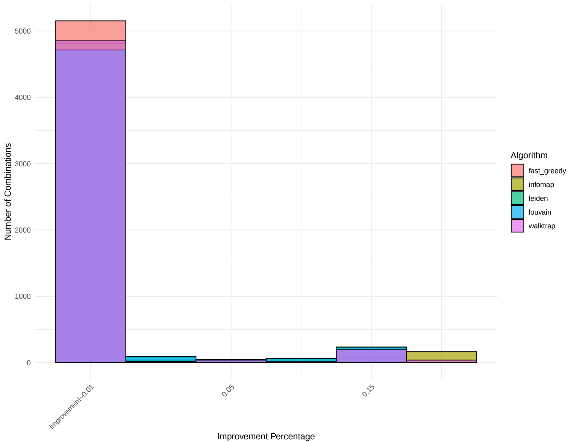
Combined Histogram for Network: barabasi_albert_10
