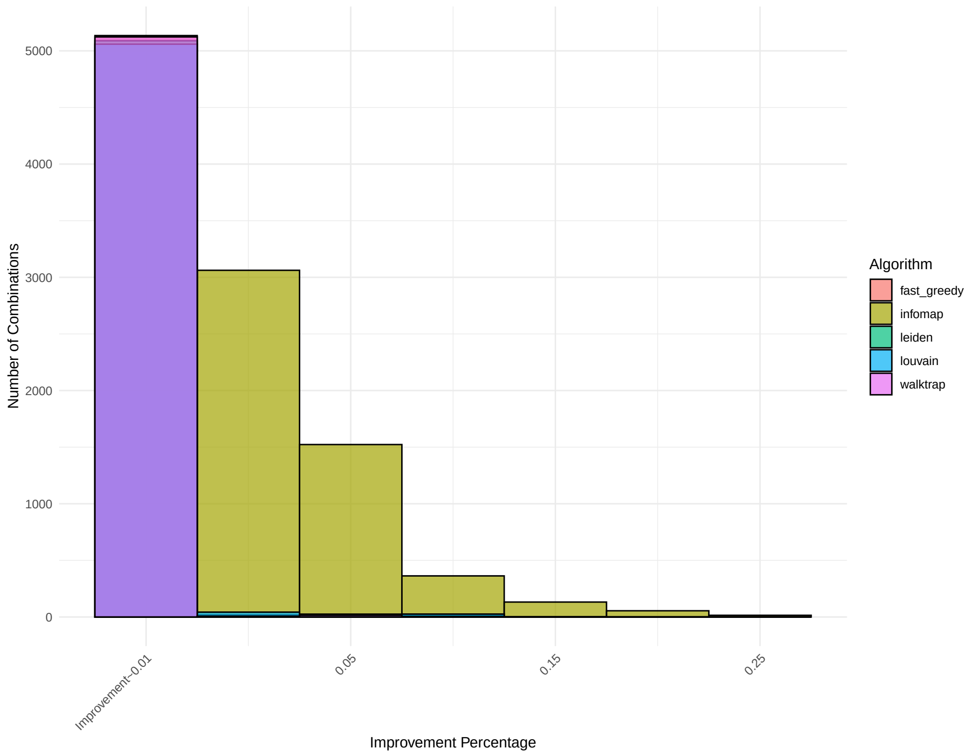
Combined Histogram for Network: barabasi_albert_7
