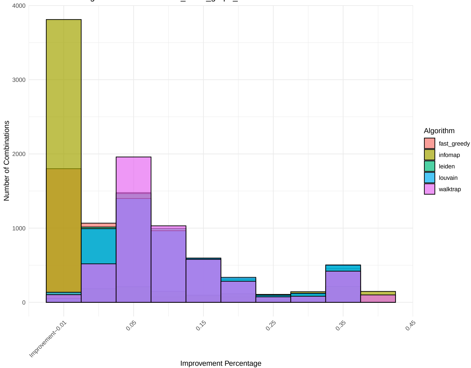
Combined Histogram for Network: small_world_graph_17
