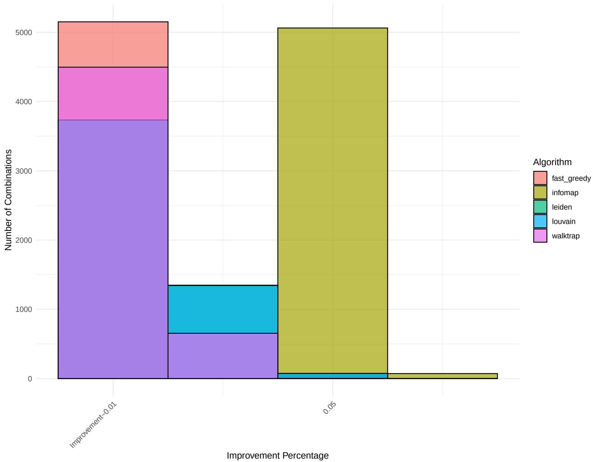
Combined Histogram for Network: moreno_kangaroo
