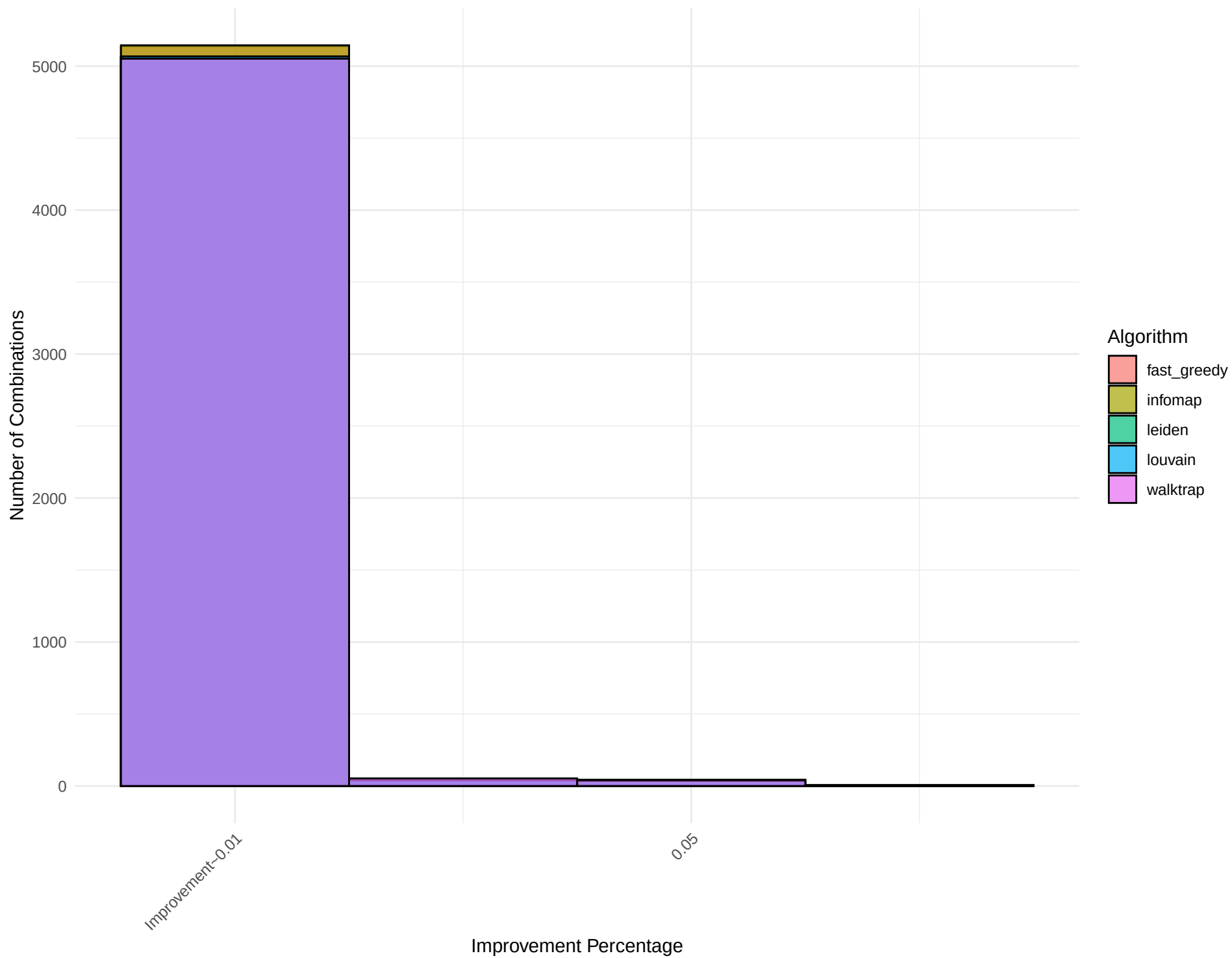
Combined Histogram for Network: small_world_graph_4
