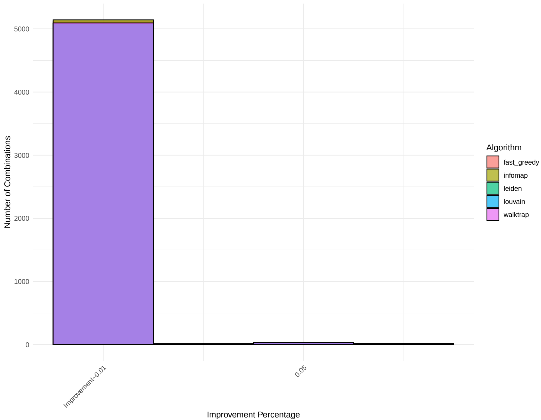
Combined Histogram for Network: hierarchical_graph_4
