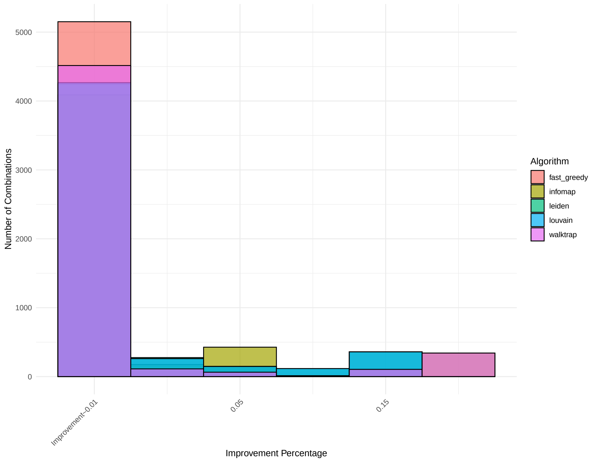
Combined Histogram for Network: barabasi_albert_15
