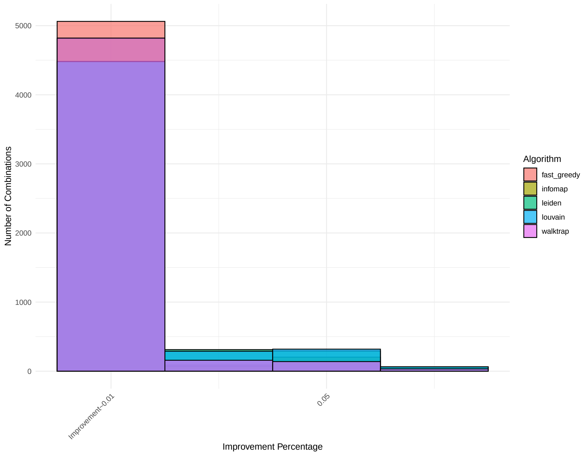
Combined Histogram for Network: contiguous-usa
