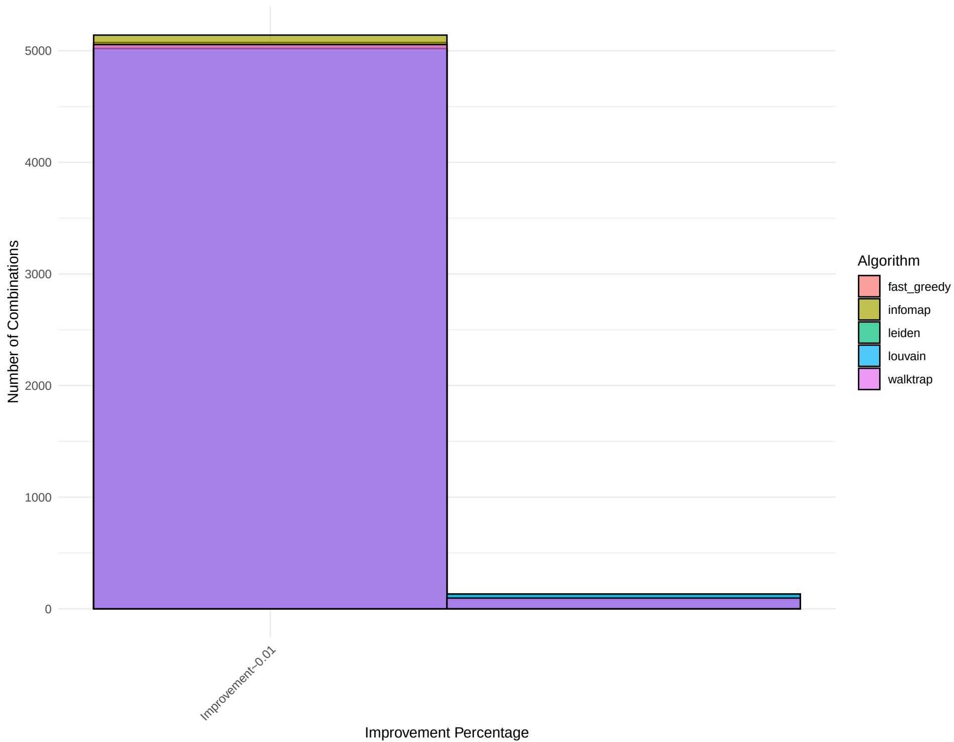
Combined Histogram for Network: hierarchical_graph_6
