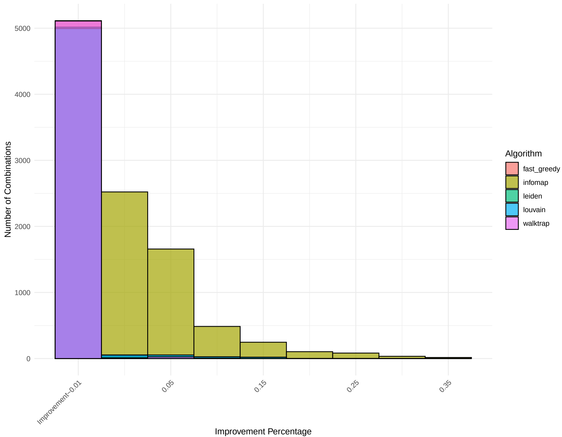
Combined Histogram for Network: barabasi_albert_2
