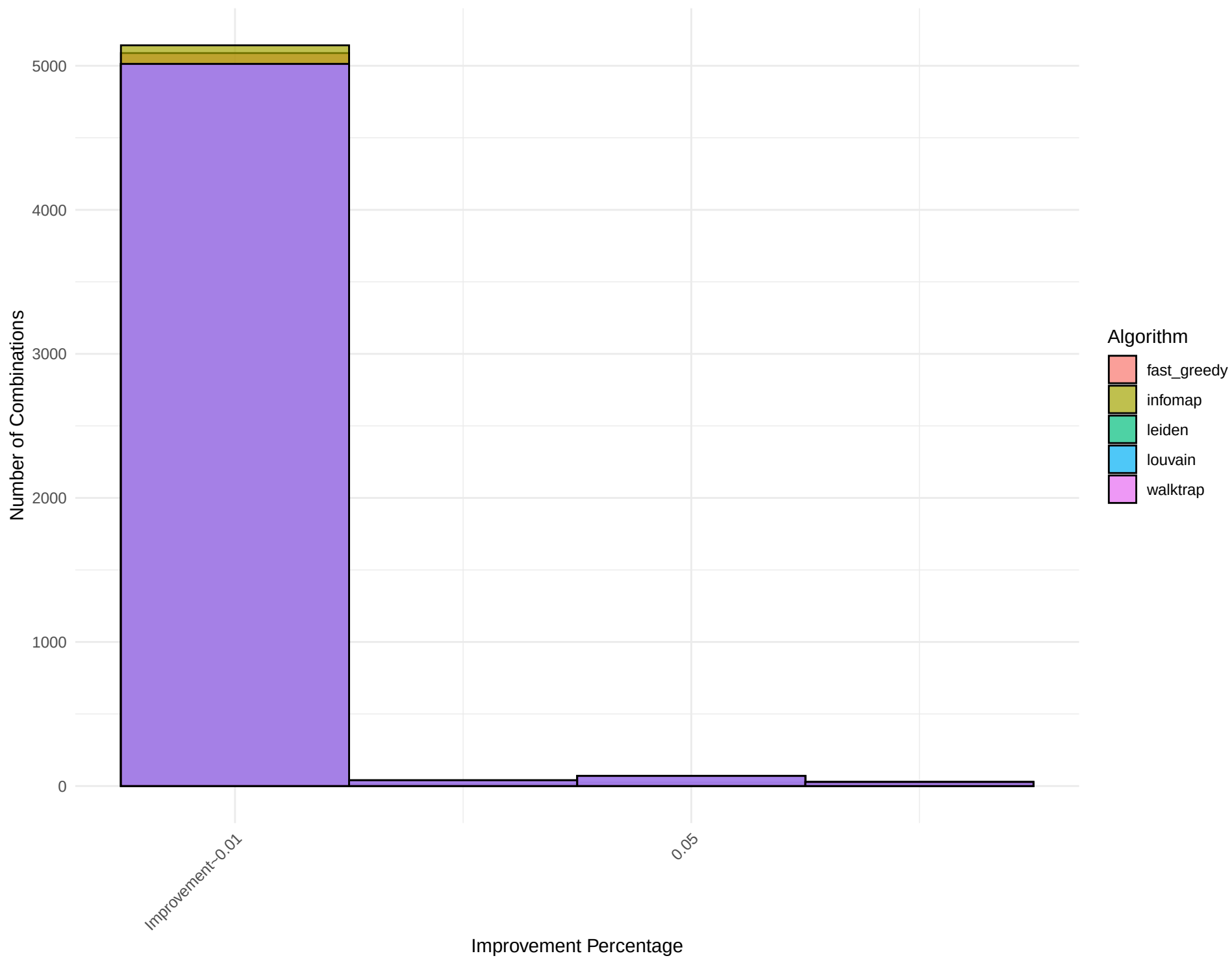
Combined Histogram for Network: hierarchical_graph_16
