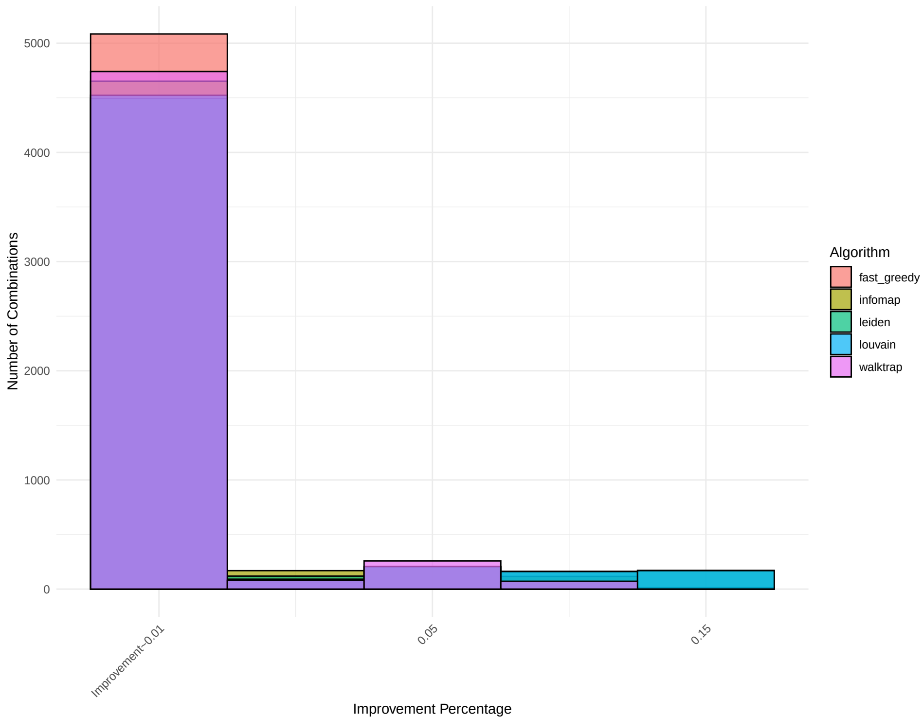
Combined Histogram for Network: edit-mhwiktionary
