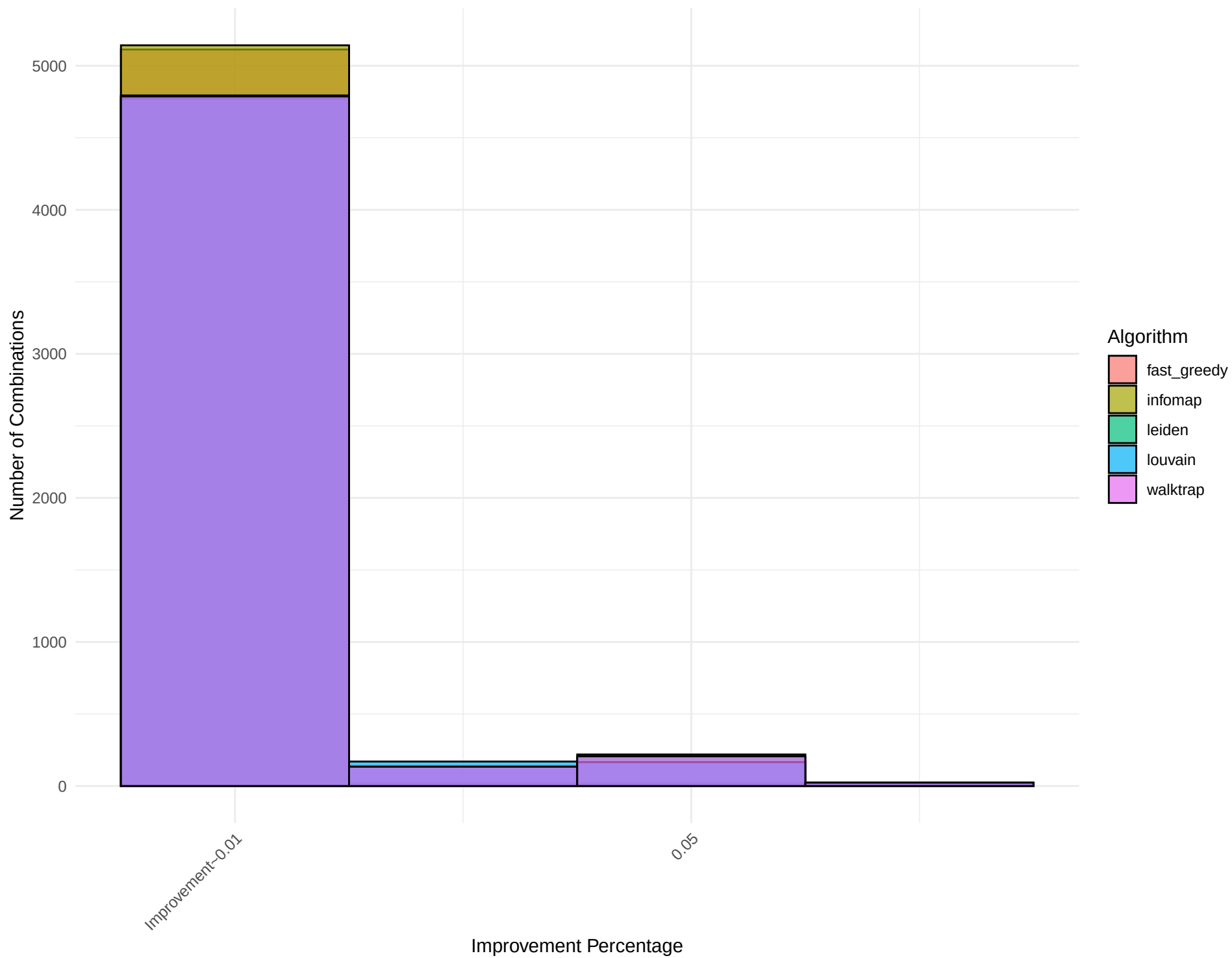
Combined Histogram for Network: small_world_graph_19
