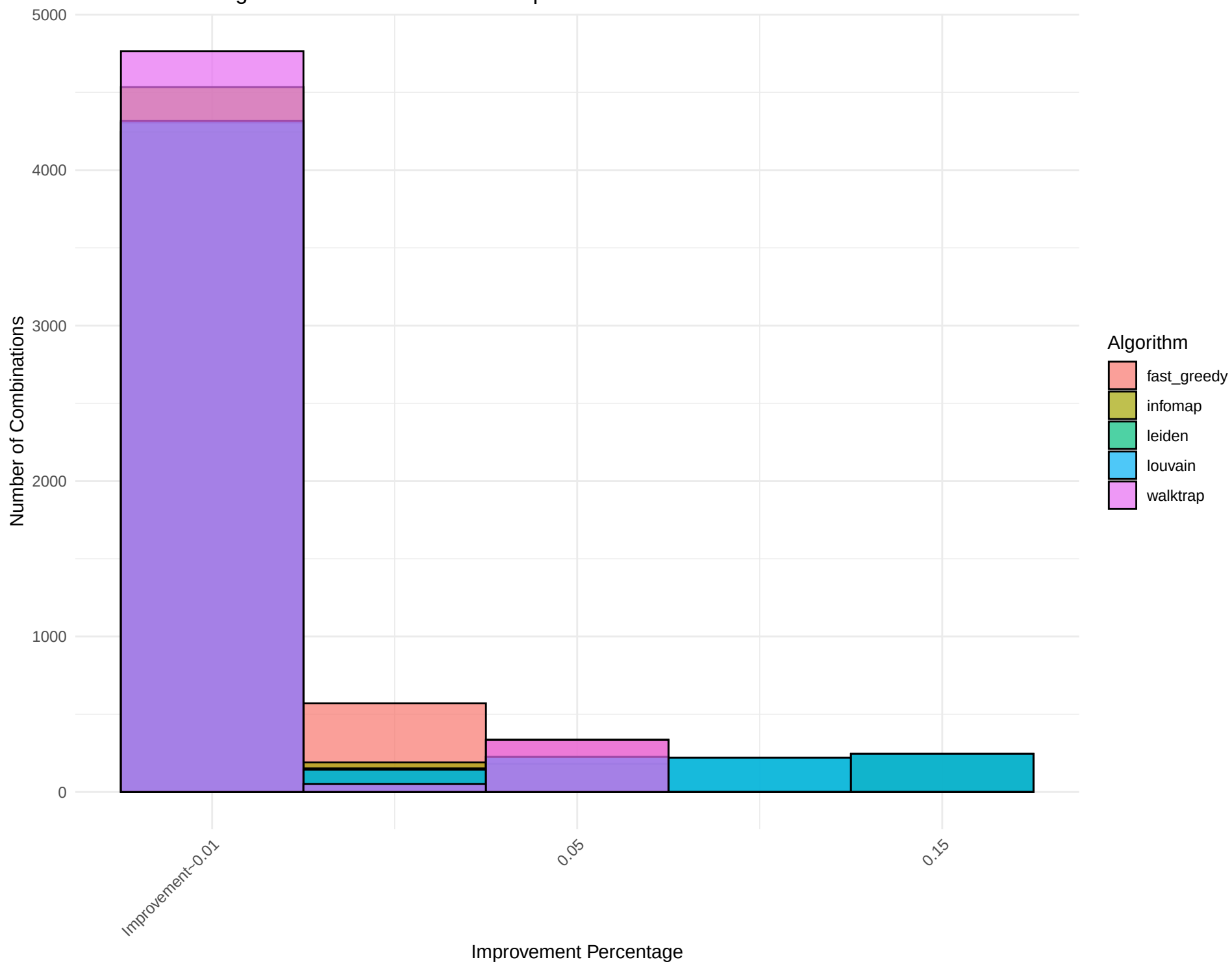
Combined Histogram for Network: edit-krwikiquote
