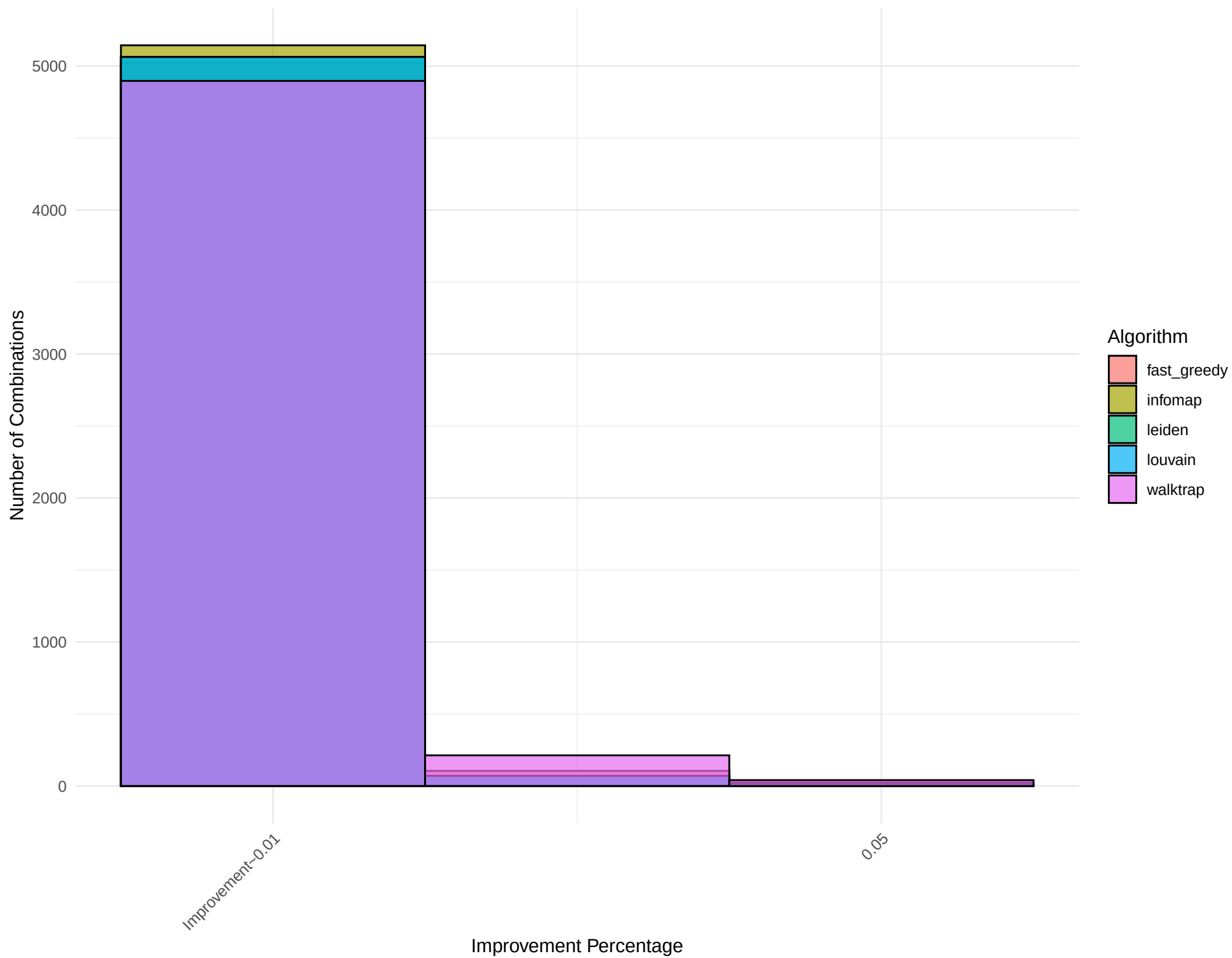
Combined Histogram for Network: dimacs10-polbooks
