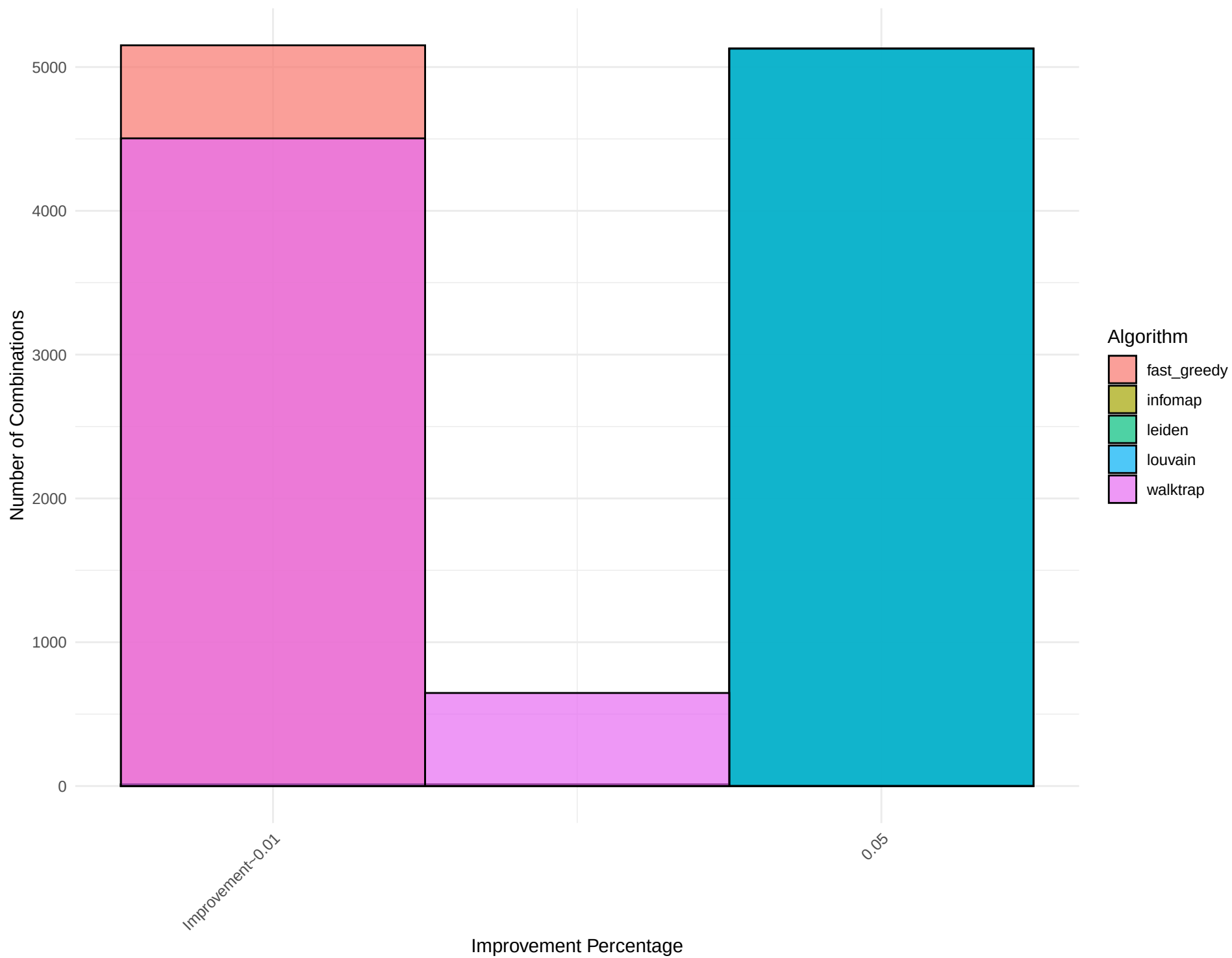
Combined Histogram for Network: league-fr1-2016
