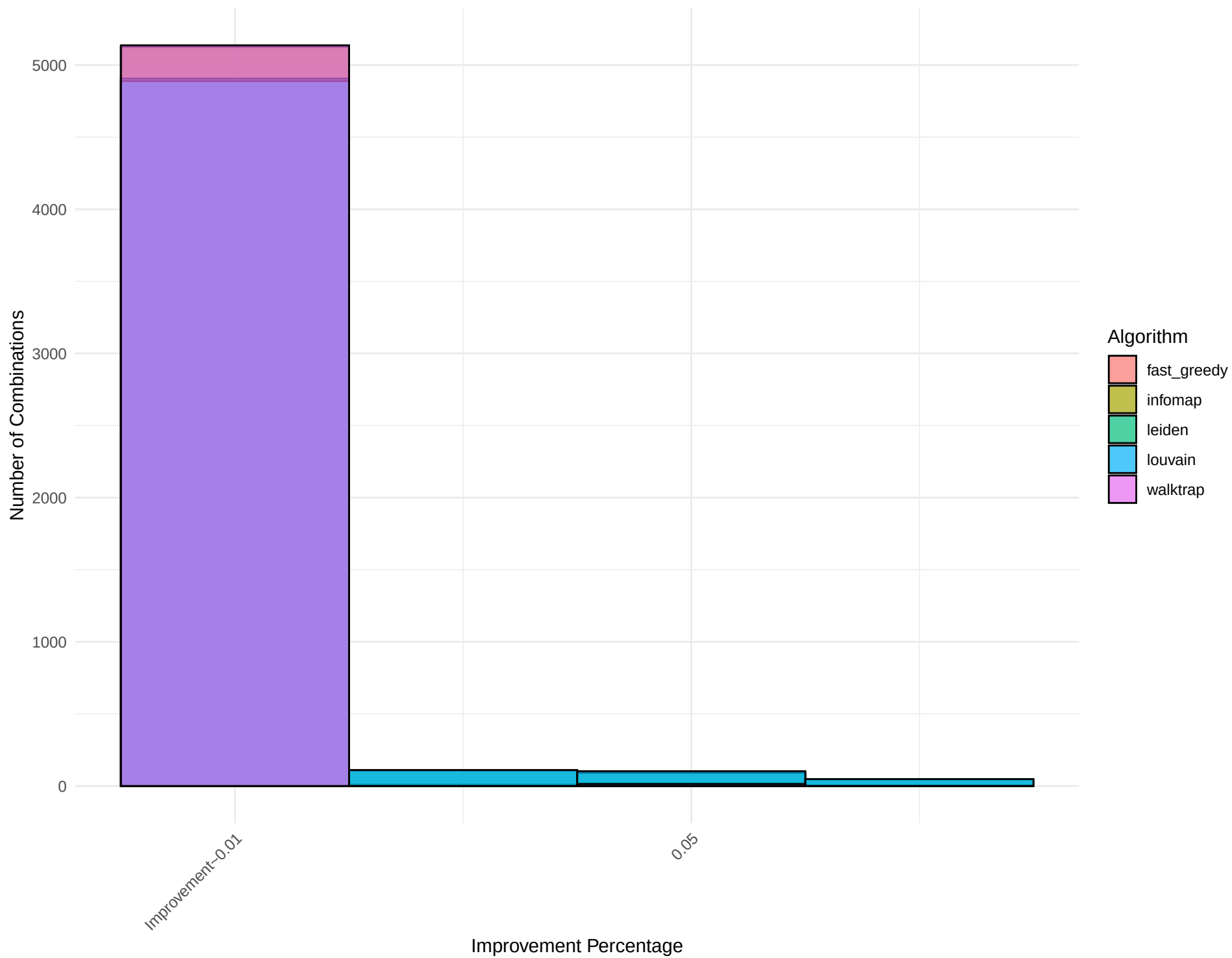
Combined Histogram for Network: hierarchical_graph_7
