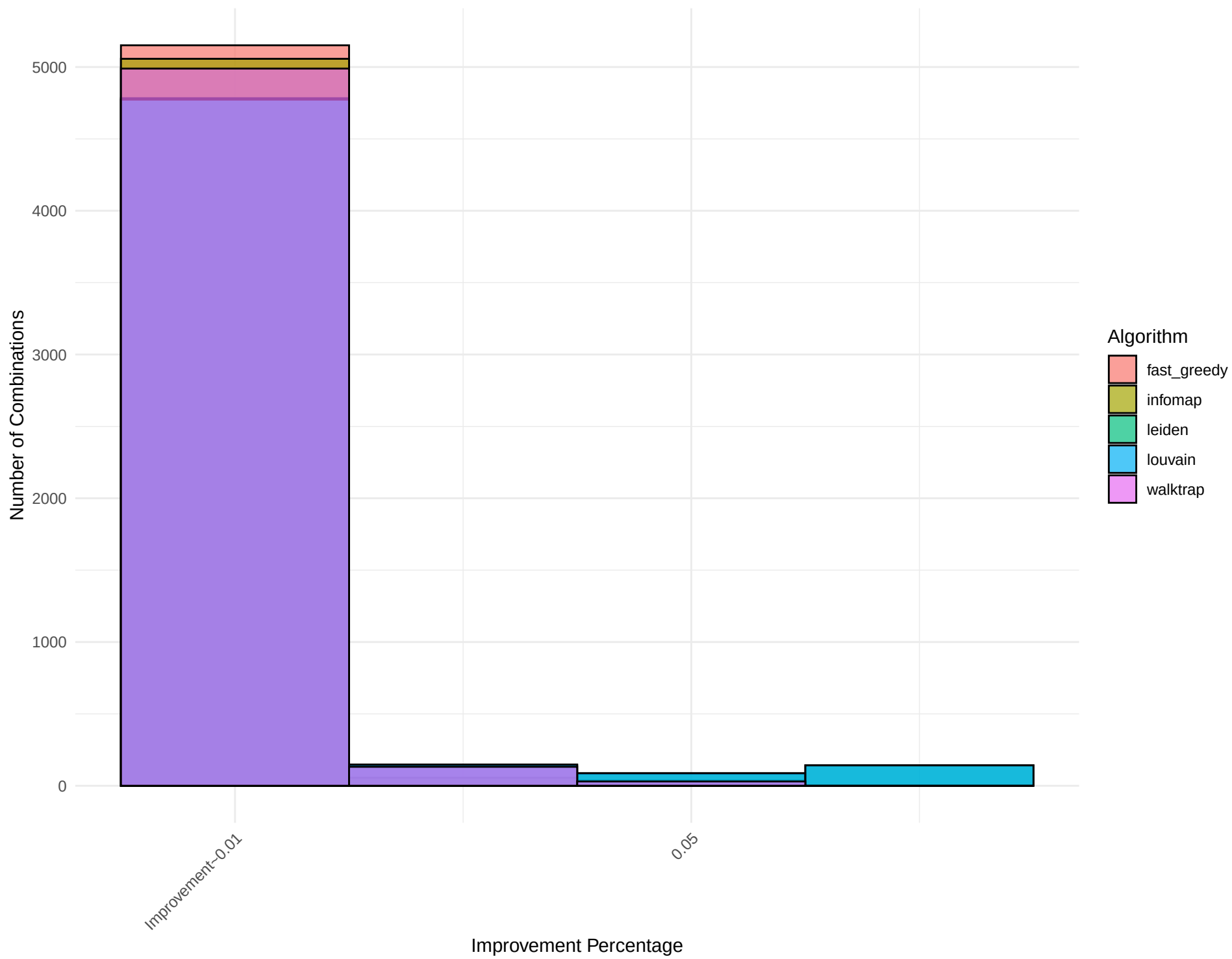
Combined Histogram for Network: edit-mywikibooks
