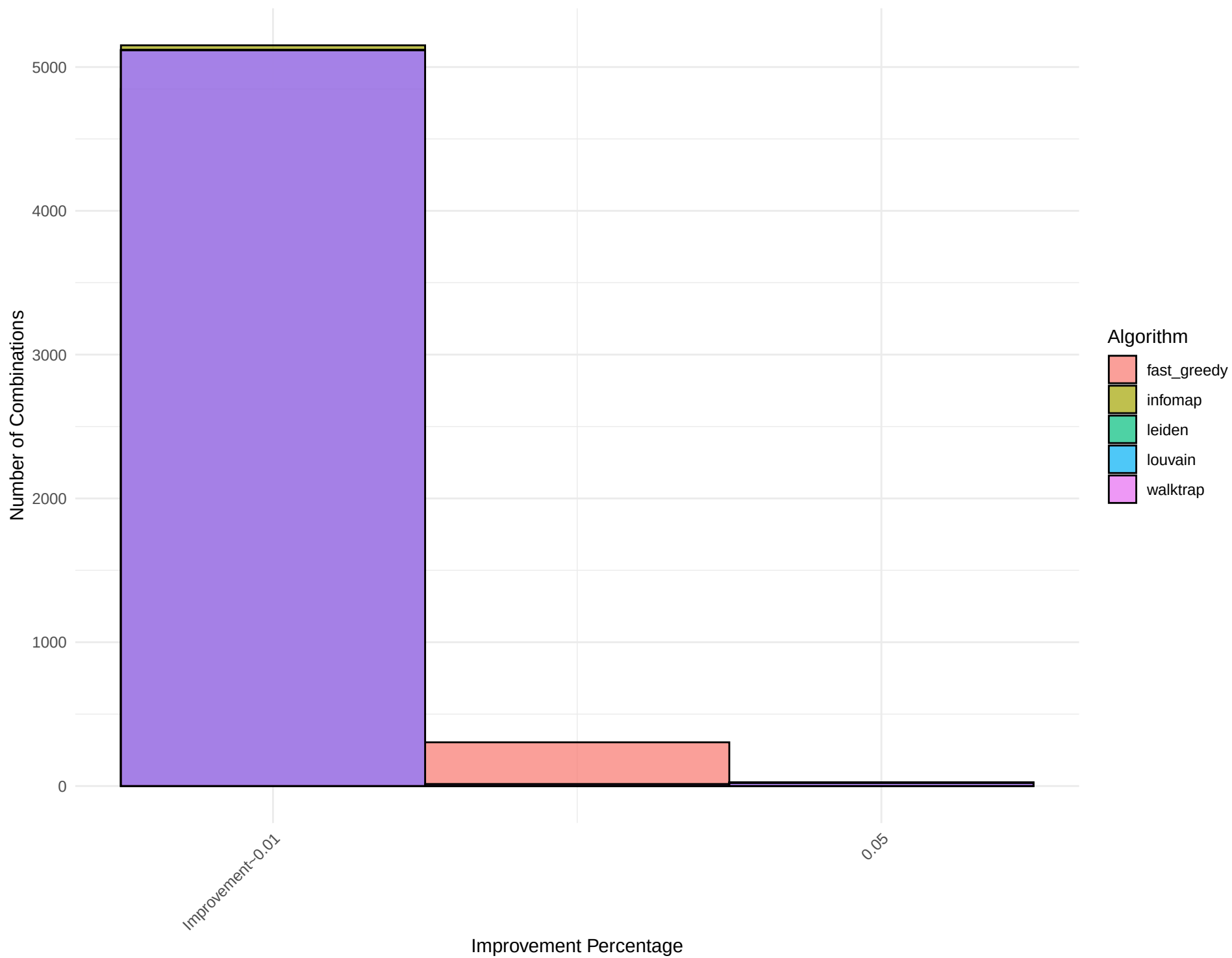
Combined Histogram for Network: edit-sewikibooks
