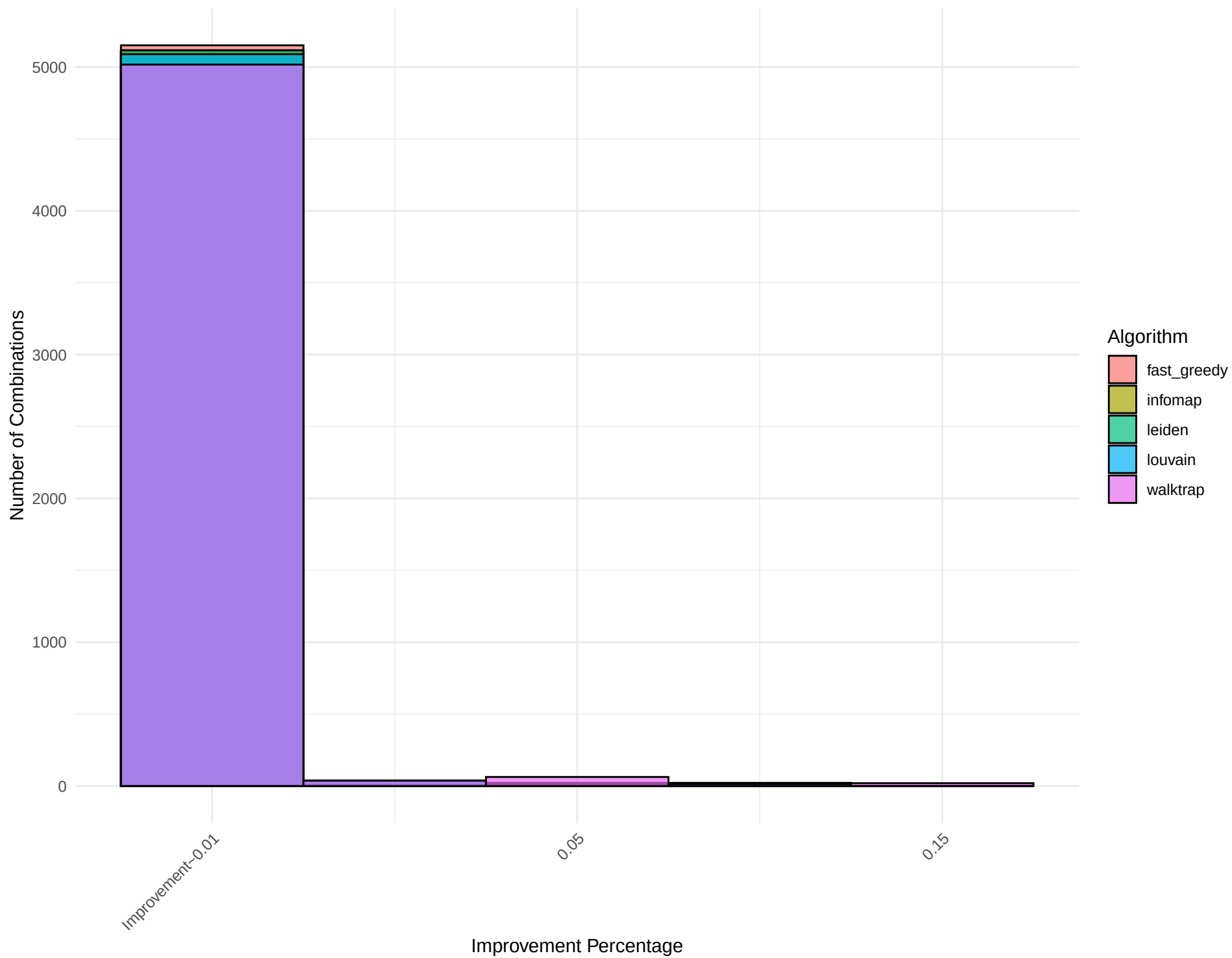
Combined Histogram for Network: edit-aawiktionary
