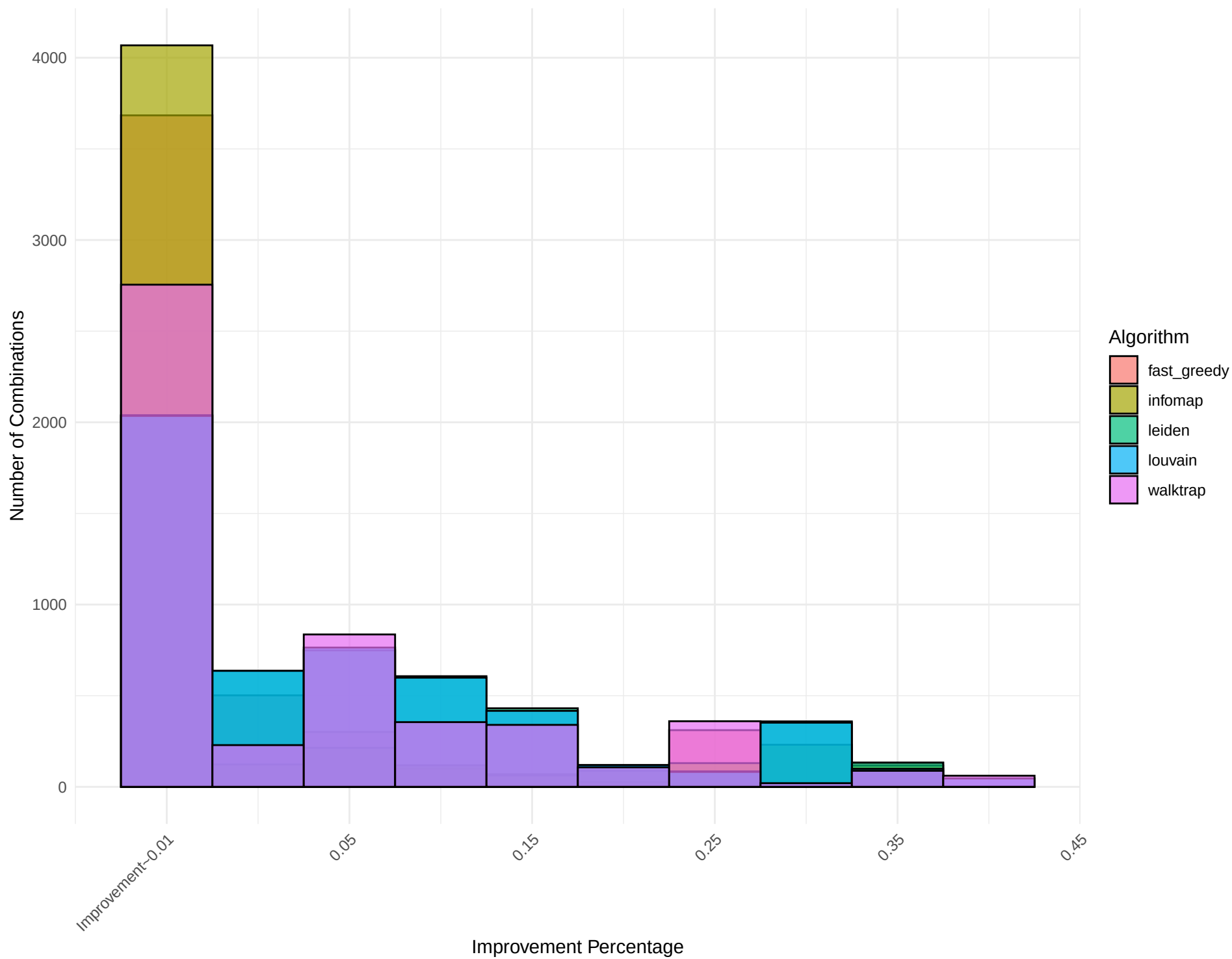
Combined Histogram for Network: small_world_graph_11
