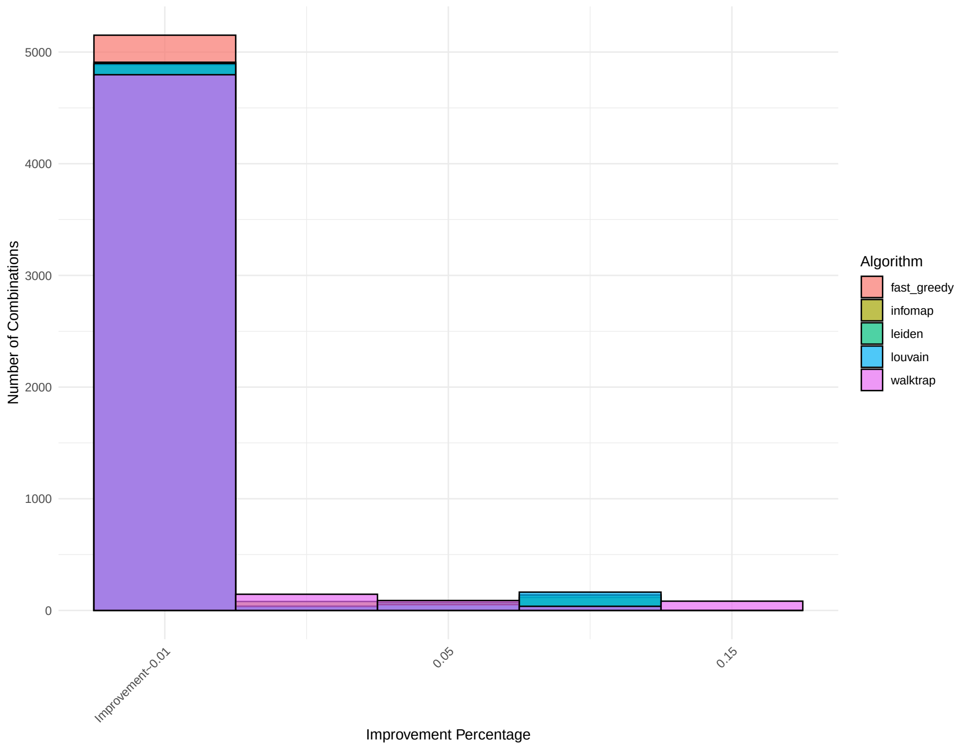
Combined Histogram for Network: edit-pswikibooks
