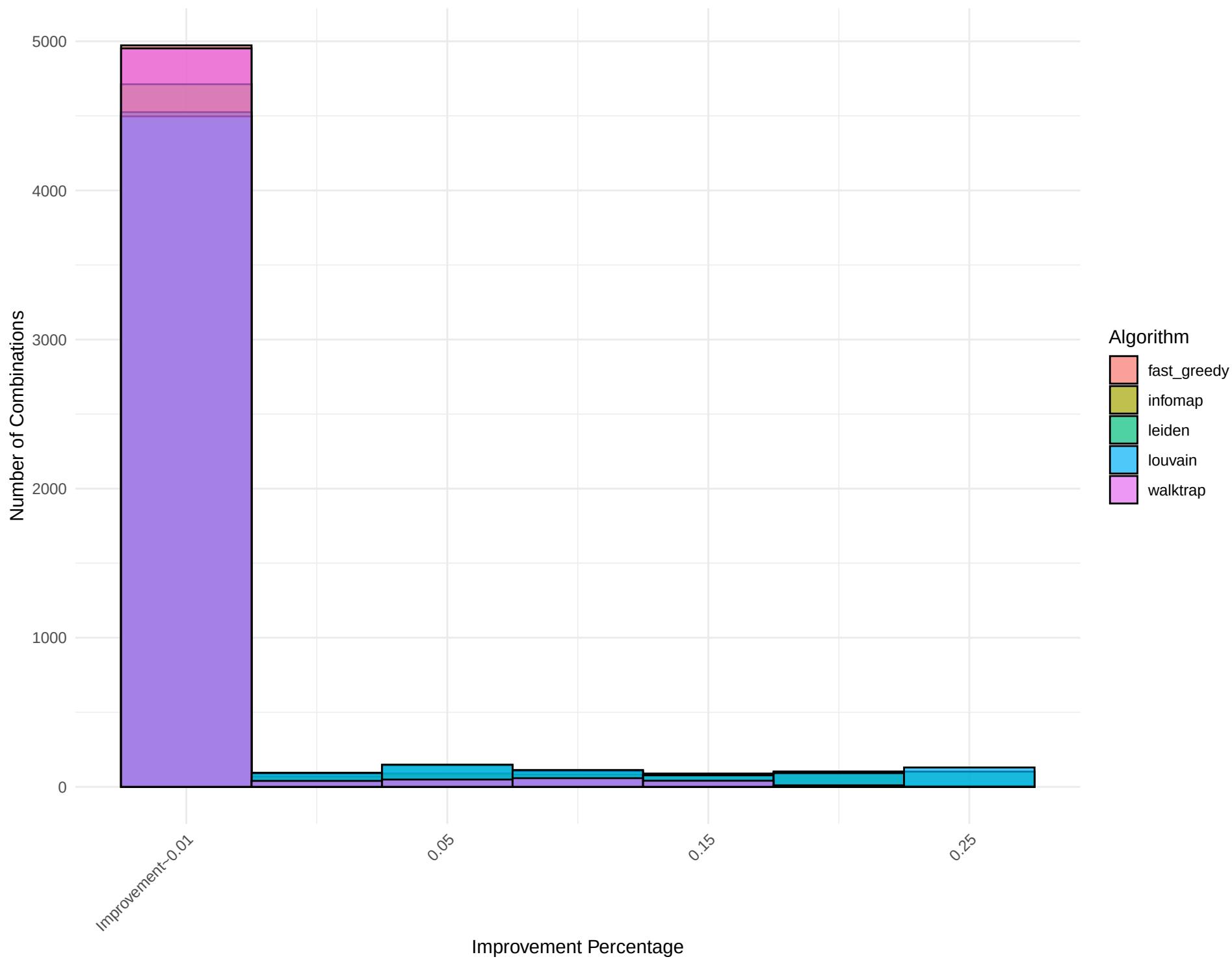
Combined Histogram for Network: barabasi_albert_13
