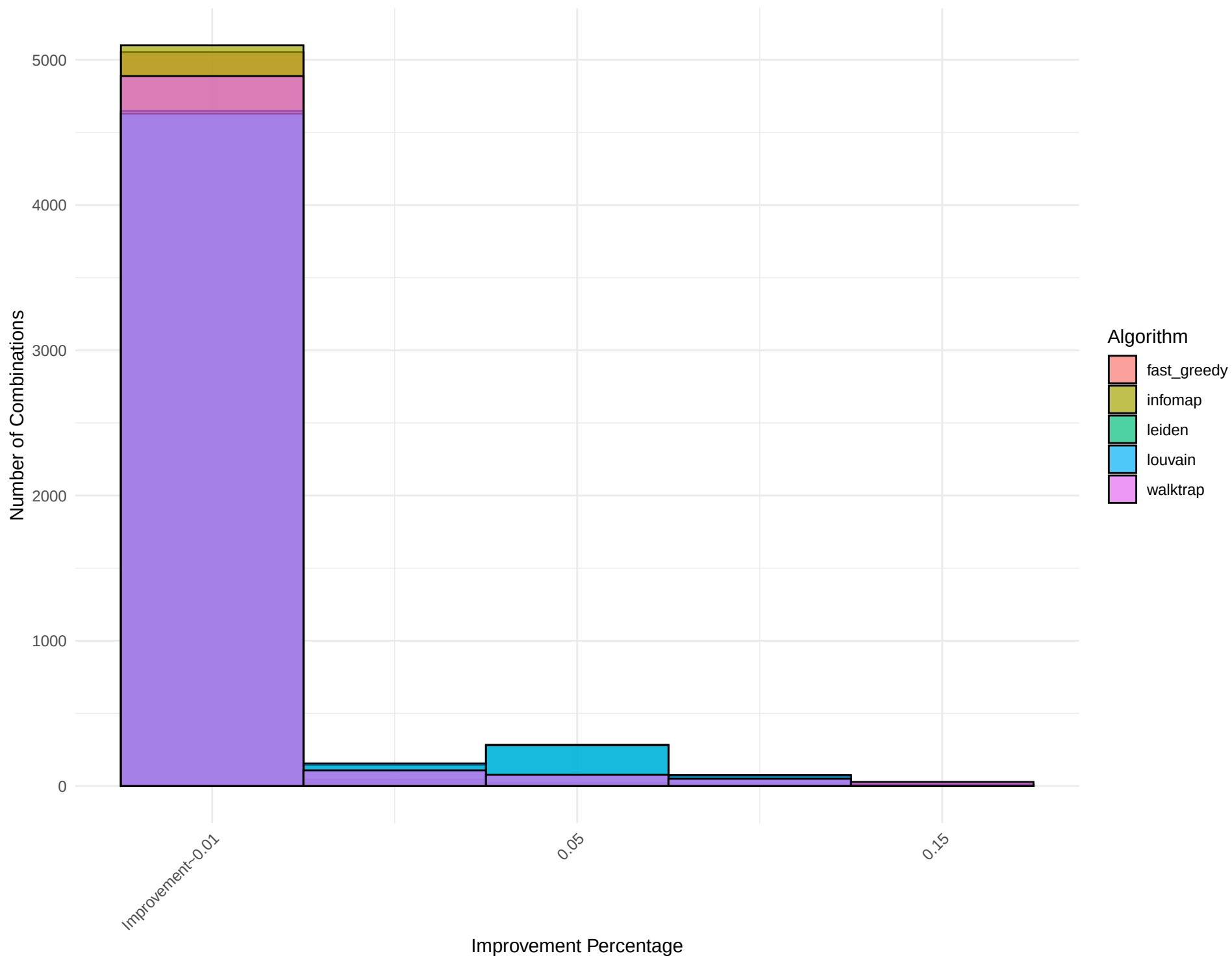
Combined Histogram for Network: dolphins
