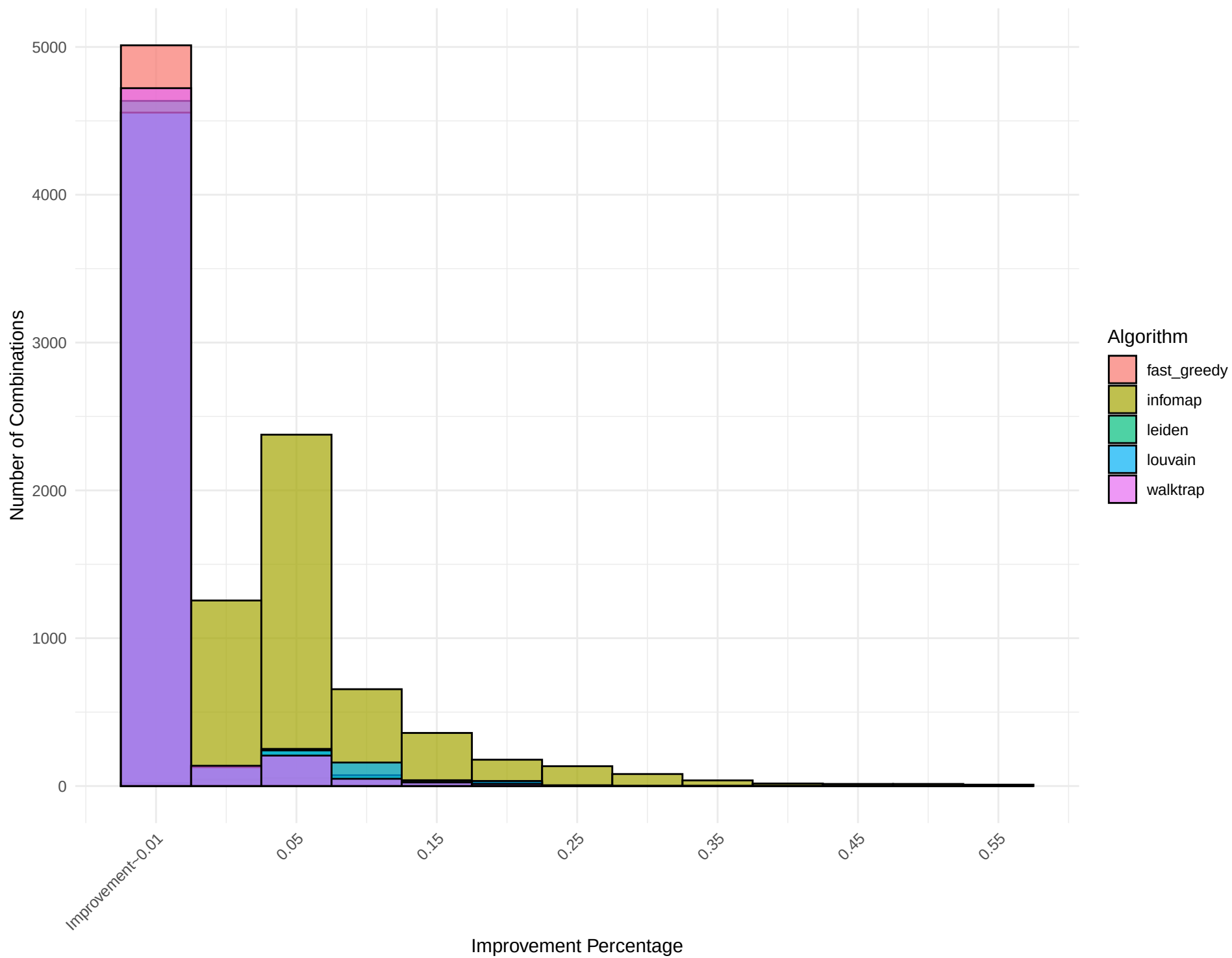
Combined Histogram for Network: hierarchical_graph_17
