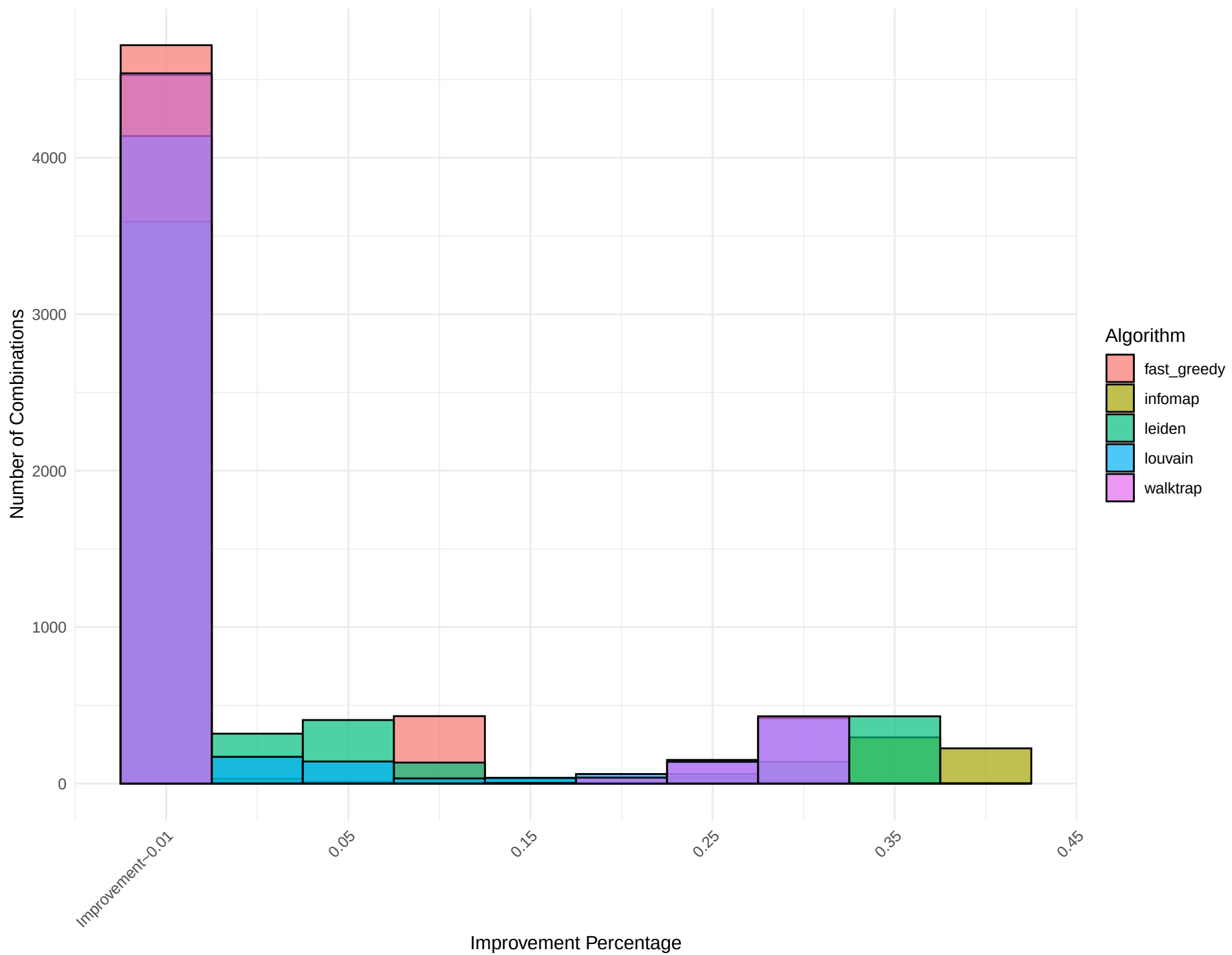
Combined Histogram for Network: brunson_south-africa
