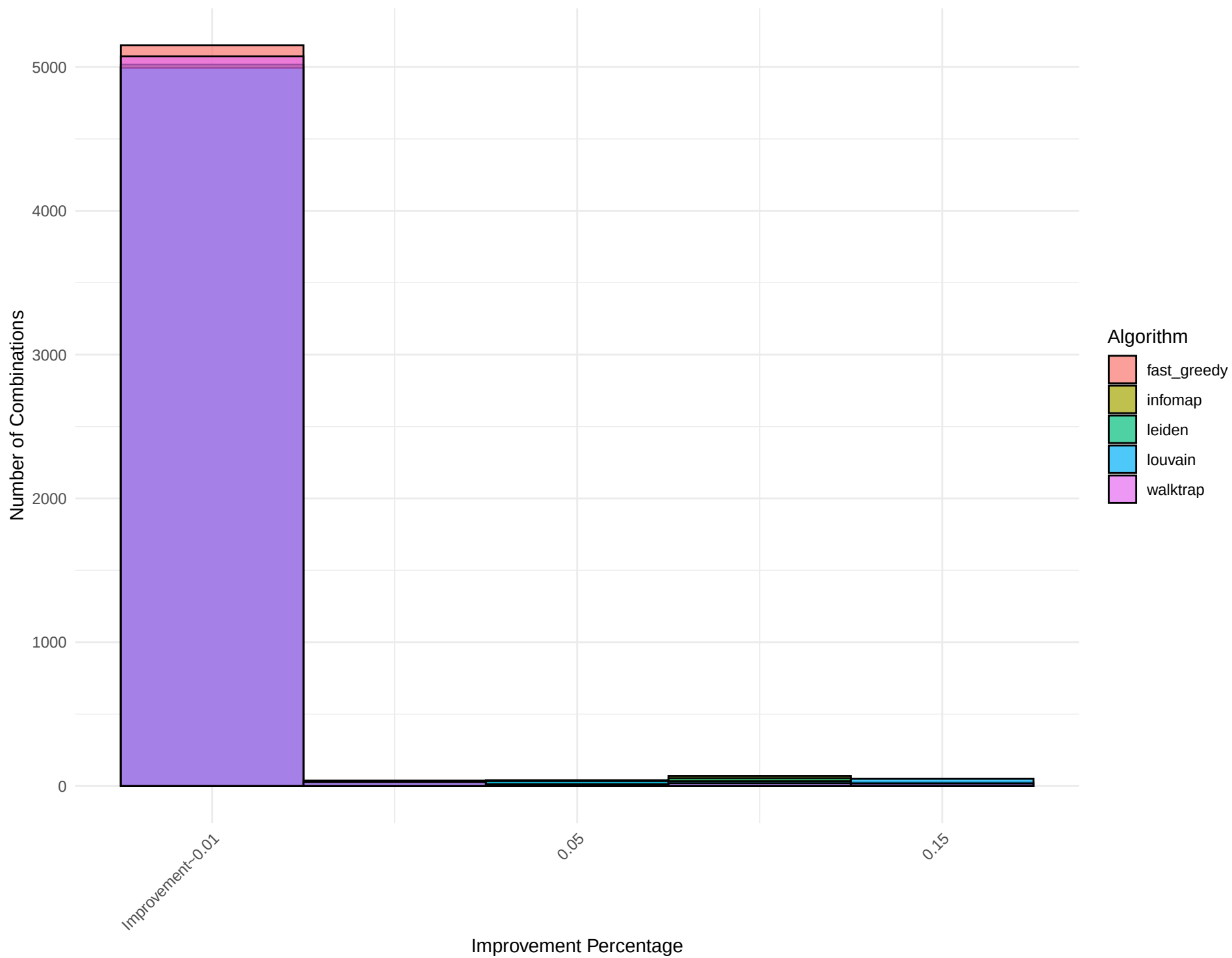
Combined Histogram for Network: edit-ndswikibooks
