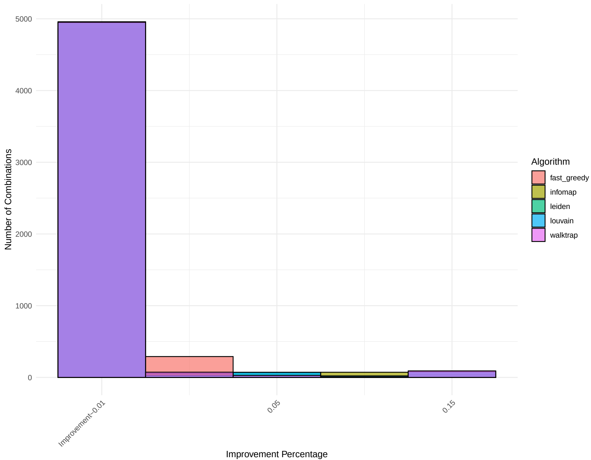
Combined Histogram for Network: edit-lbwikibooks
