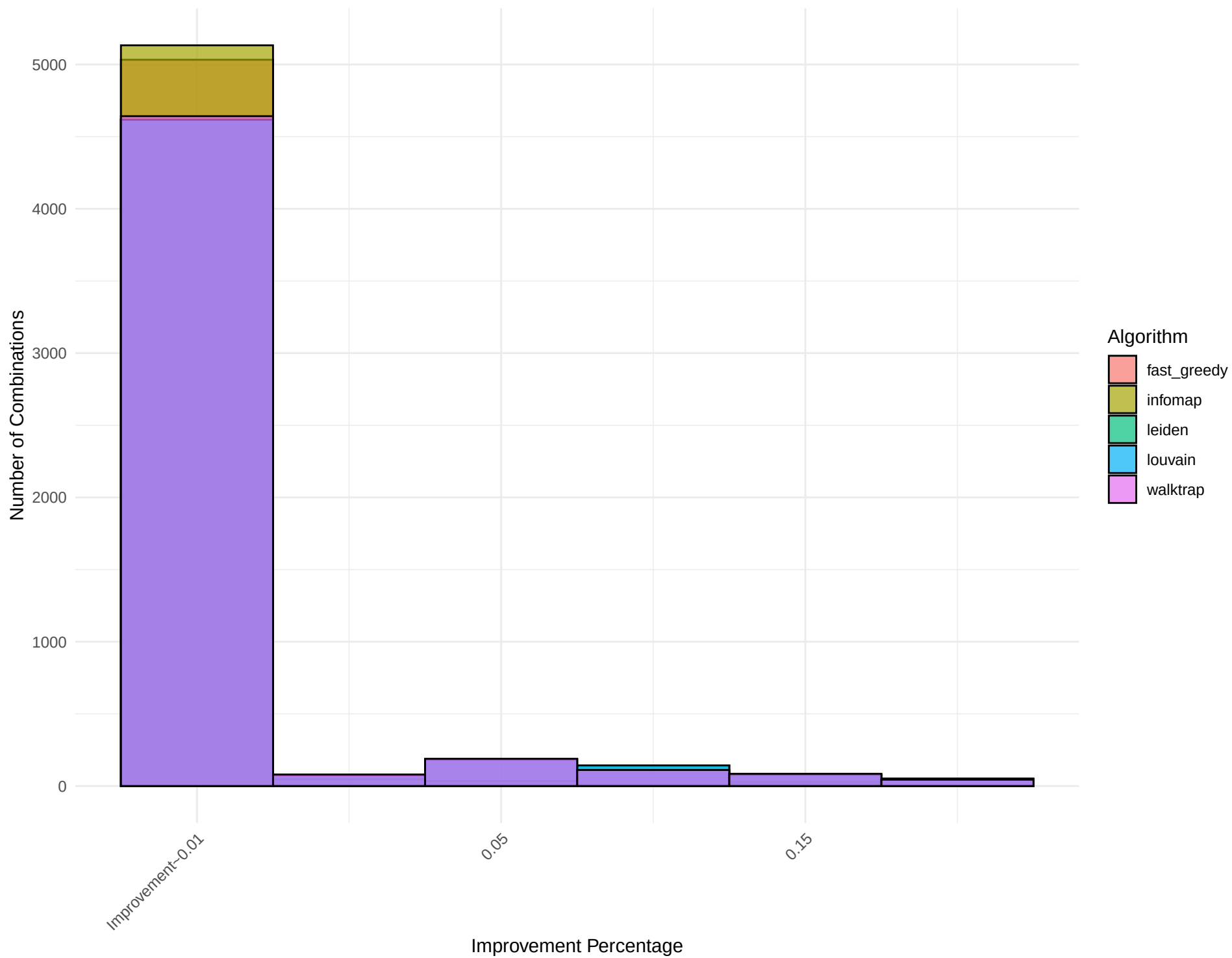
Combined Histogram for Network: dimacs10-football
