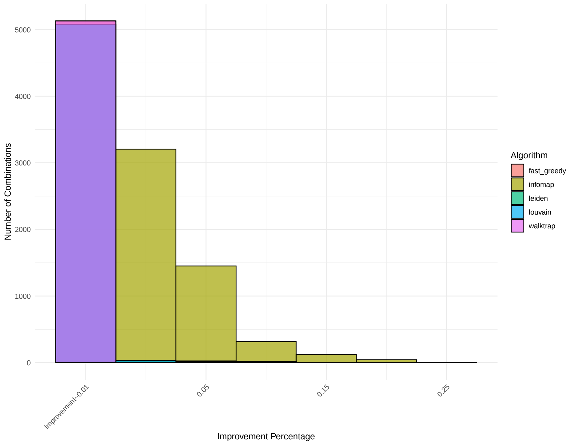
Combined Histogram for Network: barabasi_albert_14
