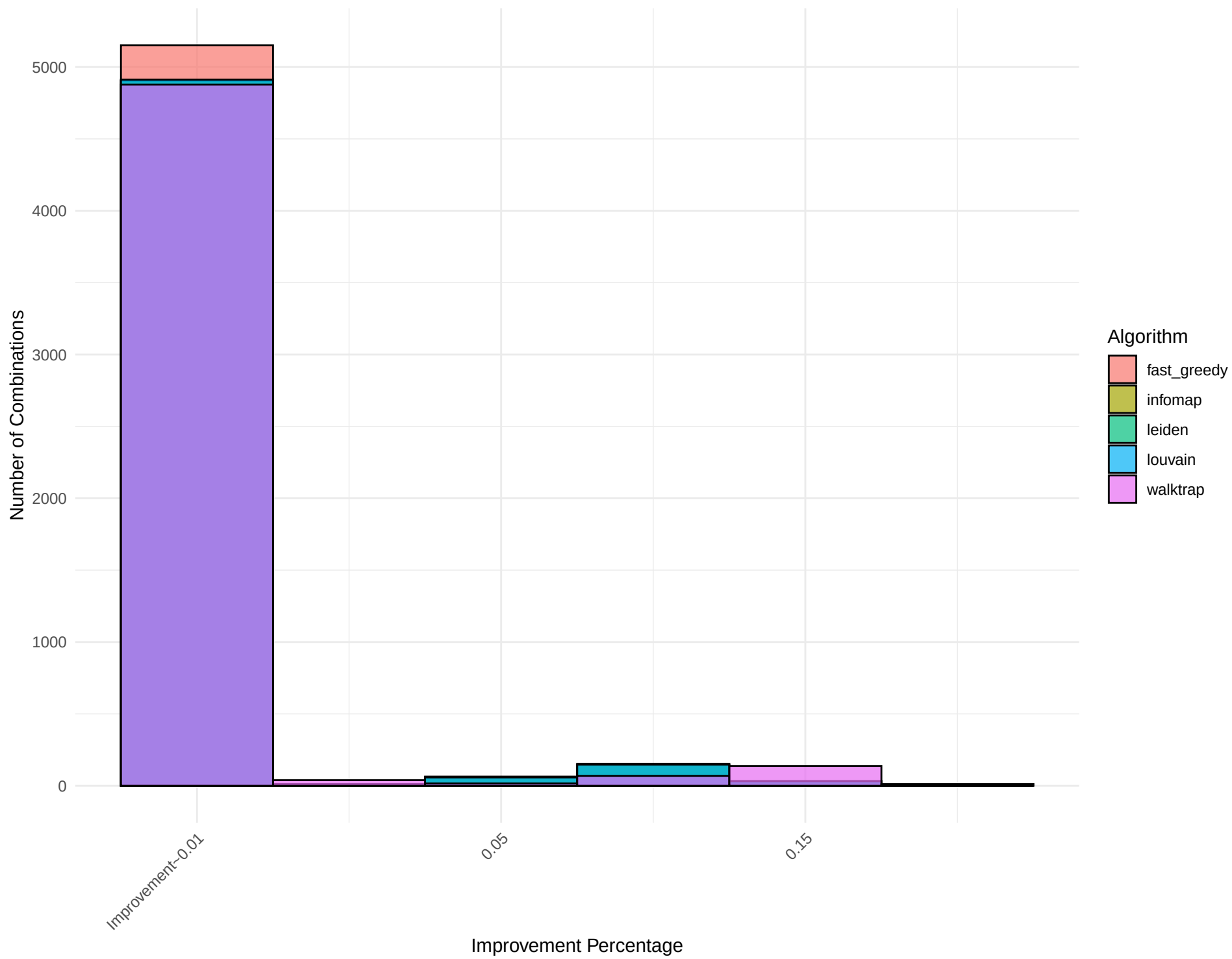
Combined Histogram for Network: edit-kswikibooks
