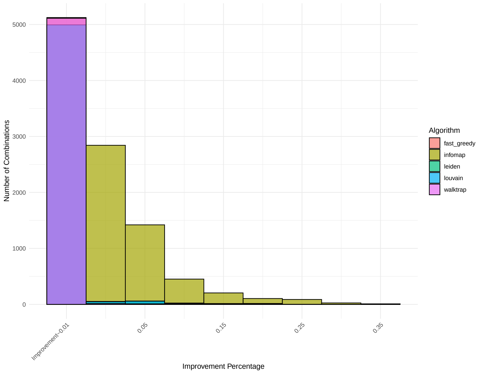
Combined Histogram for Network: barabasi_albert_11
