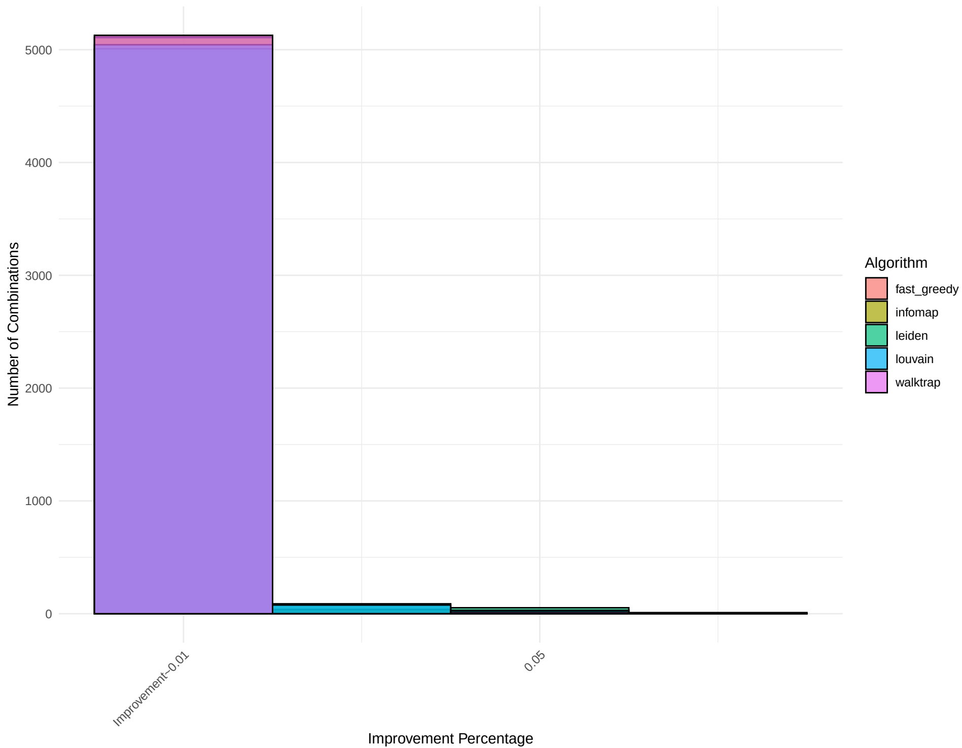
Combined Histogram for Network: hierarchical_graph_20
