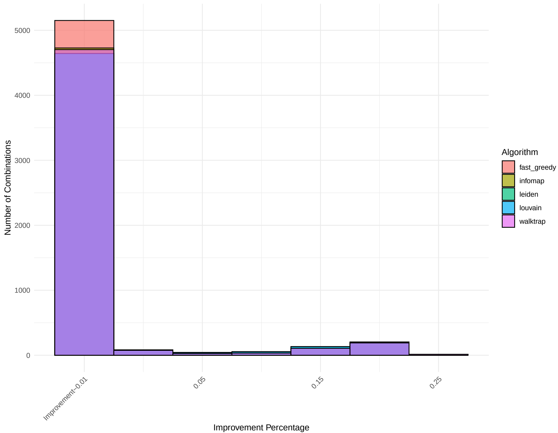
Combined Histogram for Network: barabasi_albert_20
