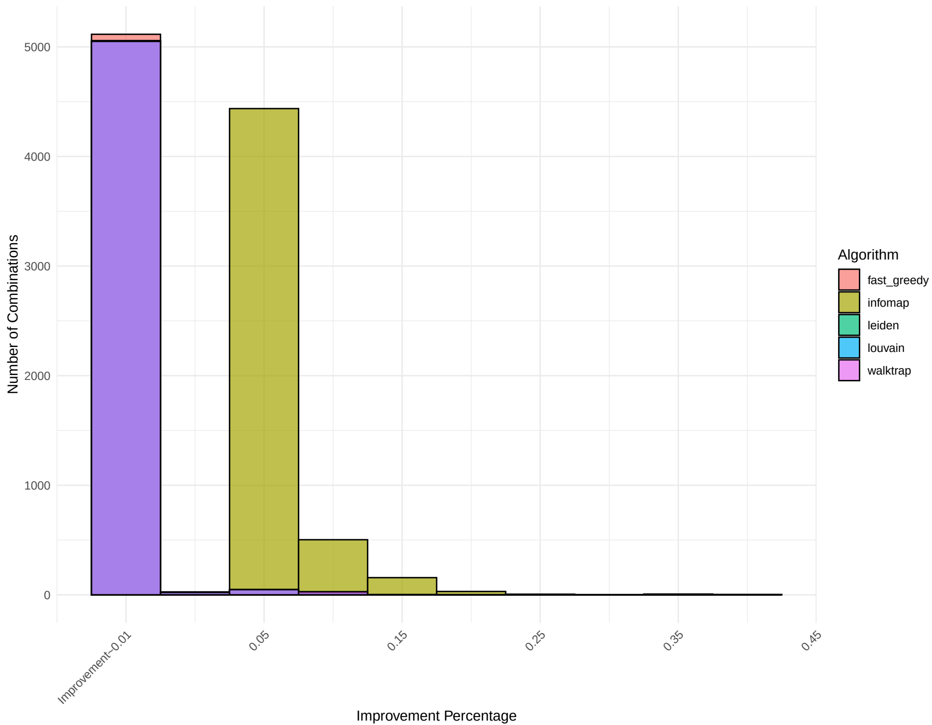
Combined Histogram for Network: small_world_graph_5
