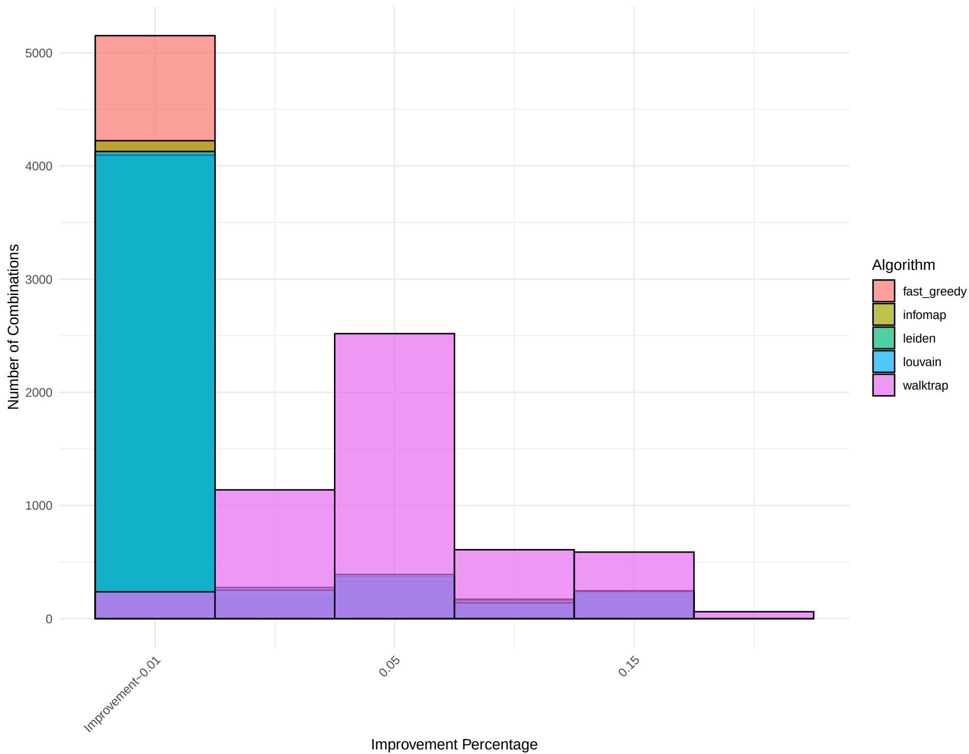
Combined Histogram for Network: edit-akwiktionary
