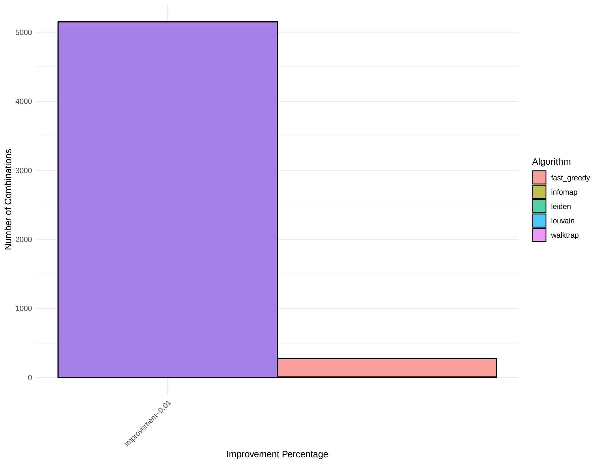
Combined Histogram for Network: edit-rmwiktionary
