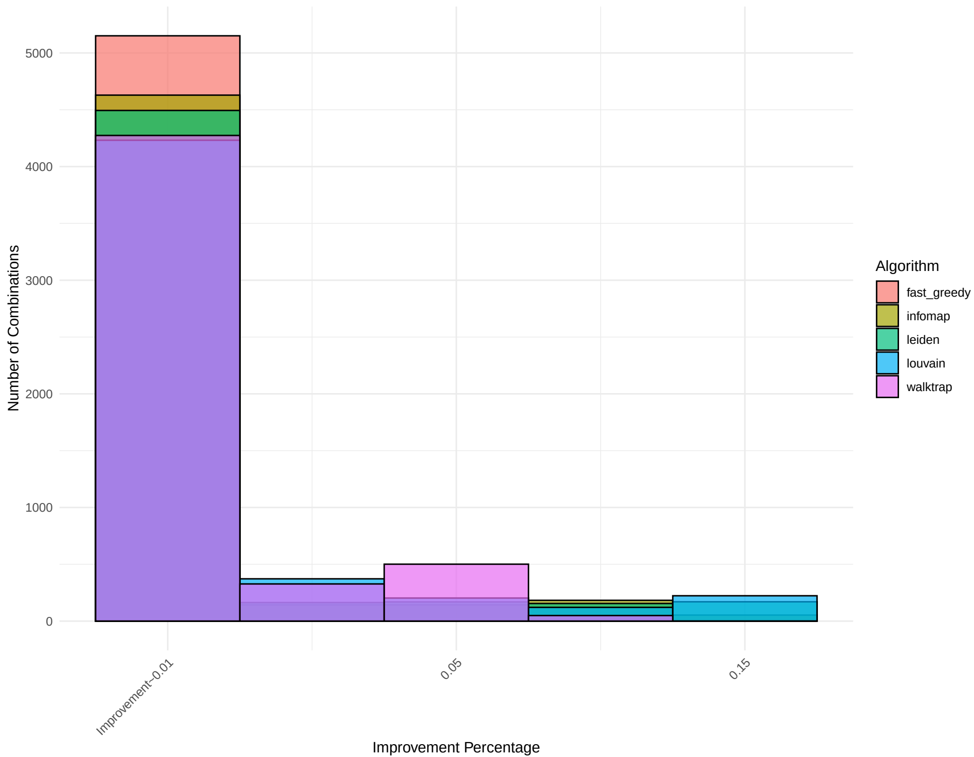
Combined Histogram for Network: edit-awiktionary
