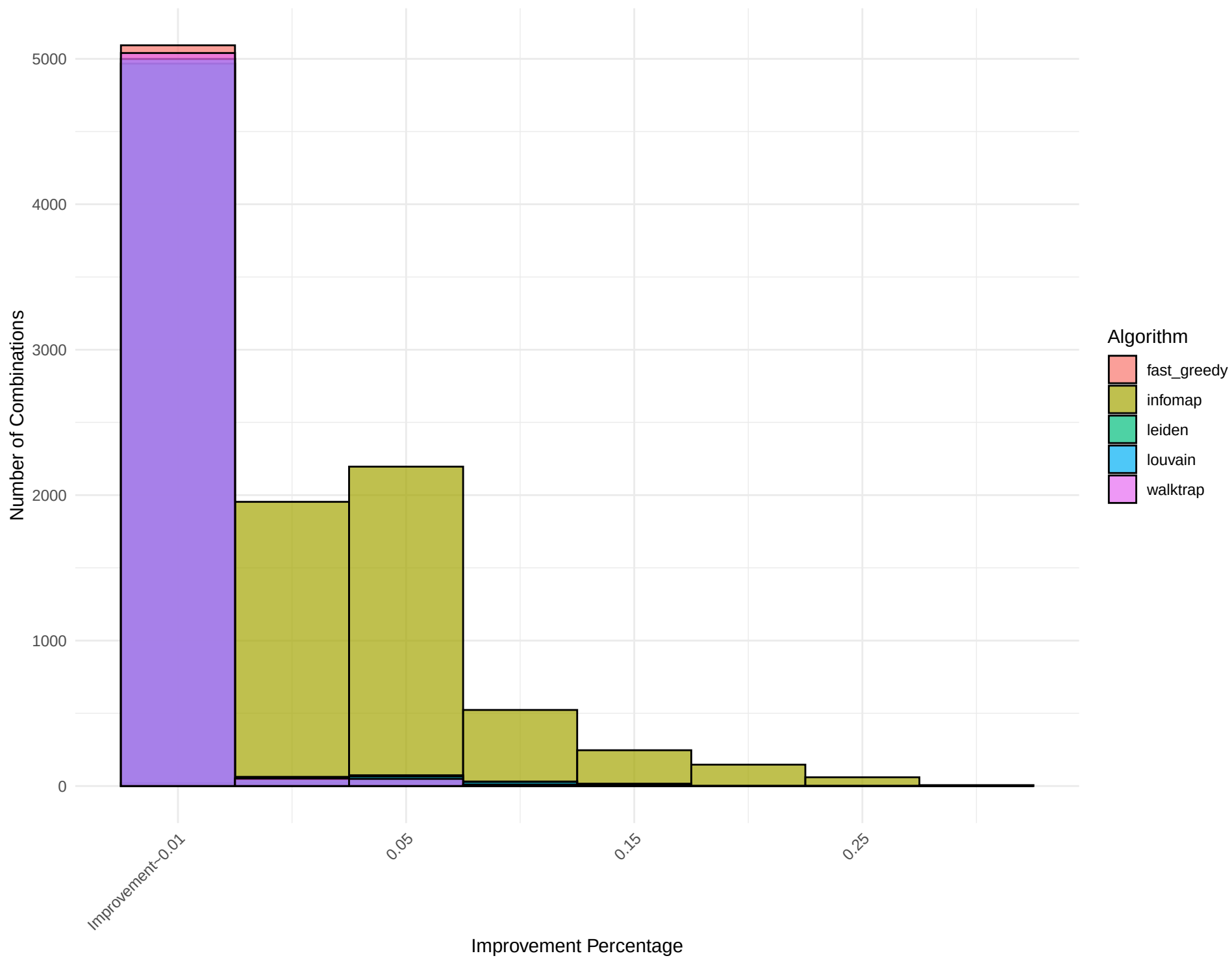
Combined Histogram for Network: hierarchical_graph_8
