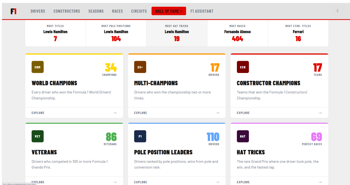
Figure 5: Hall of Fame dashboard ( /hall-of-fame/ ). All six counts (World Champions, Multi-Champions, Constructor Champions, Veterans, Pole Leaders, Hat Tricks) are queried live from SPIN-inferred graph properties.
