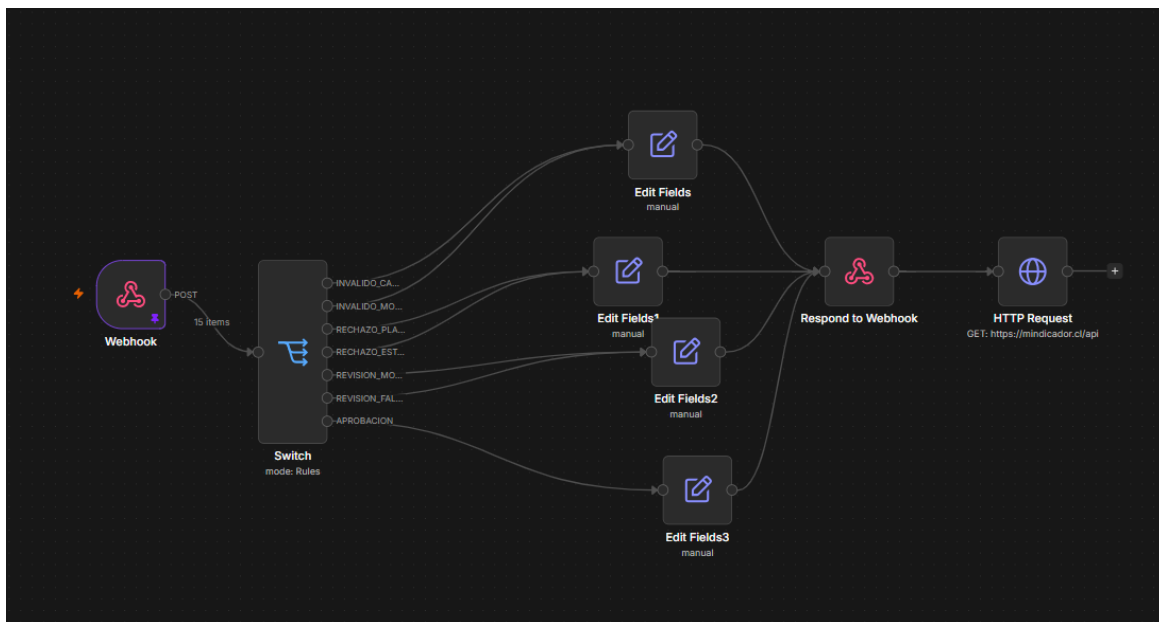
WorkFlow n8n
