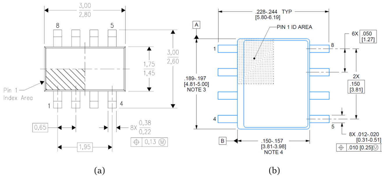
Figura 2: (a) DCN Package SOT-23 and (b) D Package SOIC
