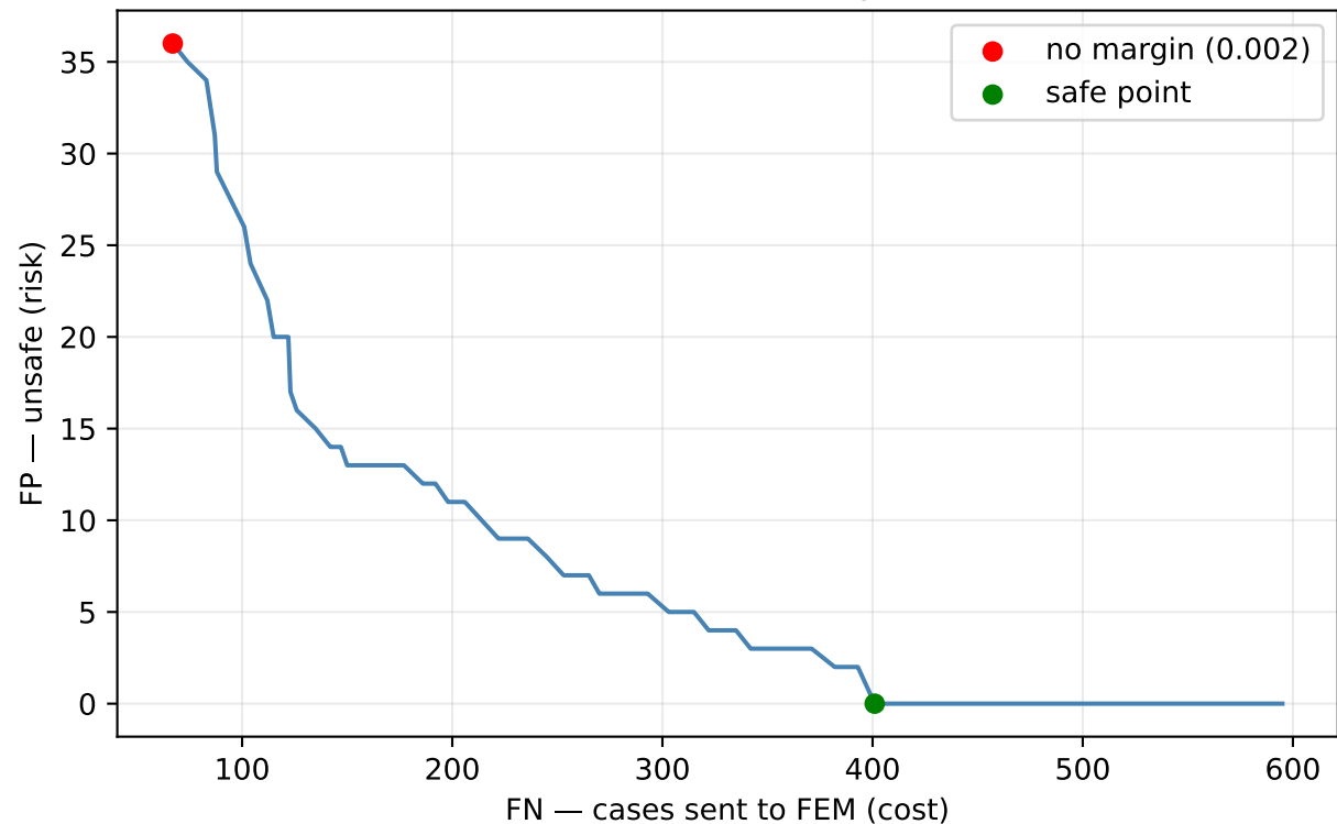
Risk-cost curve (safety ROC)
