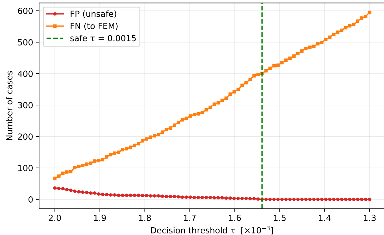
FP and FN vs safety margin
