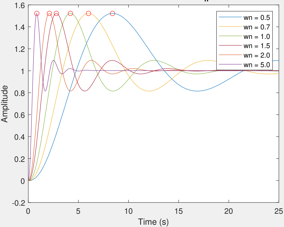
Time scaling property of \omega_n
