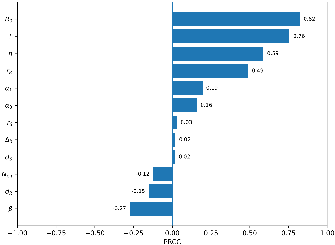
Output-specific PRCC ranking for A_R
