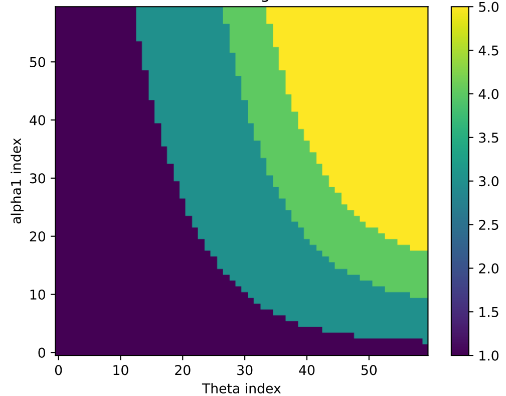
60x60: regime
