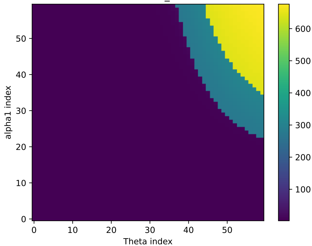
60x60: A_u
