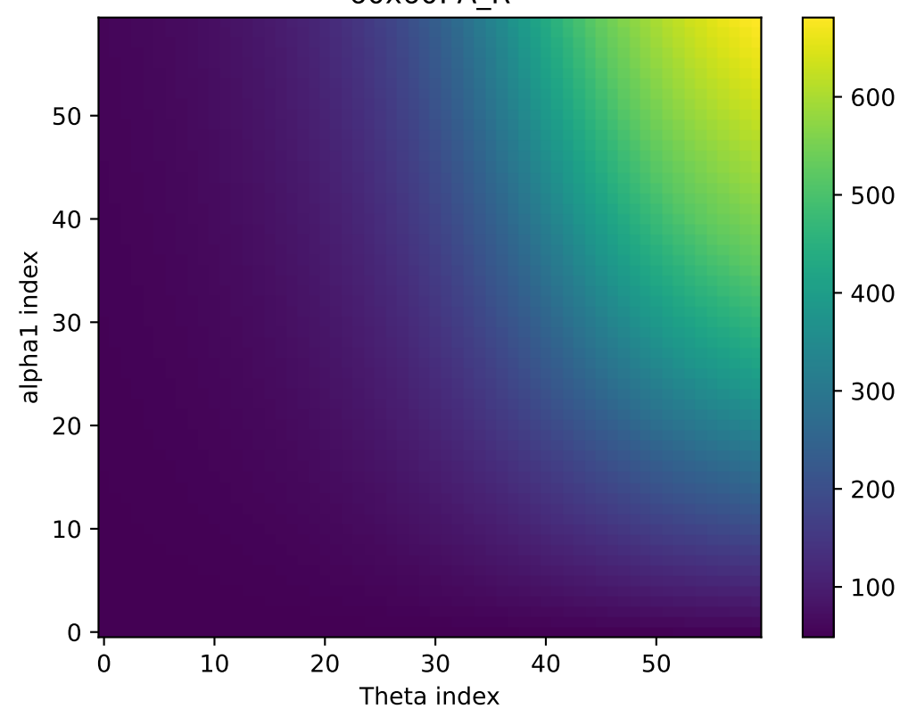
60x60: regime
