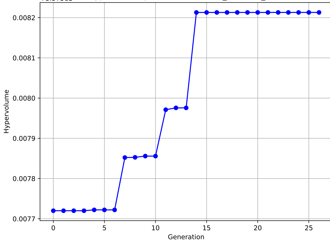
+3.573e1 Hypervolume per evaluations (std_loss, adv_loss)
