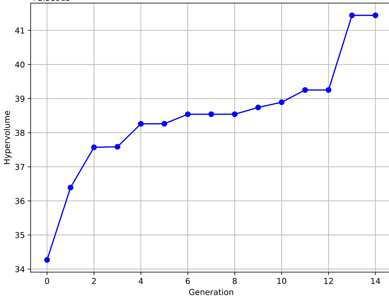
Hypervolume per evaluations (std_loss, adv_loss, flops, n_params) +1.319e5
