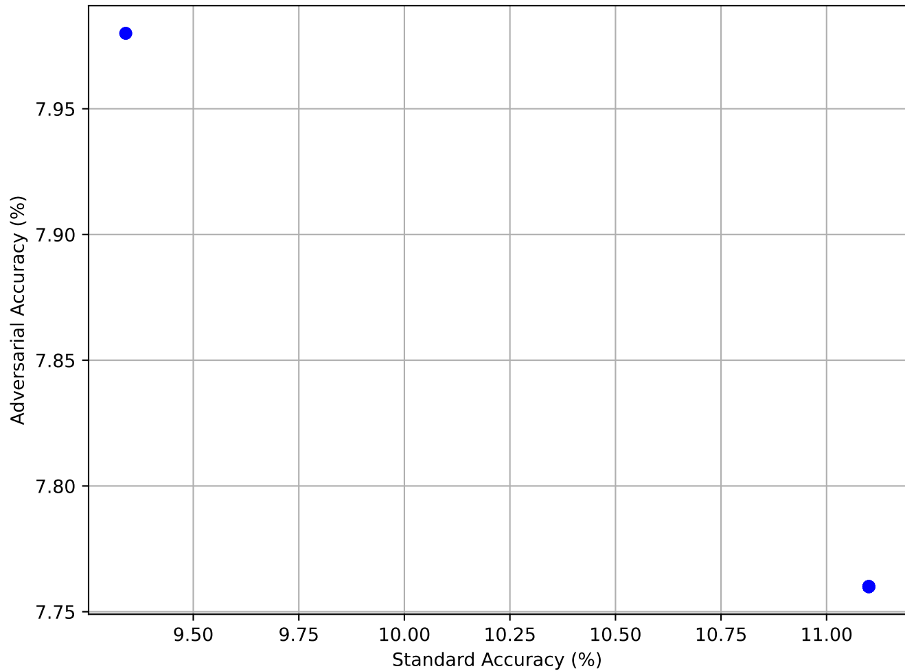
Archive Accuracy
