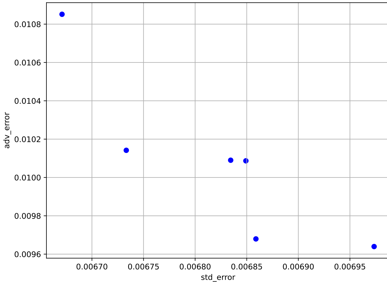
Non-dominated solutions
