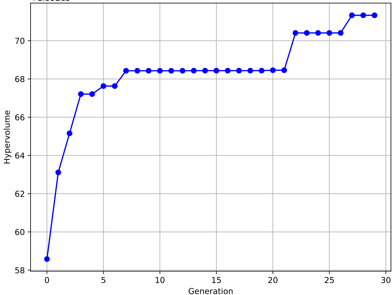
Hypervolume per evaluations (std_loss, adv_loss, flops, n_params) +1.352e5
