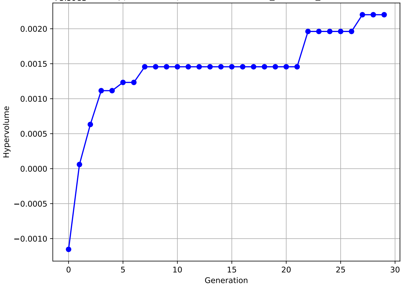
+3.59e1 Hypervolume per evaluations (std_loss, adv_loss)
