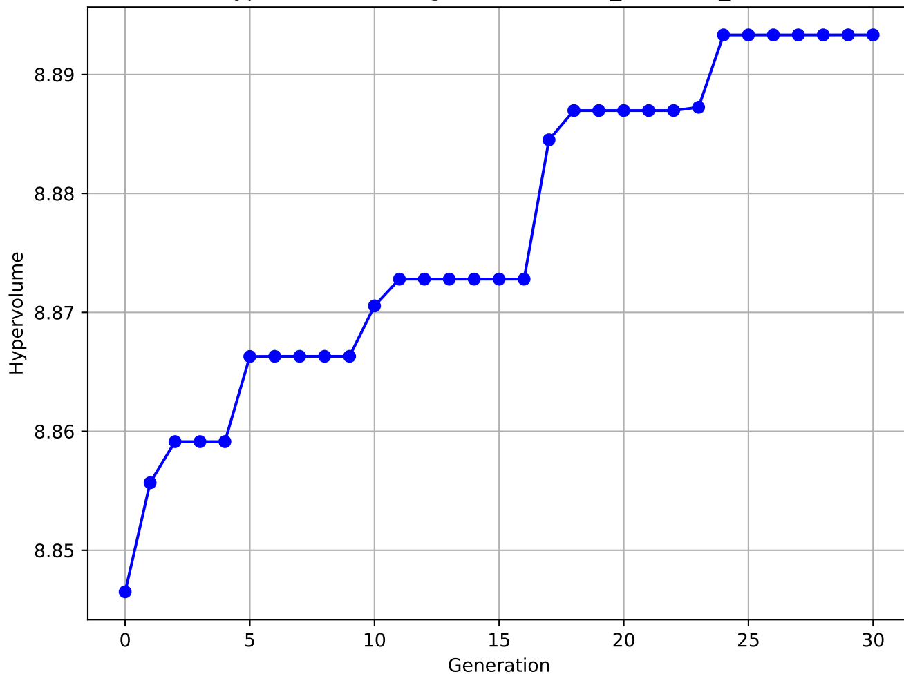
Hypervolume over generations (std_loss, adv_loss)
