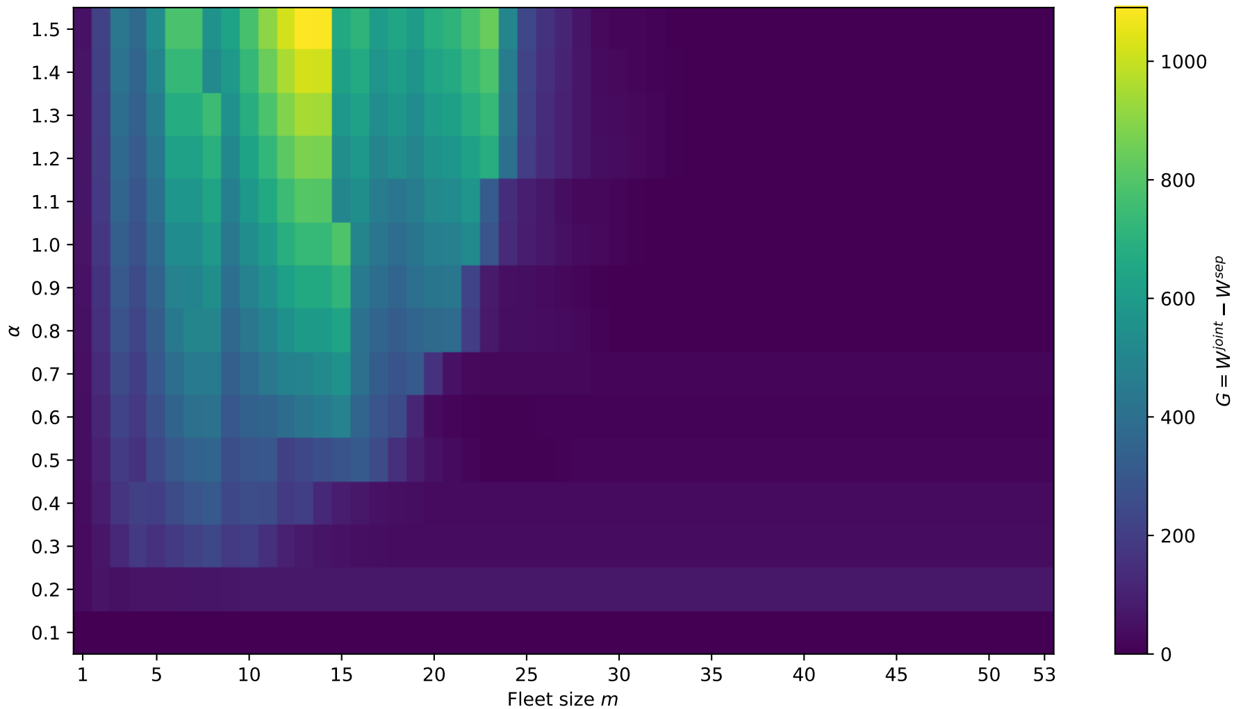
Absolute anticipative gap: G(m, \alpha)
