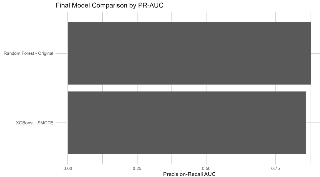
Figure 4.7: Final model comparison by Precision-Recall AUC.
