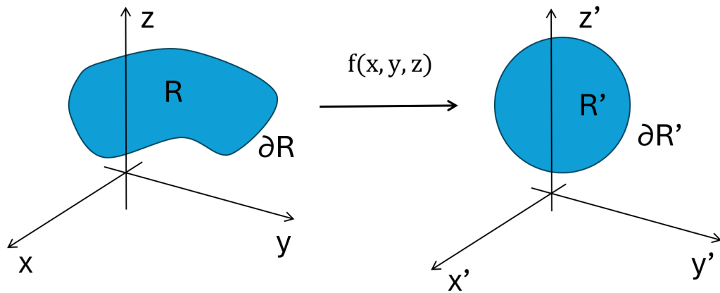
Figure 12.1: Schematic representation of a conformal transformation f(x, y, z) mapping a region R with boundary \partial R in the (x, y, z) coordinate system into a transformed region R' with boundary \partial R' in the (x', y', z') coordinate system.
