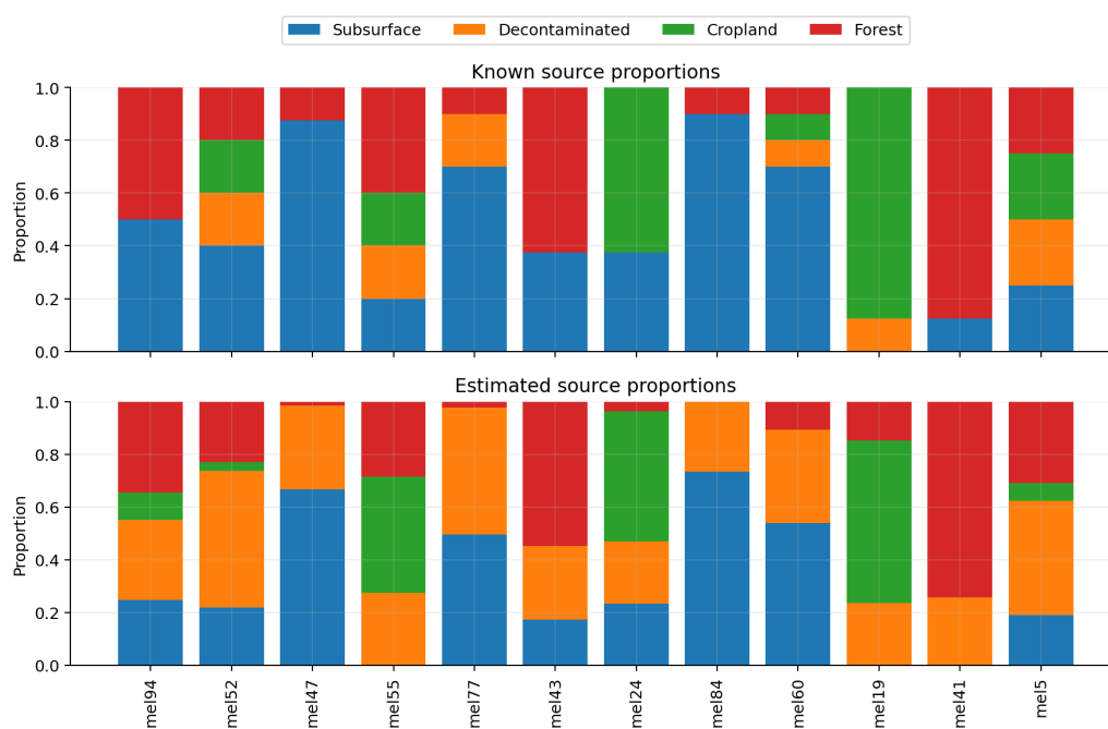
Figure 11.6: Known and reconstructed representative source compositions obtained with the McCaffrey constrained least-squares model.
