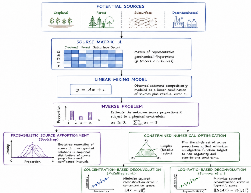
Figure 11.10: Conceptual framework of the source apportionment problem. All three methods considered in this chapter solve the same inverse mixing problem under identical physical constraints, differing only in how uncertainty is represented and how the objective function is formulated.
