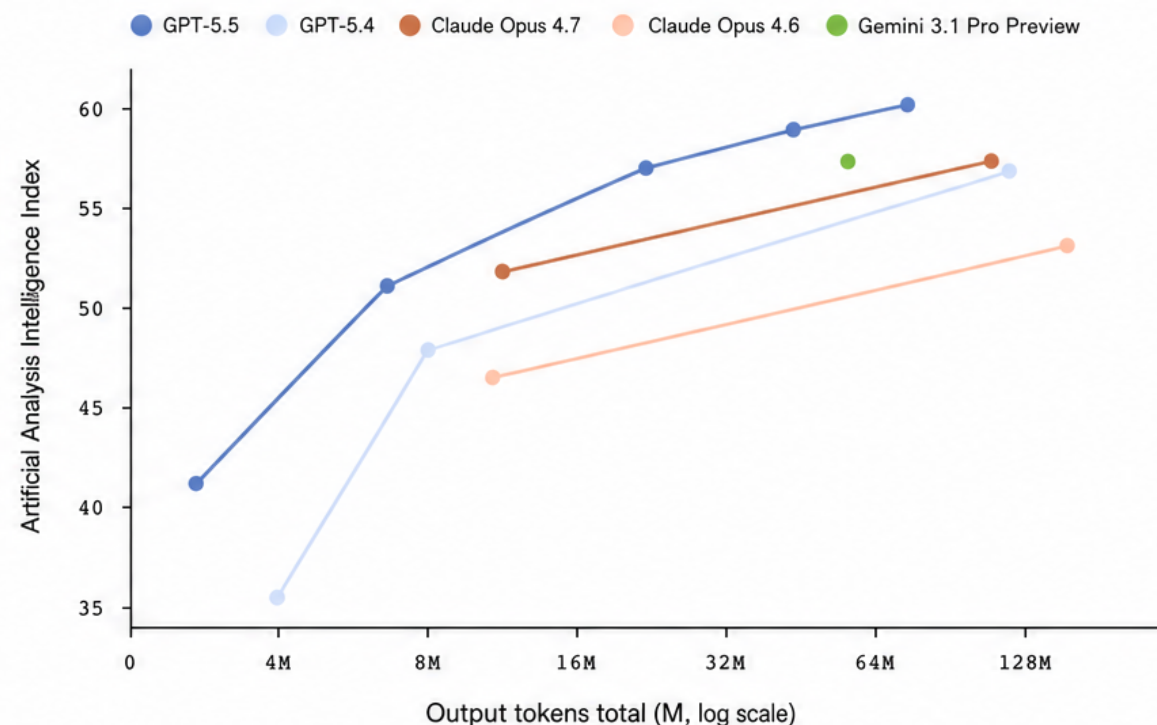
Artificial Analysis Intelligence Index
