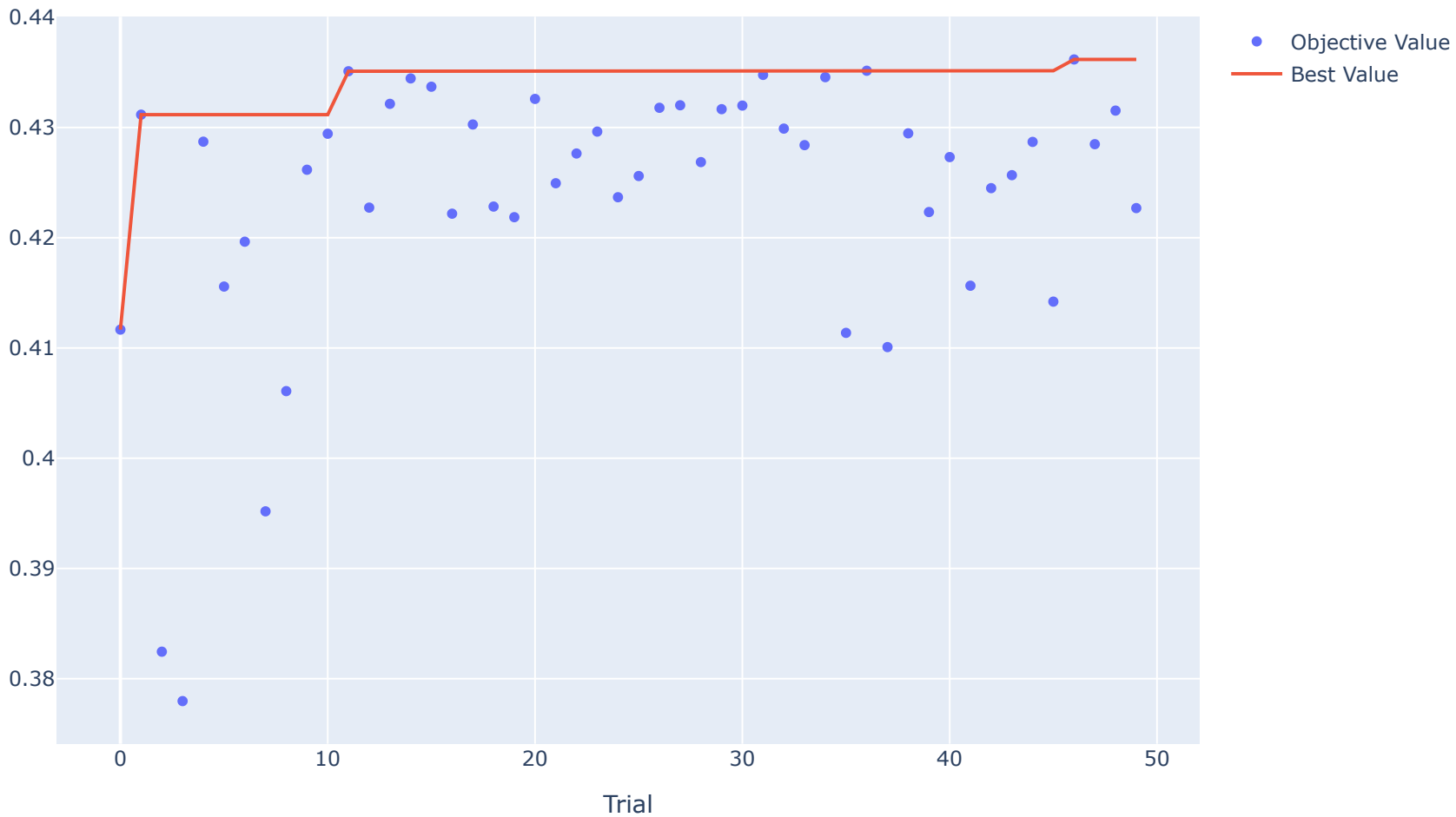
Objective Value
