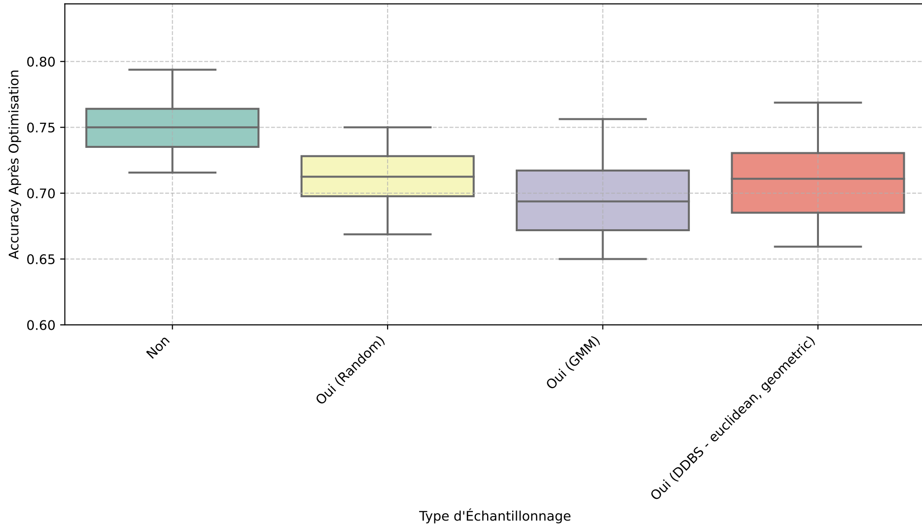
Boxplot - resultats_Decision Tree_preprocessed_winequality_dataset
