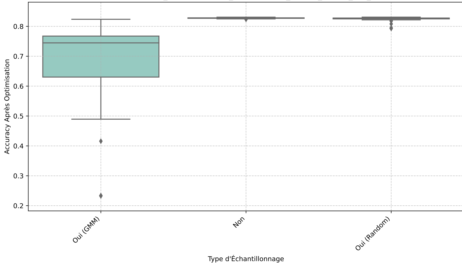
Boxplot - resultats_Neural Network_preprocessed_thyroid_cancer_risk_dataset
