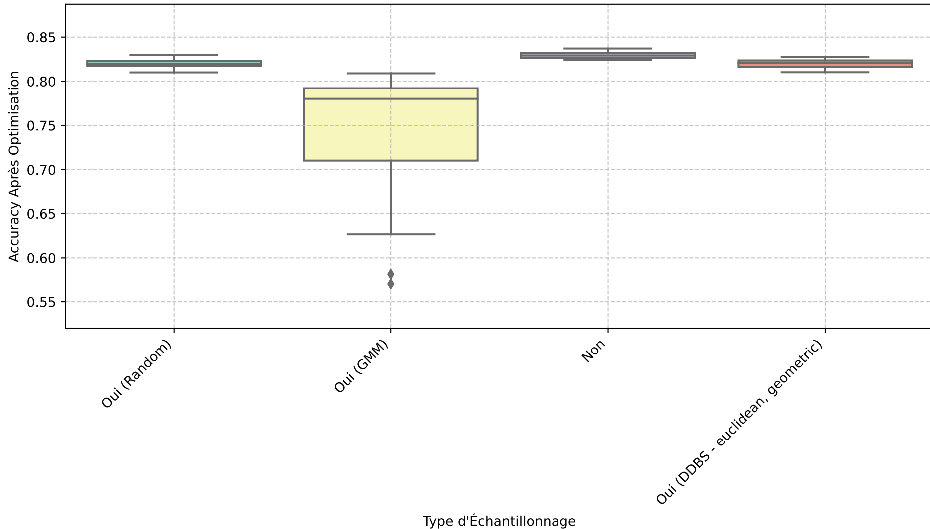
Boxplot - resultats_Decision Tree_preprocessed_student_depression_dataset
