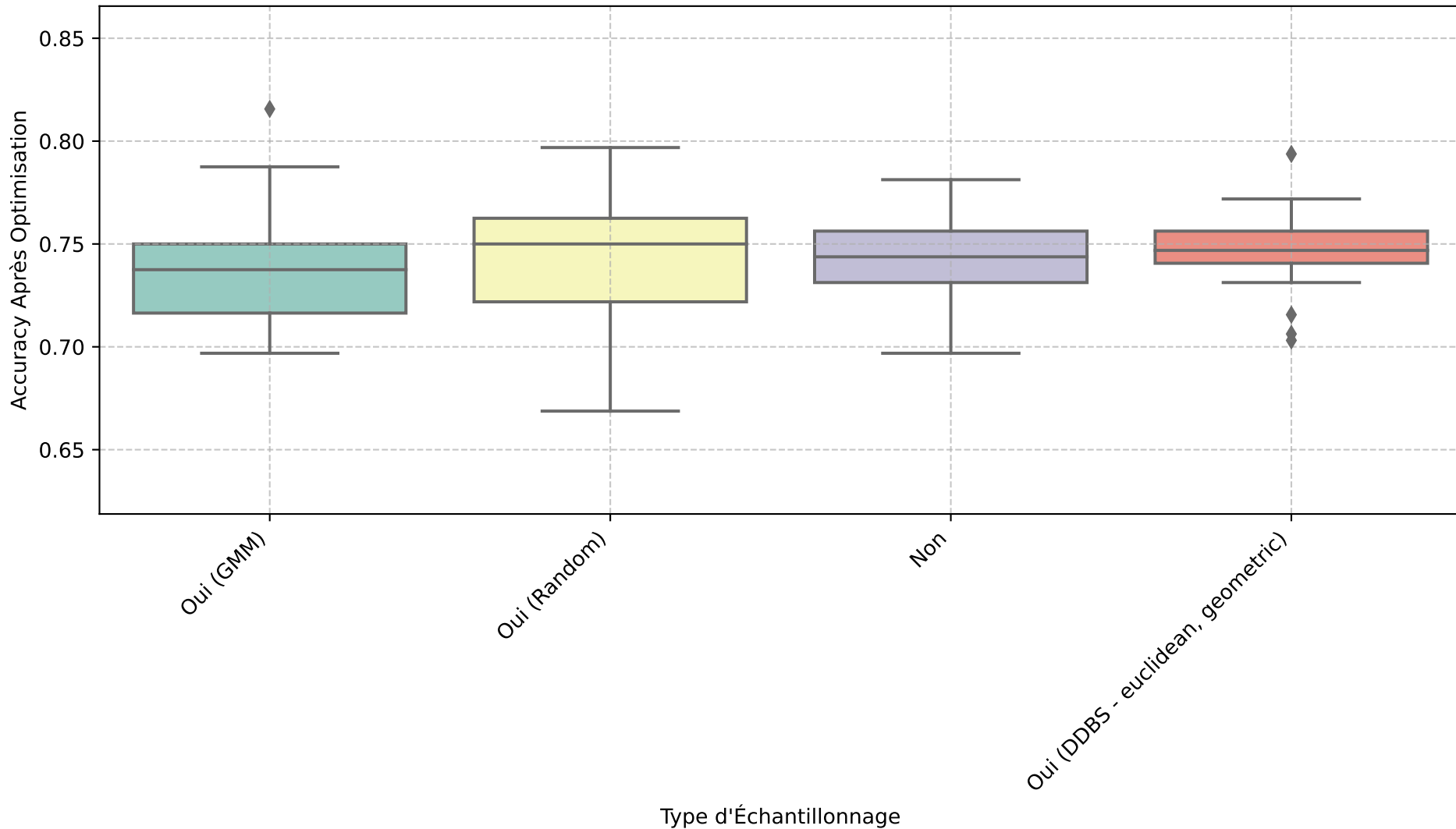
Boxplot - resultats_SVM_preprocessed_winequality_dataset
