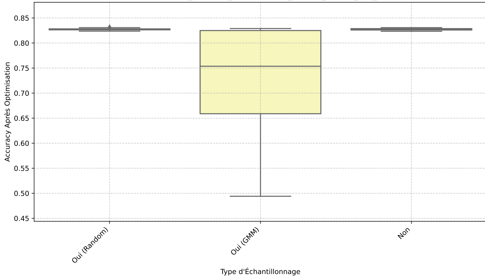
Boxplot - resultats_XGBoost_preprocessed_thyroid_cancer_risk_dataset
