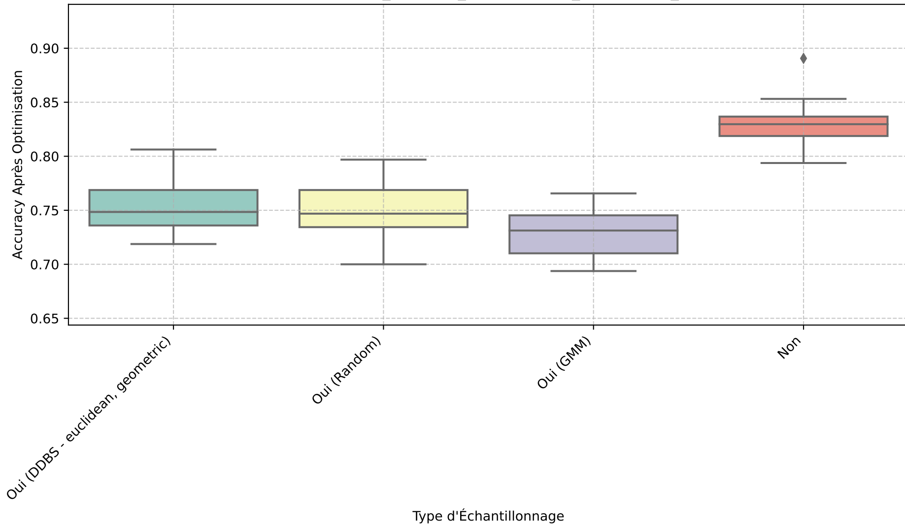
Boxplot - resultats_XGBoost_preprocessed_winequality_dataset
