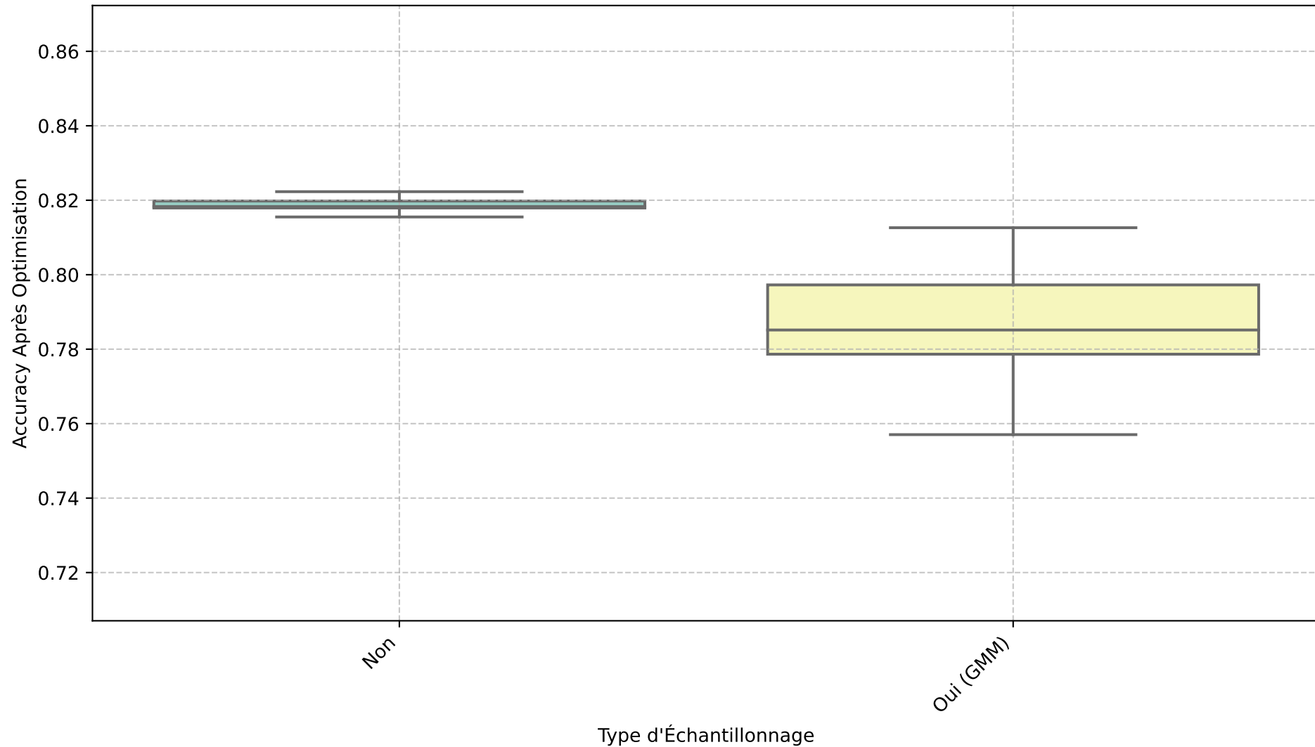
Boxplot - resultats_SVM_preprocessed_thyroid_cancer_risk_dataset
