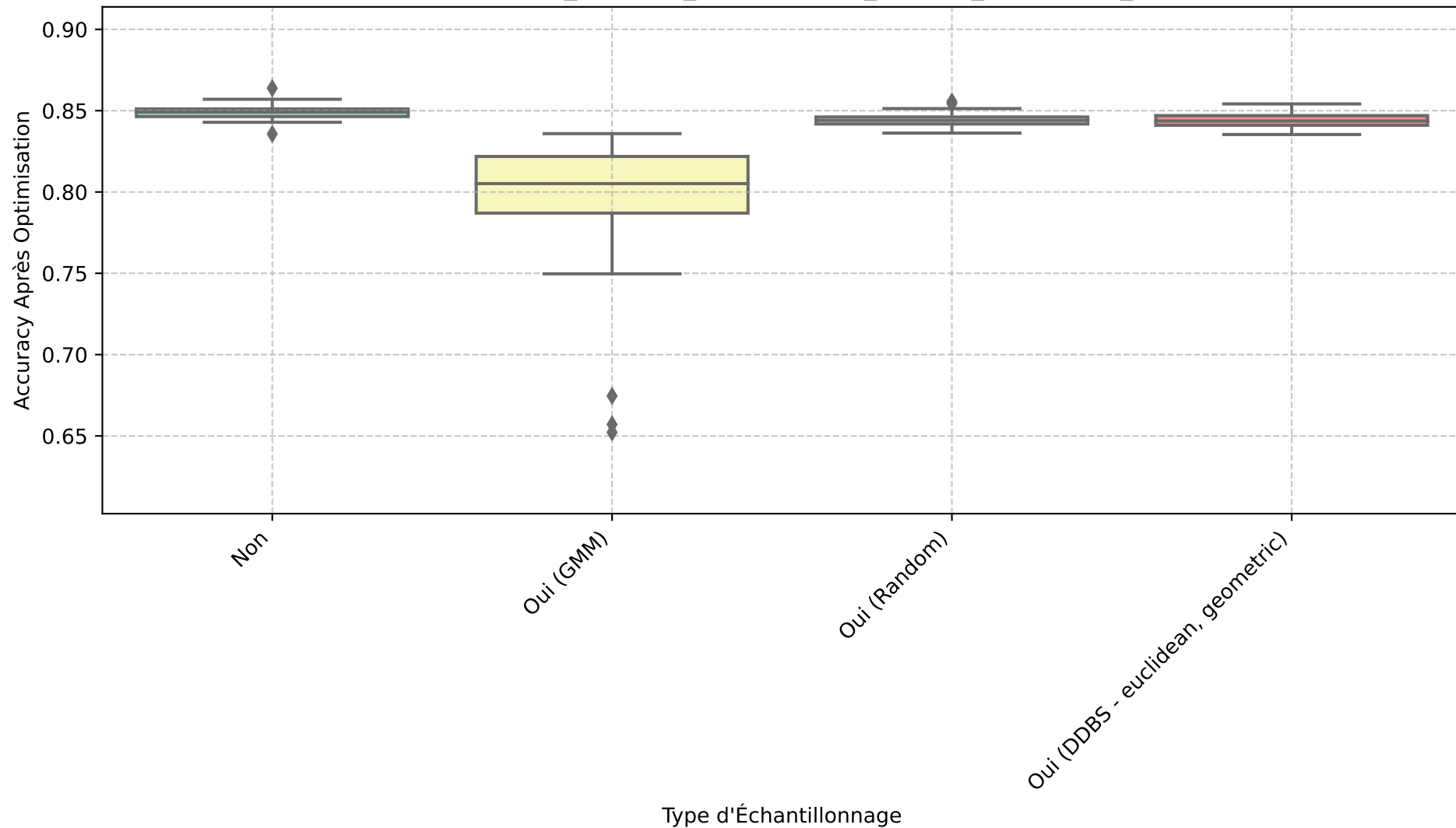
Boxplot - resultats_XGBoost_preprocessed_student_depression_dataset
