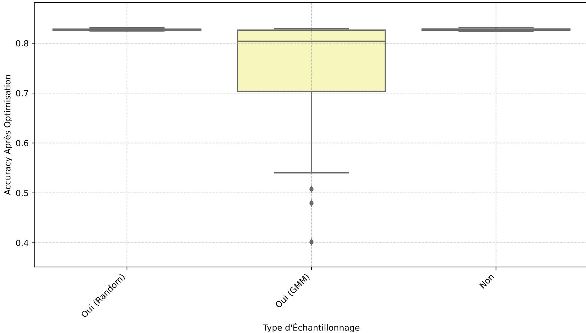
Boxplot - resultats_Random Forest_preprocessed_thyroid_cancer_risk_dataset
