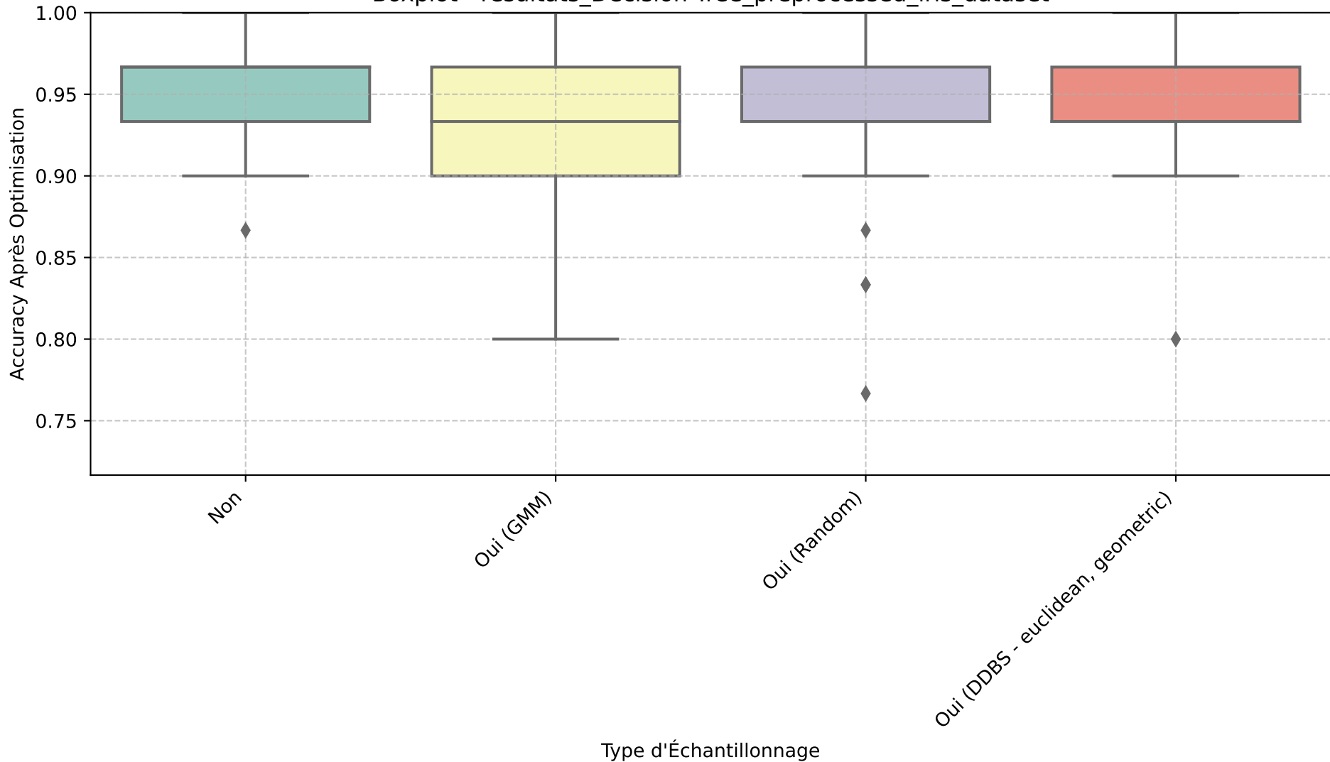
Boxplot - resultats_Decision Tree_preprocessed_iris_dataset
