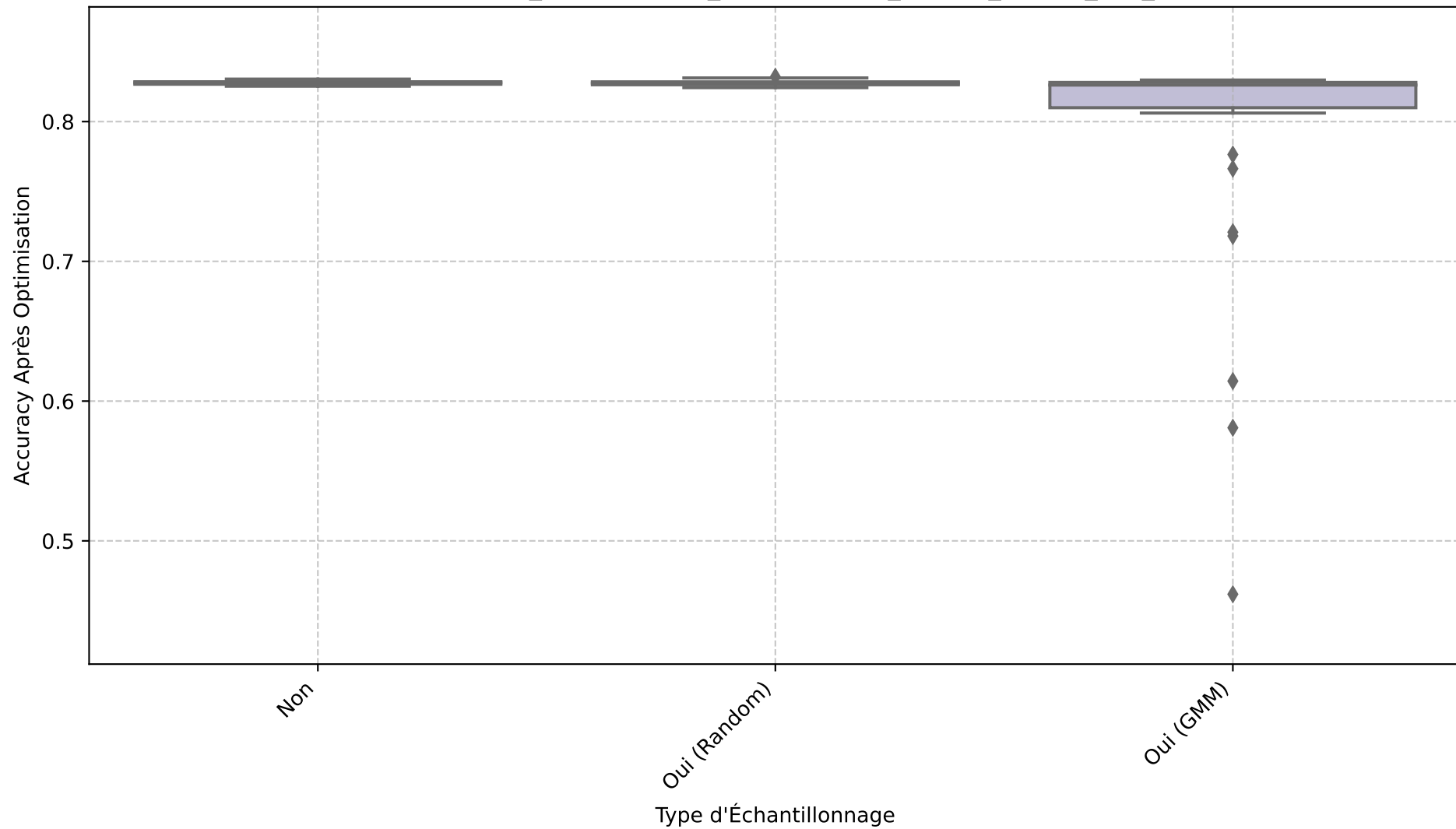
Boxplot - resultats_Decision Tree_preprocessed_thyroid_cancer_risk_dataset
