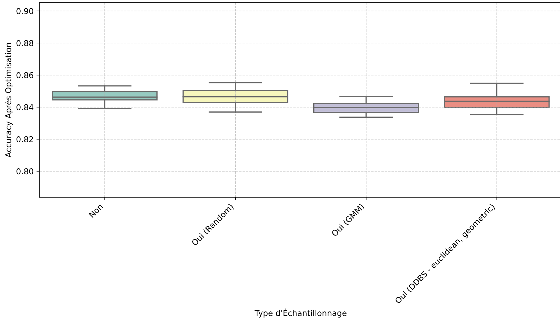
Boxplot - resultats_SVM_preprocessed_student_depression_dataset
