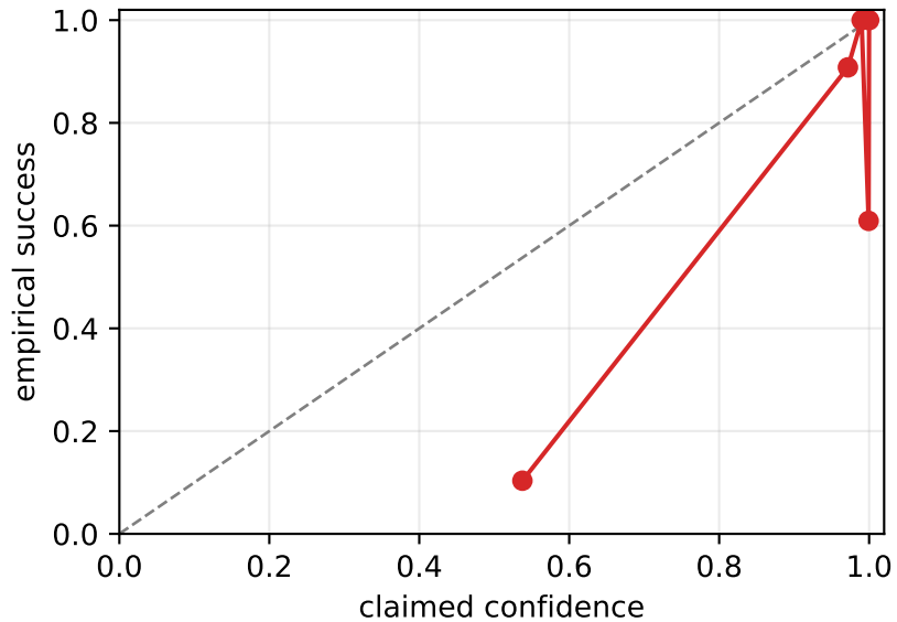
Reliability (equal-mass bins), ECE=0.180
