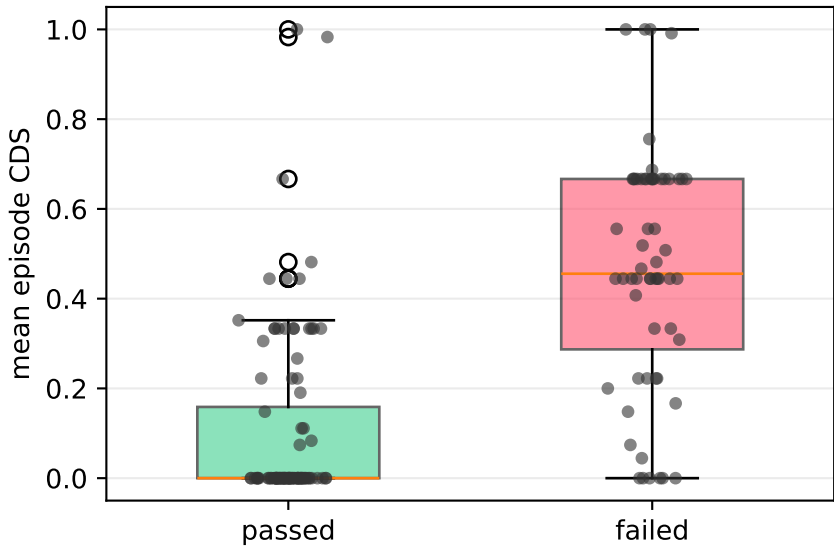
Context divergence vs outcome (multi-agent)
