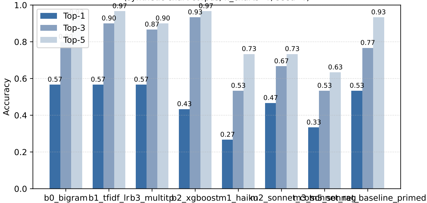
Top-K next-procedure accuracy on 240 examples (synthetic chart corpus, n_charts=?, seed=?)
