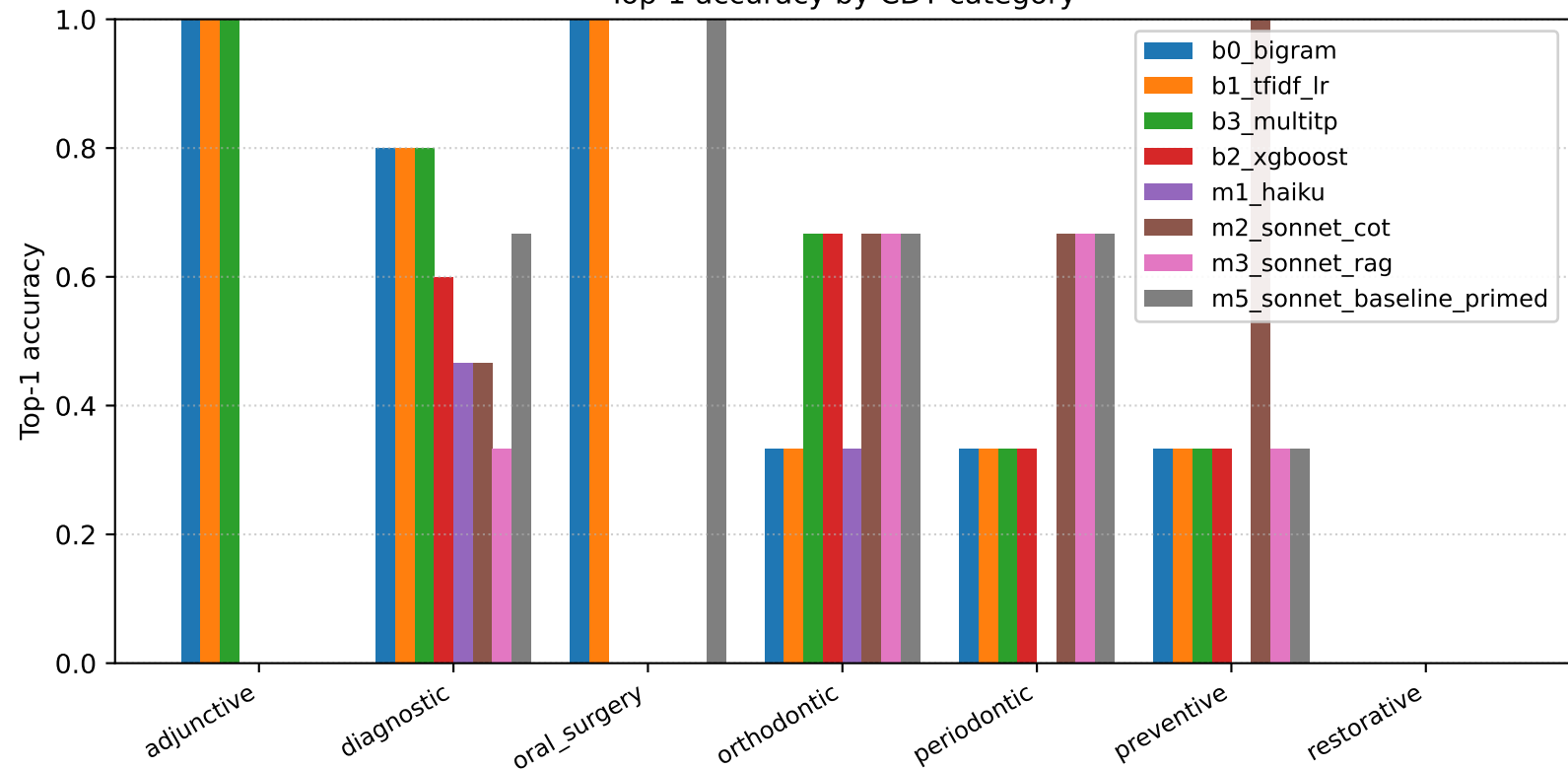
Top-1 accuracy by CDT category
