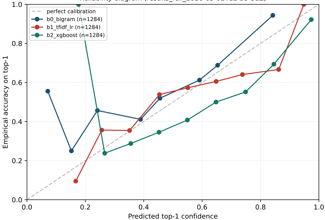
Reliability diagram (results_full_2026-05-02T12-35-51Z)
