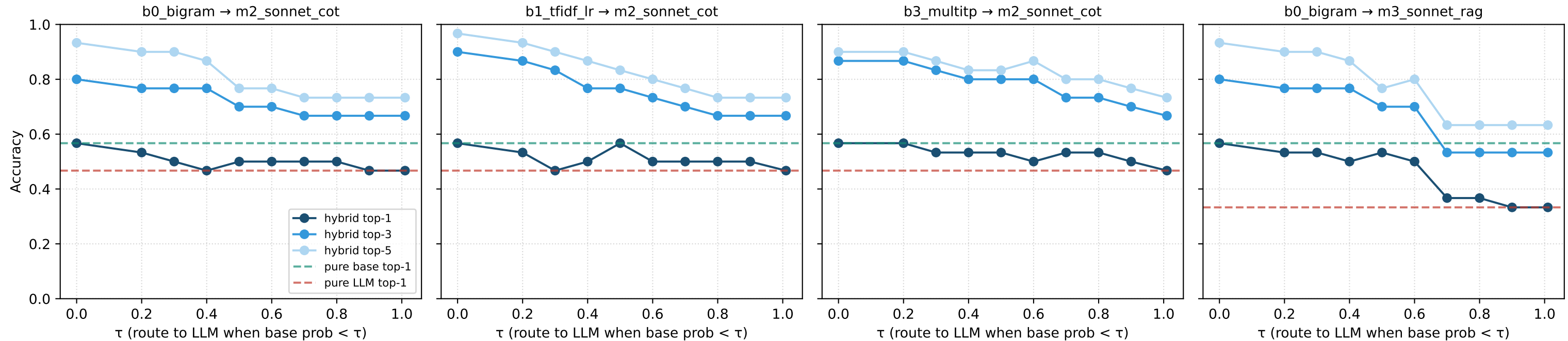
Confidence-routed hybrid: classical baseline (gate) \rightarrow LLM (when base top-1 < \tau ). Synthetic n=30.
