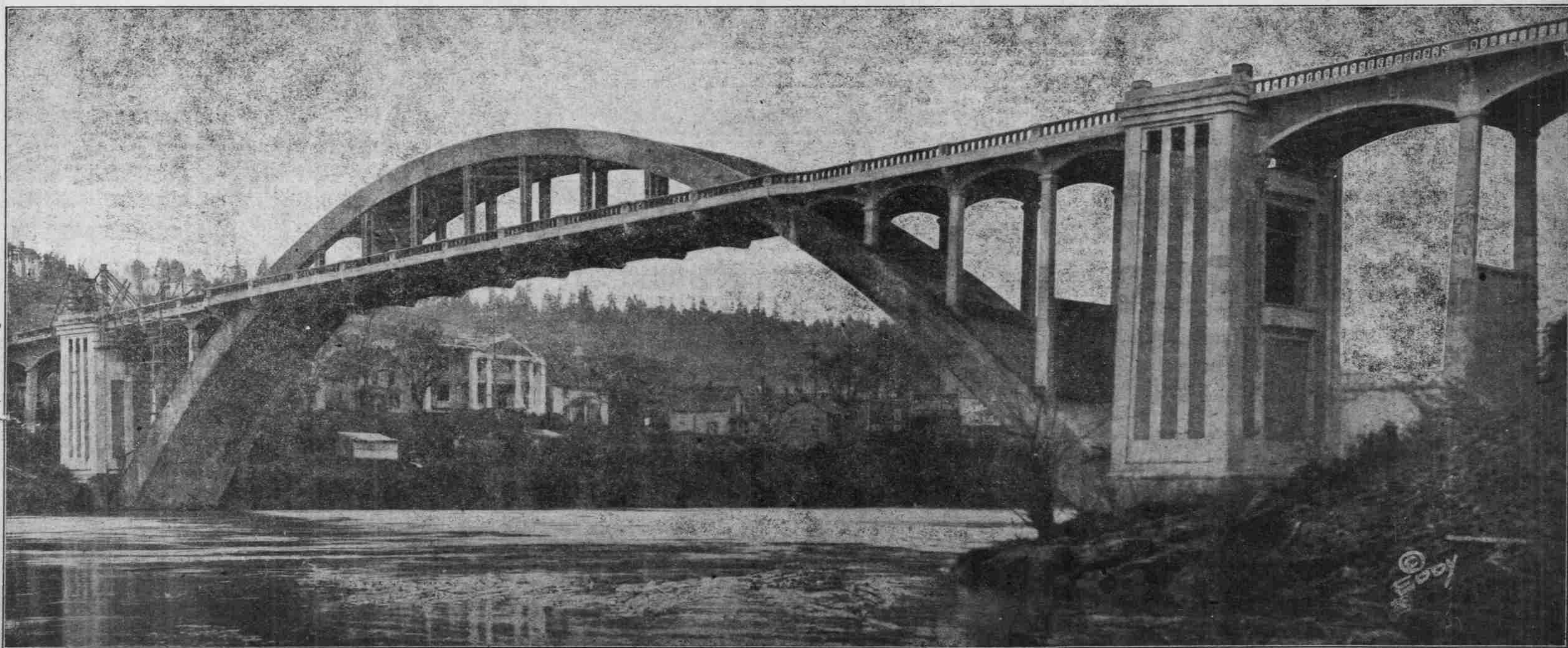
The new arch, upon the Pacific Highway between Oregon City and West Linn, was designed by the state highway commission bridge engineer C. B. McCullough, and its construction supervised by Engineers R. A. Furrow and C. P. Richards. It was built by A. Guthrie and Company, Inc., of Portland. Its total length is 850 feet. Deck above low water at mid-span, 77 ft. Main span: steel rib arch with gunite encasement; 350 ft. span, 100 ft. high. Approaches: reinforced concrete beam and slab spans, 35 ft. centers. Height of West Linn pier, rock foundation to road level, 98 ft. Road: slope, 5 per cent; width, 13 1-2 ft. Two sidewalks, 4 3-4 ft. each. Weight of steel in arch, 480 tons; reinforcing steel, 150 tons. Volume, concrete, 4600 cu. yds. Volume, gunite, 250 cu. yds. Construction started July 29, 1921. Completed December, 1922. Cost $275,000.00.
