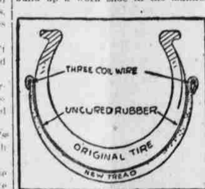
How New Tread is Attached.
