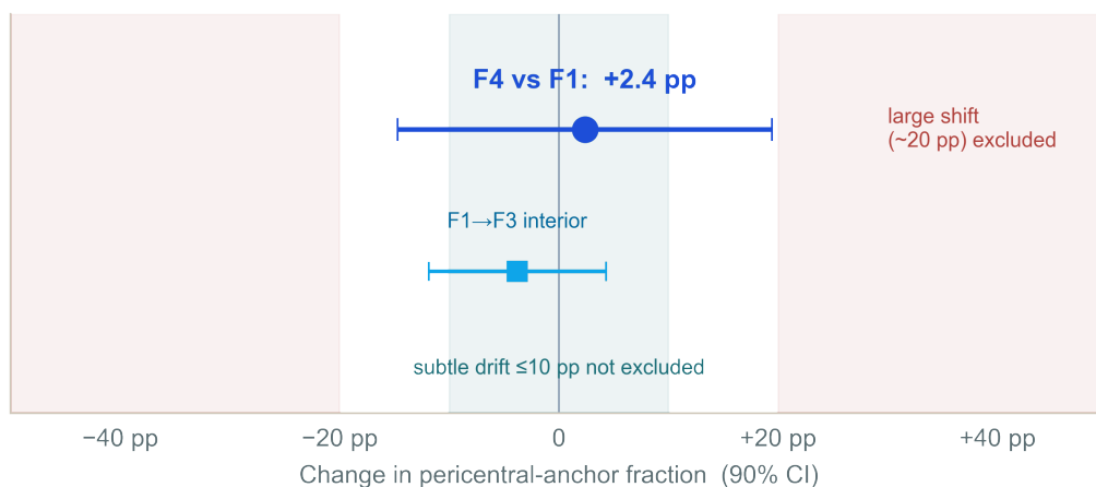
Figure 4: Equivalence bound on the F4-vs-F1 pericentral-anchor change: a large shift is excluded, a subtle one is not.
