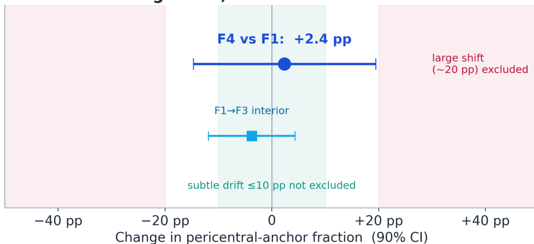
Figure 4: Equivalence bound. TOST on the donor-level pericentral-anchor fraction across biopsy F1→F4: the 90% CI excludes a ~20-point shift but not a ≤10-point drift — a quantified bound on “preserved,” honest about the limited power at n=4 .
