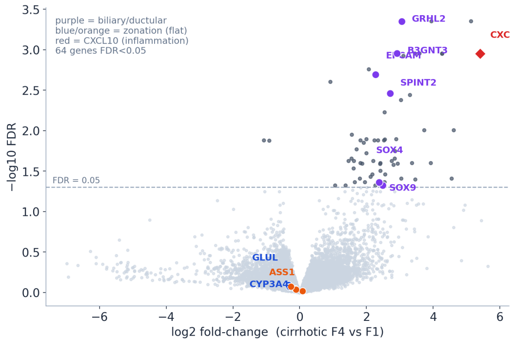
Figure 6: Genome-wide pseudobulk DGE (F4-vs-F1) volcano. Zonation genes sit at the origin (flat; GLUL FDR 0.80). The significant hits are a biliary/ductular marker set (EPCAM, GRHL2, SPINT2, SOX4, SOX9, B3GNT3) plus CXCL10.
