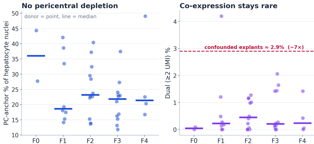
Figure 2: Matched-biopsy anchor classification. Pericentral-anchor and strict ( \geq 2 -UMI) dual co-expression fractions across needle-biopsy fibrosis stages. The pericentral fraction is flat/non-monotone; the dual fraction is near-zero and collapses from the permissive 1-UMI value, indicating the 1-UMI co-expression was ambient. Full four-panel breakdown (PC / dual / null / PP:PC) in Figure 3.
