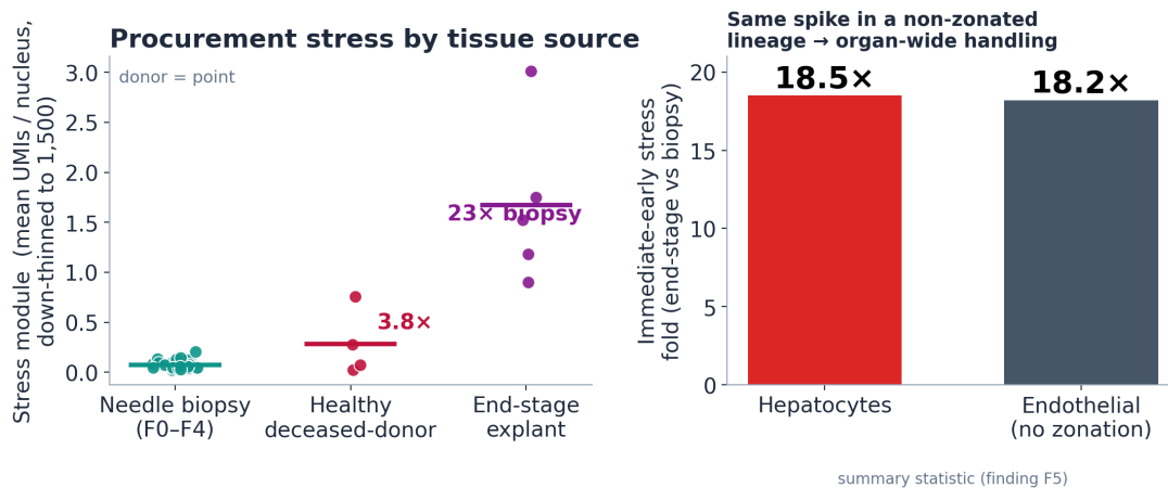
Figure 1: Procurement stress by tissue source and across lineages. Depth-matched stress-module (immediate-early + heat-shock) UMIs per nucleus are uniformly low across needle biopsies and rise sharply in the deceased-donor organ-cube endpoints (healthy, end-stage). The explant-vs-biopsy fold is essentially identical in hepatocytes and in endothelial cells, which carry no zonation program — establishing the signal as organ-wide acute handling, not a hepatocyte disease program.
