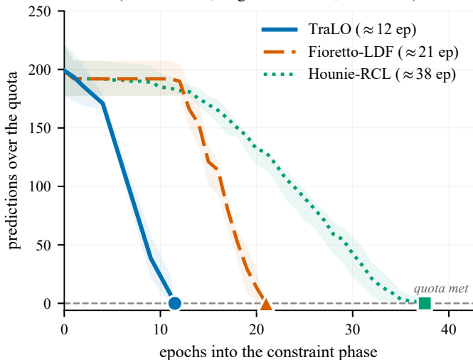
Reaching the quota during training (DermMNIST, RegNetY-400MF, L = G = 30 )
