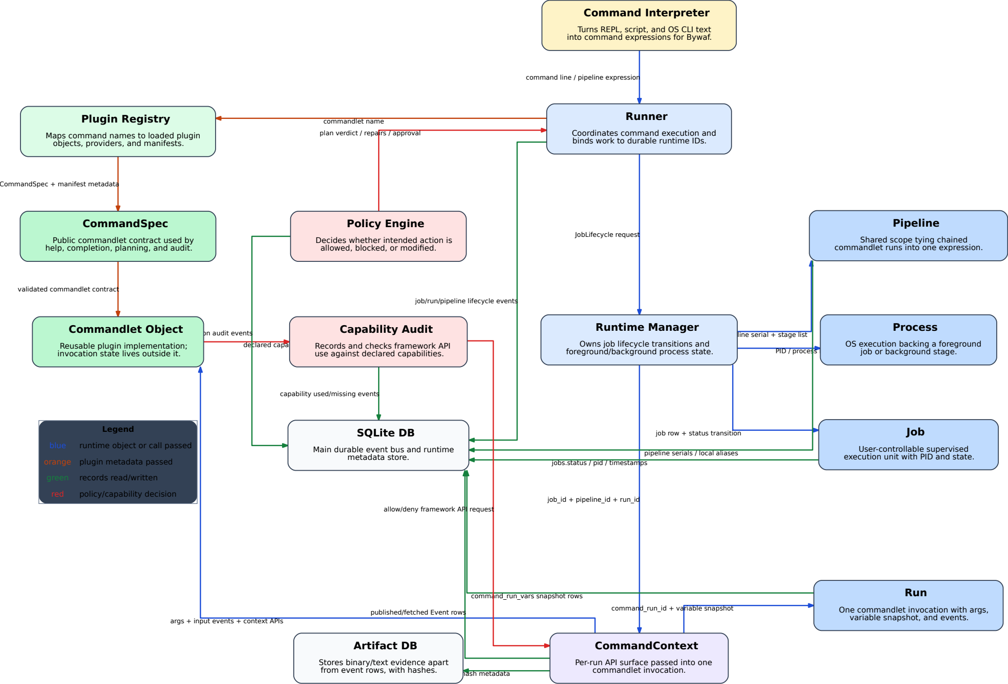
Bywaf Runtime Block Diagram Runtime constructs and framework objects. Data movement is shown separately in SYSTEM_DATAFLOW_DIAGRAM.pdf.
