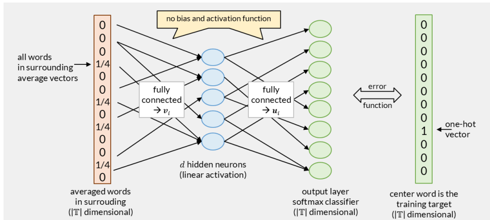
Figure 5.13: CBOW network architecture: context word vectors are averaged into the input, then the same hidden-layer and softmax structure as Skip-Gram predicts the center word.
