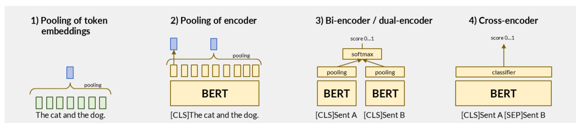
Figure 5.19: Four architectures for sentence similarity, progressing from simple to powerful: (1) pooling static word embeddings, (2) pooling BERT token outputs, (3) bi-encoder with independently encoded sentences compared via learned similarity, (4) cross-encoder that jointly processes both sentences for maximum accuracy.
