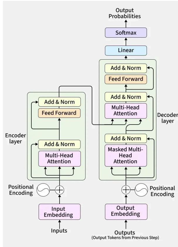
Figure 5.17: The transformer architecture (Vaswani et al., 2017). Left: the encoder processes input bidirectionally through stacked layers of multi-head self-attention and feed-forward networks. Right: the decoder generates output auto-regressively with masked attention. For text embeddings, only the encoder is used.
