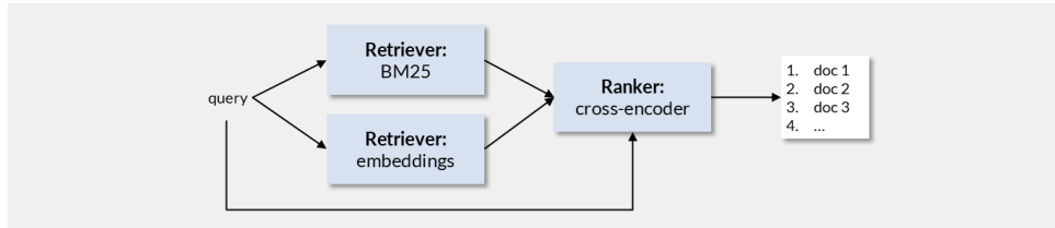
Figure 5.23: Pipeline D: BM25 and dense retrieval run in parallel on the same query. Their candidate lists are fused, then a cross-encoder reranks the merged results.
