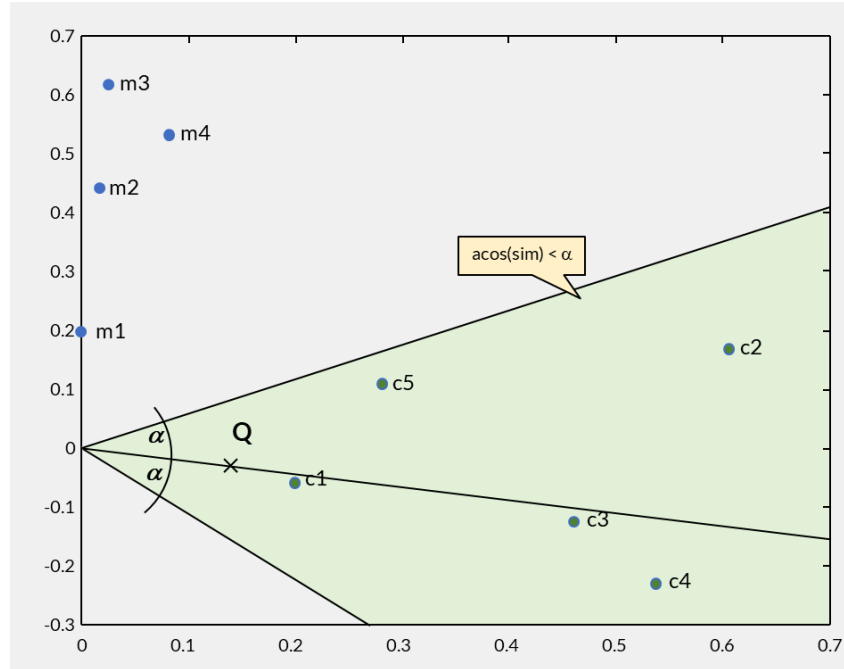
Figure 5.8: Documents and query in the 2D latent space. Topic 1 (horizontal) aligns with the interface documents c1-c5, while topic 2 (vertical) aligns with the graph documents m1-m4. The shaded angular cone shows all documents within angle \alpha of the query vector.
