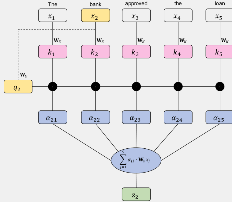
Figure 5.15: Self-attention computing z_2 for “bank”. The query q_2 is compared against all keys to produce attention weights. “Approved” (0.52) and “loan” (0.36) dominate, so z_2 is primarily a blend of their values, making “bank” context-aware as a financial institution.
