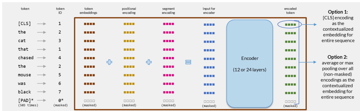
Figure 5.18: BERT input construction for "the cat that chased the mouse was black". Token embeddings, positional encodings, and segment encodings are summed to produce the encoder input. After 12/24 layers, each token has a contextualized output vector. Option 1: use the [CLS] encoding as the sequence embedding. Option 2: pool over all non-masked token encodings.
