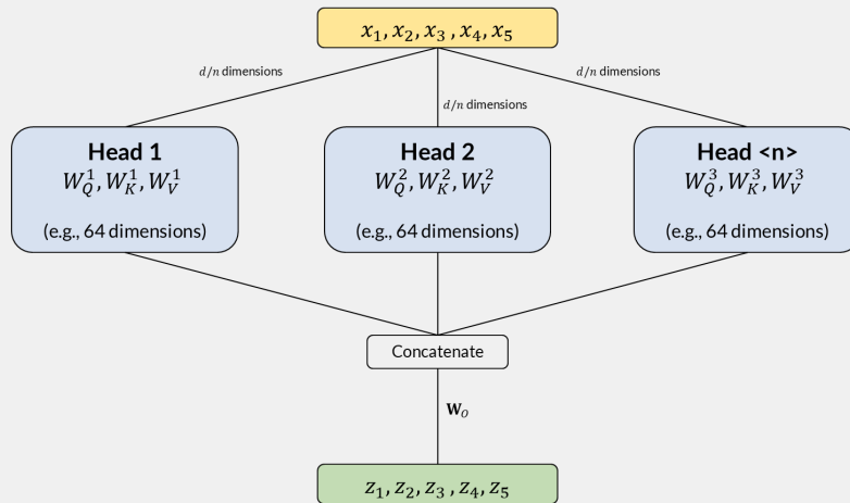
Figure 5.16: Multi-head attention: h parallel heads each run self-attention in d/h dimensions with independent projections. Concatenating all heads recovers the full d -dimensional output.
