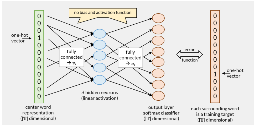
Figure 5.11: Skip-Gram as a single-hidden-layer neural network. The first weight matrix stores center word vectors \mathbf{v}_i , the second stores context word vectors \mathbf{u}_i .
