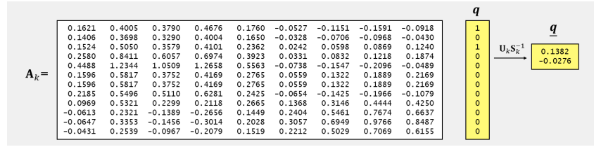
Figure 5.7: Folding-in of the query “human computer interaction”: the sparse 12-dimensional term vector q is projected to a 2-dimensional latent representation via U_k S_k^{-1} .
