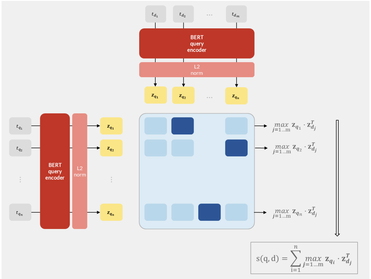
Figure 5.20: ColBERT architecture: query and document are encoded independently (allowing document pre-computation), but scoring uses token-level MaxSim interaction rather than a single-vector dot product.
