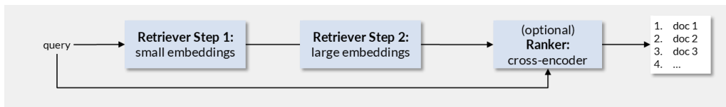
Figure 5.24: Multi-stage retrieval with Matryoshka embeddings: fast initial retrieval using small (truncated) embeddings narrows candidates, then full-dimension embeddings rerank with higher precision. A single model serves both stages.
