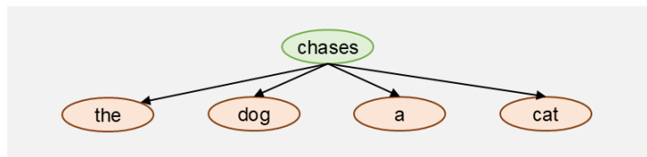
Figure 5.10: Skip-Gram context for “the dog chases a cat”: the center word “chases” independently predicts each surrounding word within the window.
