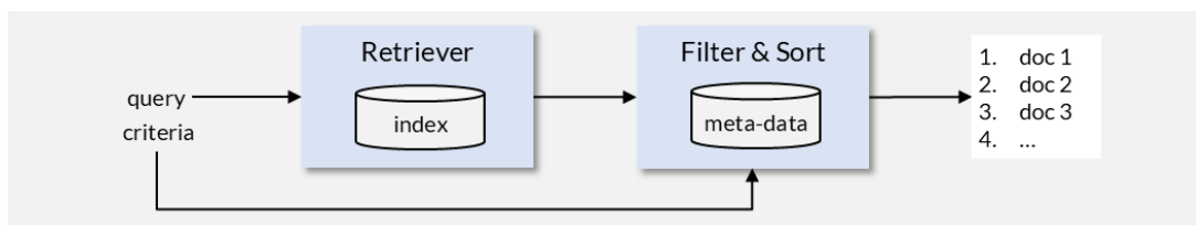
Figure 1.3: Retriever with faceted filtering: candidates are filtered and sorted by metadata.
