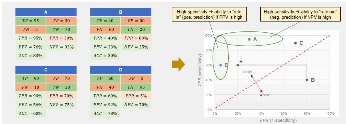
Figure 2.12: Four classifiers (A-D) mapped from their confusion matrices to ROC space. The upper-left region represents high sensitivity with low false-positive rate; the diagonal represents random performance.
