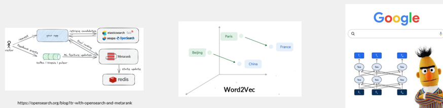
Figure 0.7: Neural ranking in the 2010s: a Learning-to-Rank pipeline (left), an embedding space (center), and contextual models like BERT (right).
