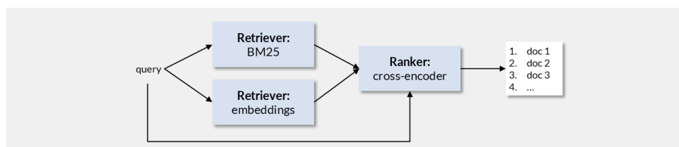
Figure 5.21: Pipeline D: BM25 and dense retrieval run in parallel on the same query. Their candidate lists are fused, then a cross-encoder reranks the merged results.
