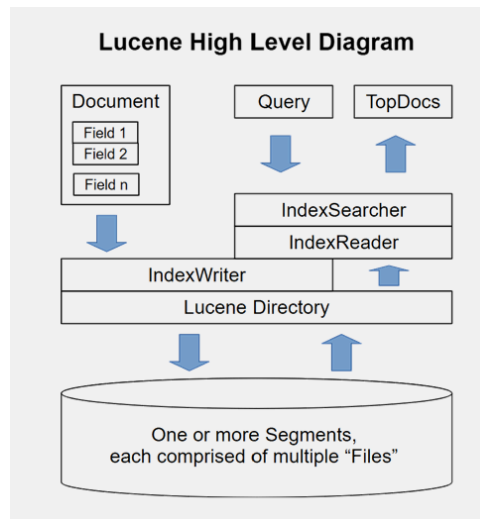
Figure 4.4: Lucene's architecture: the write path (Document, IndexWriter, Directory, Segments) and the read path (Query, IndexSearcher, IndexReader, Directory, Segments, TopDocs) meet at the Directory storage abstraction.
