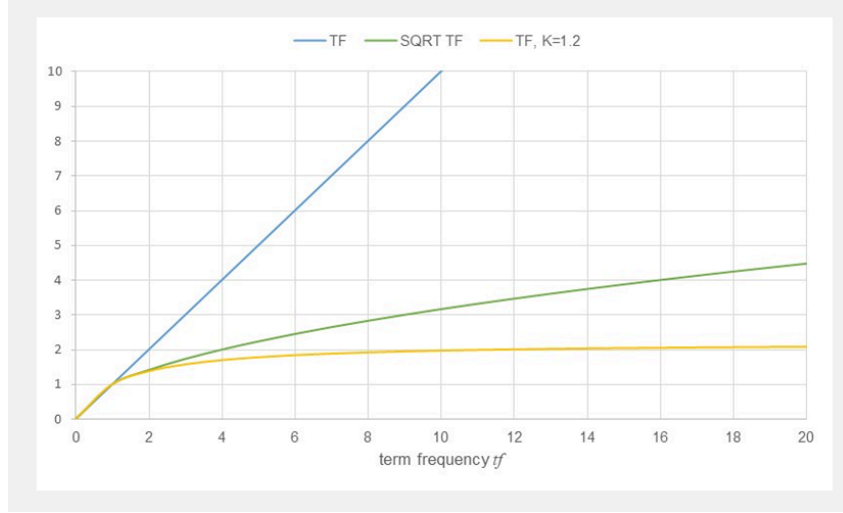
Figure 1.16: Linear, square-root, and BM25-saturated term-frequency weighting.
