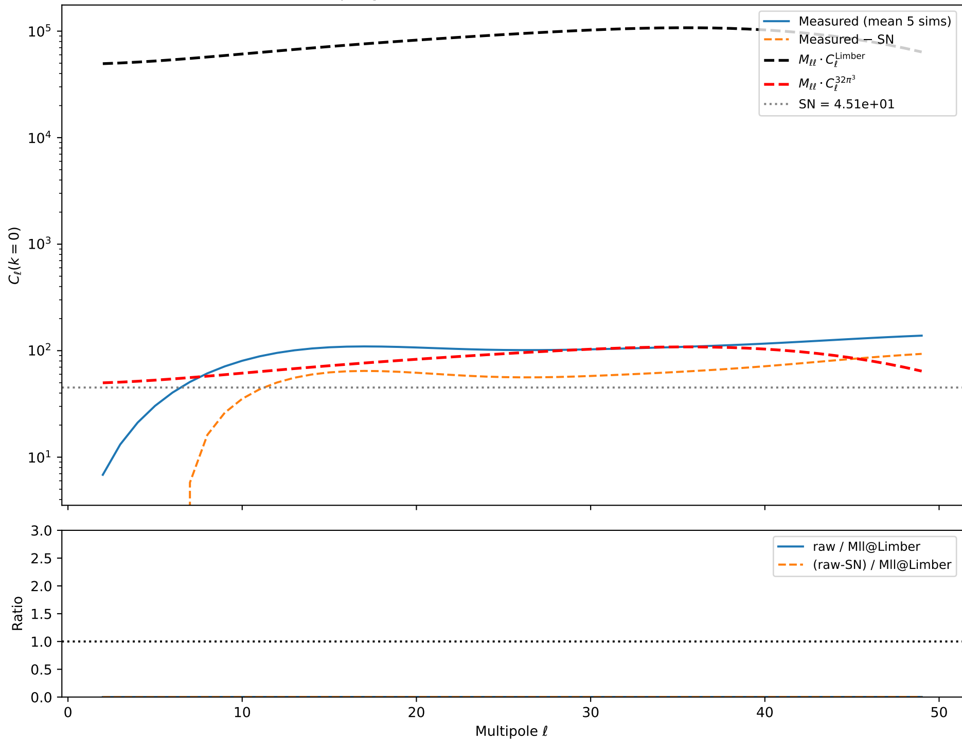
Full-sampling test: N=64, Nskew=N 2 =4096, NI=50, 5 sims
