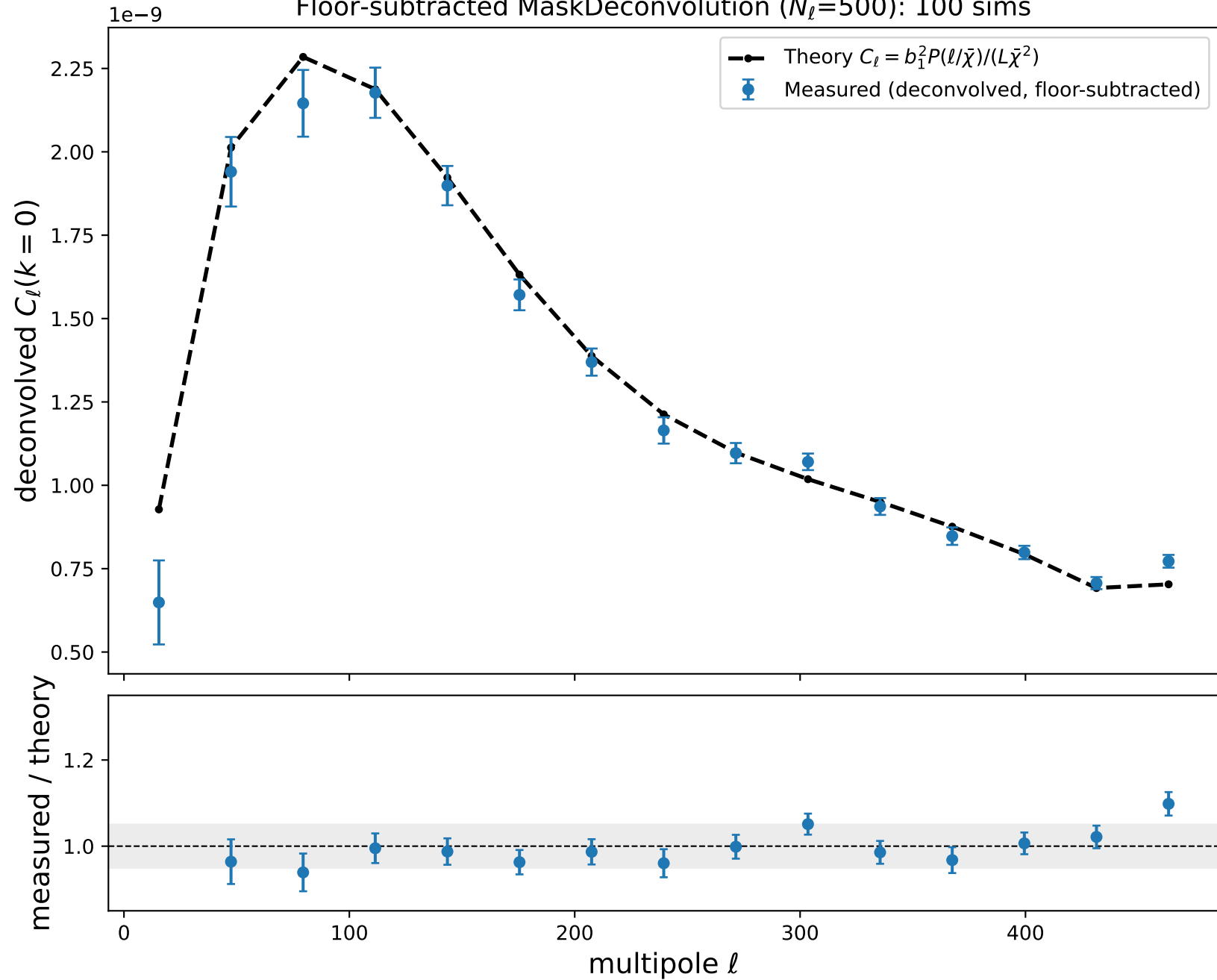
Floor-subtracted MaskDeconvolution ( N_\ell=500 ): 100 sims
